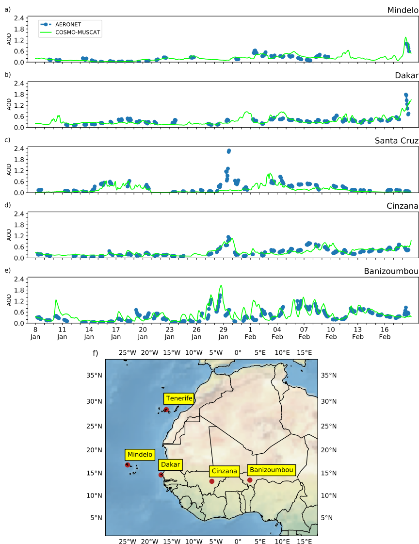
Figure 3. Dust AOT at 550 nm calculated from COSMO-MUSCAT dust concentration fields (green) and AOT at 550 nm from AERONET sun-photometer measurements (blue) for January-February 2022 where each x-axis tick represents the 12:00 UTC for each day in the range of 8 January to 18 February 2022. Five different stations across the Sahara Desert and downwind locations are shown. a) Mindelo (16.878°N, 24.995°W; Cape Verde; Level2.0), b) Dakar Belair (14.702°N, 17.426°W; Senegal; Level2.0), c) Santa Cruz Tenerife (28.473°N, 16.247°W; Spain; Level2.0), d) IER Cinzana (13.278°N, 5.934°W; Mali; Level1.5), e) Banizoumbou (13.547°N, 2.665°E; Niger; Level2.0), (f) AERONET stations geographic locations and names used in this comparison.
