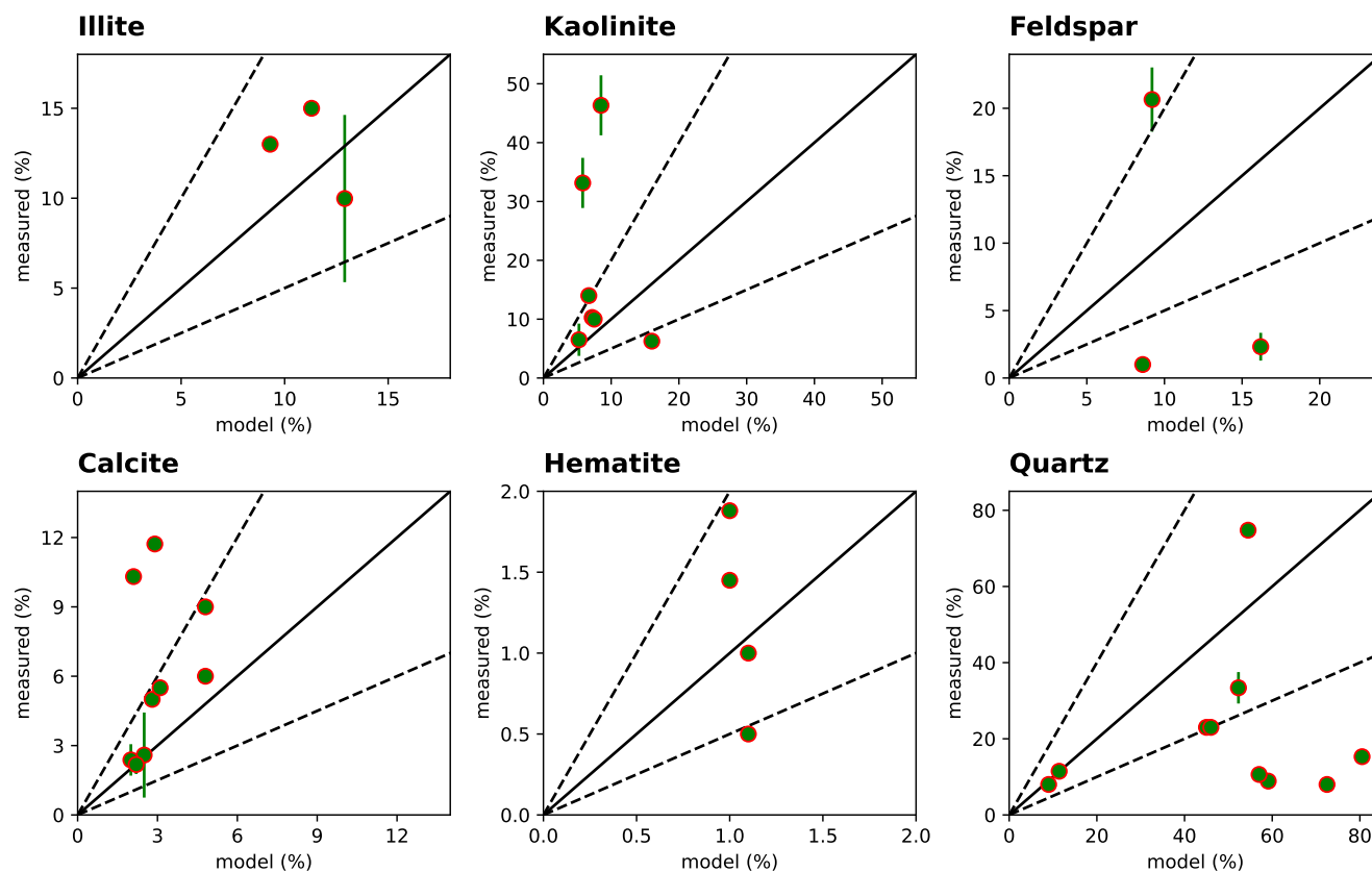
Figure 5. Scatterplot of minerals mass percentages of illite, kaolinite, feldspar, calcite, hematite and quartz simulated by COSMO-MUSCAT vs. measurements. All measurements were done on aerosols bulk size range. The dashed lines represent the ratios of 2:1 and 1:2 between the simulated and observed mineral percentages. The error bars are present when reported in the measurements.
