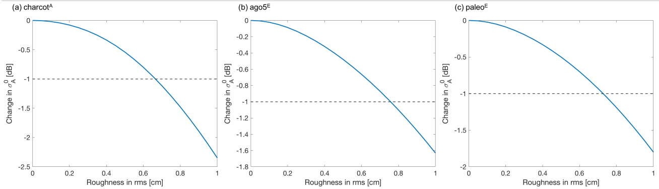
Figure A2. Change in \sigma_A^0 when the surface roughness (expressed as root mean square heights; rms) is changed. The dashed line indicates when the sensitivity exceeds 1 dB.
