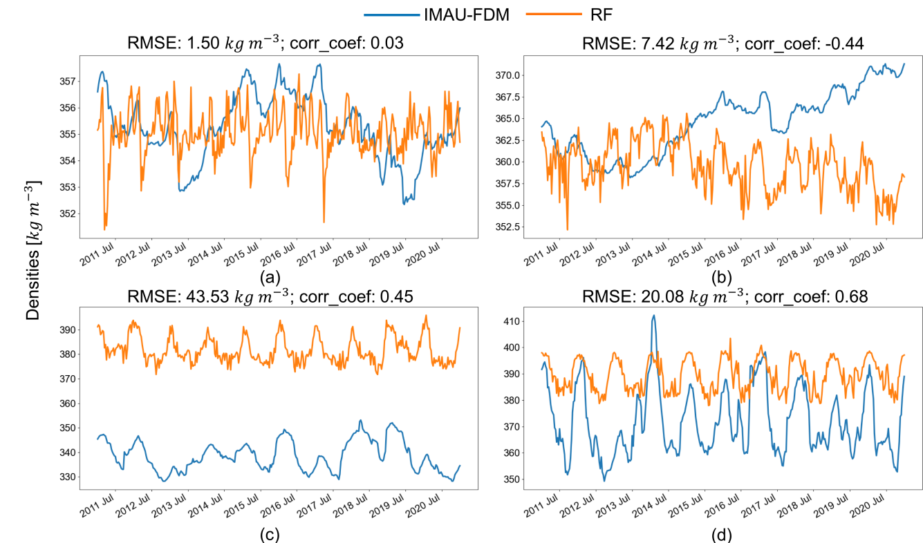
Figure 8. Comparison between time series of IMAU-FDM densities (in blue) and RF densities (in orange) at 4 representative sample points and Dome C. Panels (a)–(d) correspond to A–D labelled in Fig.4. The RMSE and correlation coefficient (corr_coef) between the IMAU-FDM densities and the RF densities are shown above each figure.
