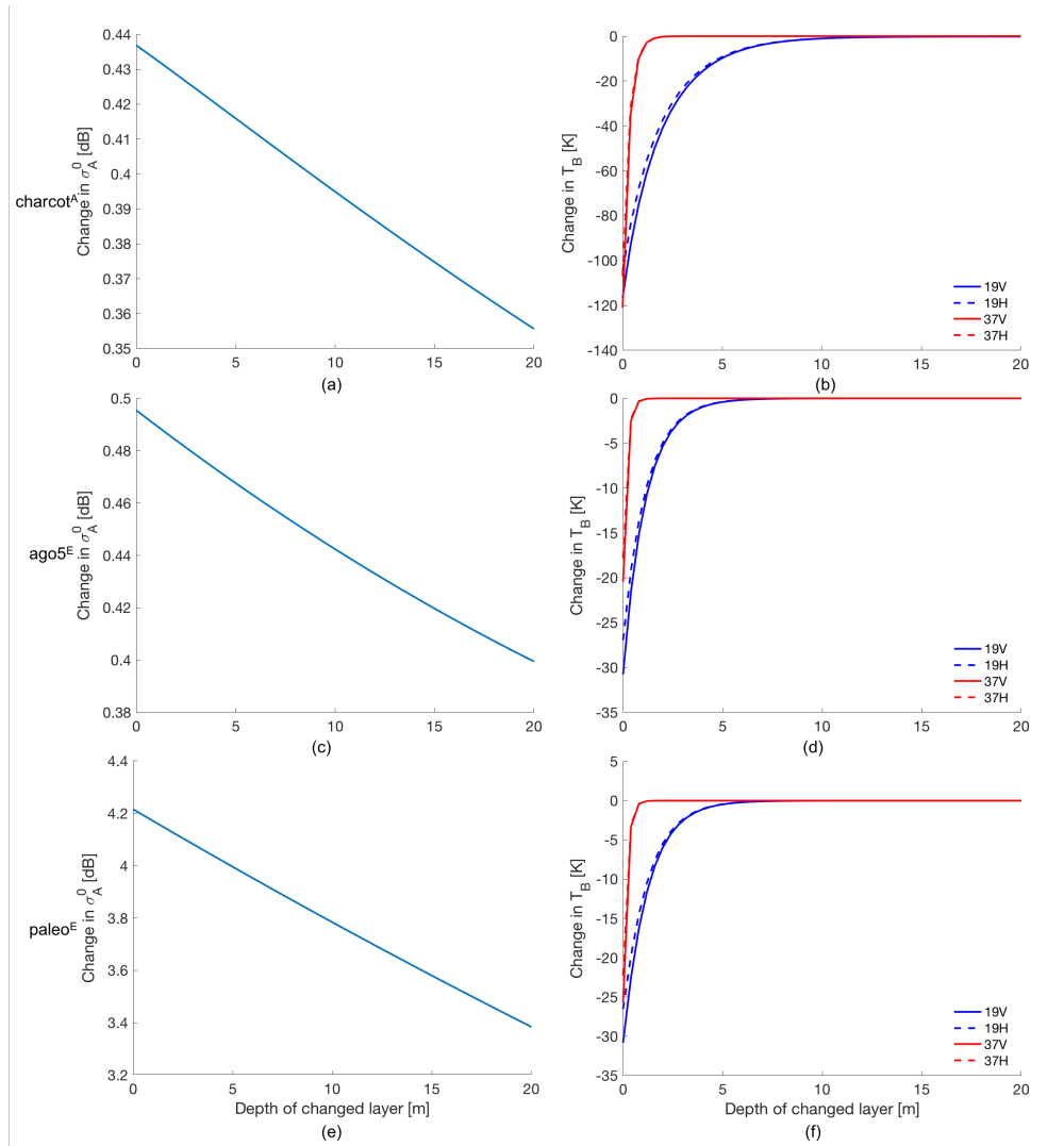
Figure A1. Change in \sigma_A^0 and T_B as a function of the depth of the layer whose density and grain size are changed.
