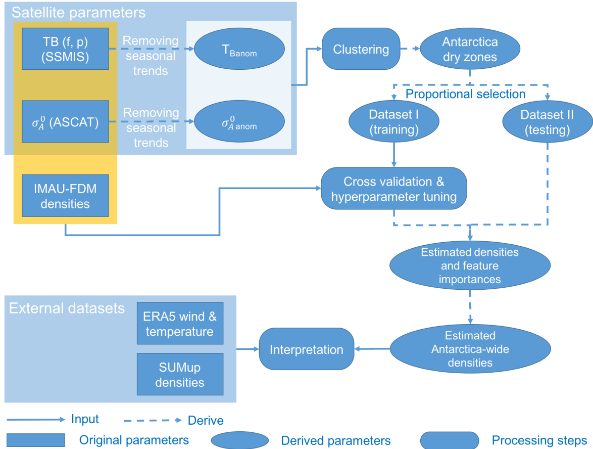
Figure 1. Overview flowchart of the data and method used in this study. The clustering process uses T_{Banom} and \sigma_{A^0}^{anom} as input to derive dry snow zones over the Antarctic ice sheet. Then, pixels clustered as dry snow are included to estimate firm density with the RF regressor. Parameters used as features of the RF regressor are further elaborated in Sect. 3.3. Among the derived parameters, Antarctica dry zones, Dataset I and Dataset II are selected proportionally based on the number of pixels per cluster.
