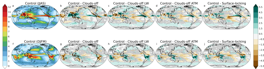
Figure 12. As in Figure 2, but for precipitation. All values have units of mm day -1 .
