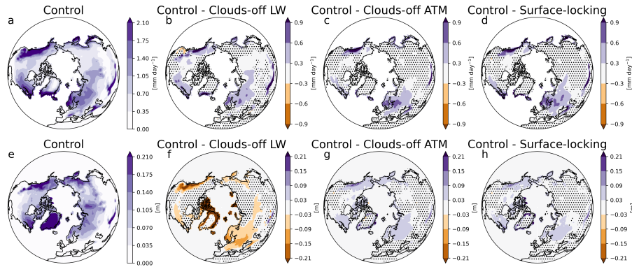
Figure 5. (Top row) Arctic snowfall for the (left a,e) Control, and the impact of clouds relative to the (middle b,f) Clouds-off LW and (right c,g) Clouds-off ATM, and (d,h) Surface-locking experiments. (Bottom row) the same, but for the snow water equivalent (SWE). Stippling denotes locations where differences are not statistically significant at the 95th percentile. Snowfall is given in \text{mm day}^{-1} and SWE is given in m.
