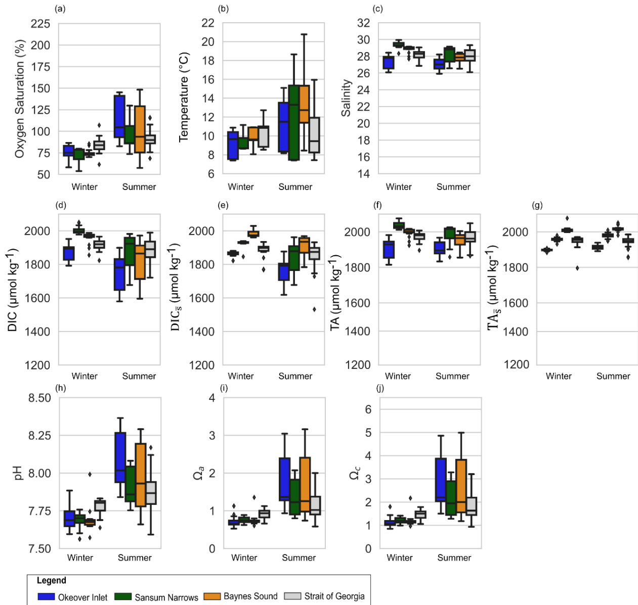
275 Figure 3 Observed variability in the 5-20 m layer at shellfish grow sites and in adjacent waters in a) dissolved oxygen (% saturation), b) 280 temperature c) salinity, d) DIC, e) salinity normalized DIC ( DIC_s ), f) TA, g) salinity normalized TA ( TA_s ), h) pH, i) \Omega_a and j) \Omega_c at nearshore locations shown in Fig. 1: Okeover (dark blue), Sansum Narrows (dark green), Baynes Sound (orange) and ship collected data from the SOG (grey). Data have been split into a summer season capturing the phytoplankton bloom (April-September) and winter season (October-March). Note that Y-axes are the same as Fig. 2 for comparison, and locations by season are shown in the same order right to left in each panel. The mean annual salinity (Table A3) at each location was used to normalize DIC and TA to show the impact of dilution. Similar to the surface layer, there is inter-seasonal variability at all locations and greater variability and range of conditions during the
