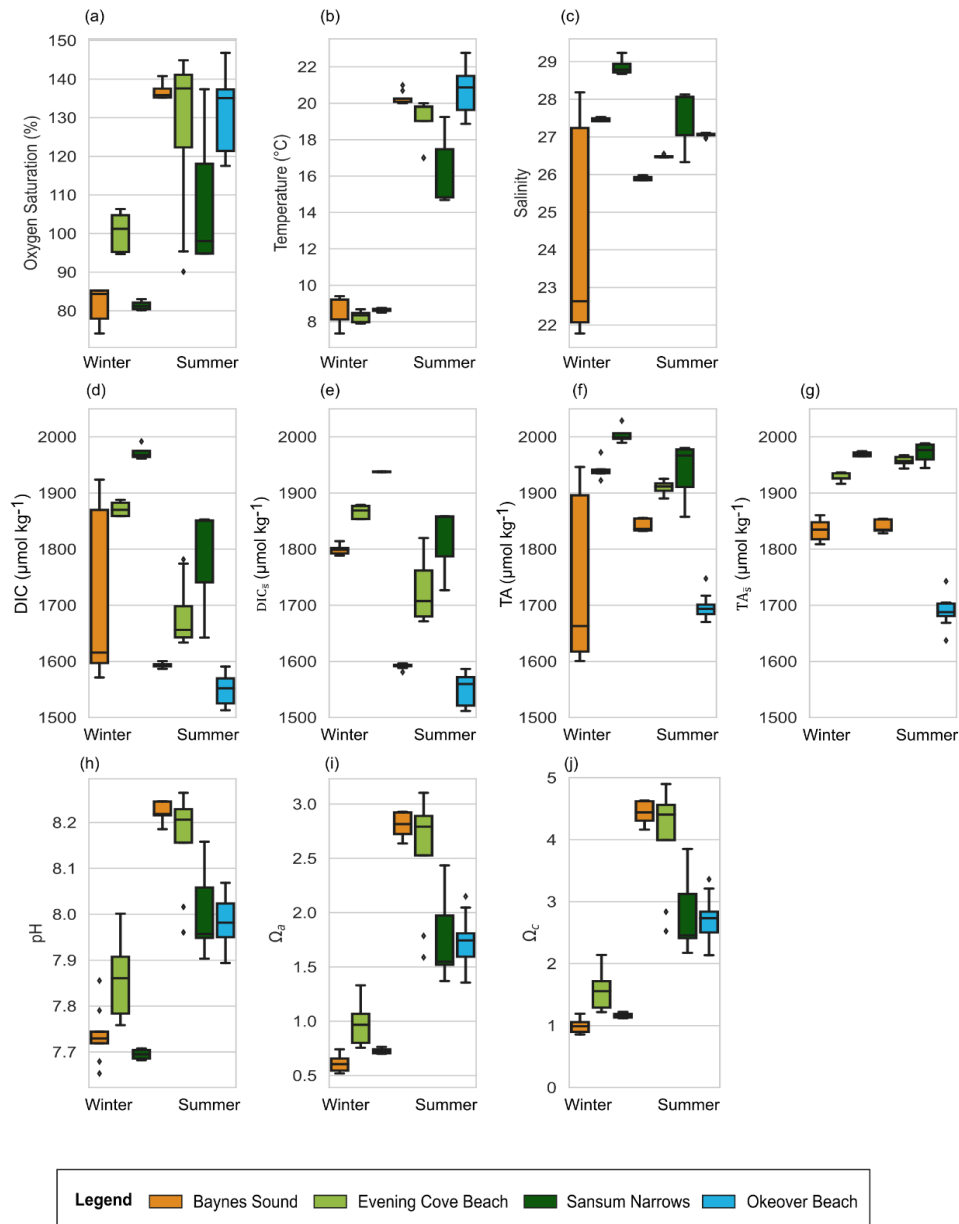
285 Figure 4 Variability during one sampling day (Table 2) at Baynes Sound (orange), Evening Cove beach (light green) and Sansum Narrows (dark green) for both summer and winter, and Okeover beach (light blue) in summer only, in a) dissolved oxygen (% saturation), b) temperature c) salinity, d) DIC, e) salinity normalized DIC ( \text{DIC}_s ), f) TA, g) salinity normalized TA ( \text{TA}_s ), h) pH, i) \Omega_a and j) \Omega_c , in winter (left) and summer (right). The mean annual salinity (Table A3) at each location was used to normalize DIC and TA (e,h) to
