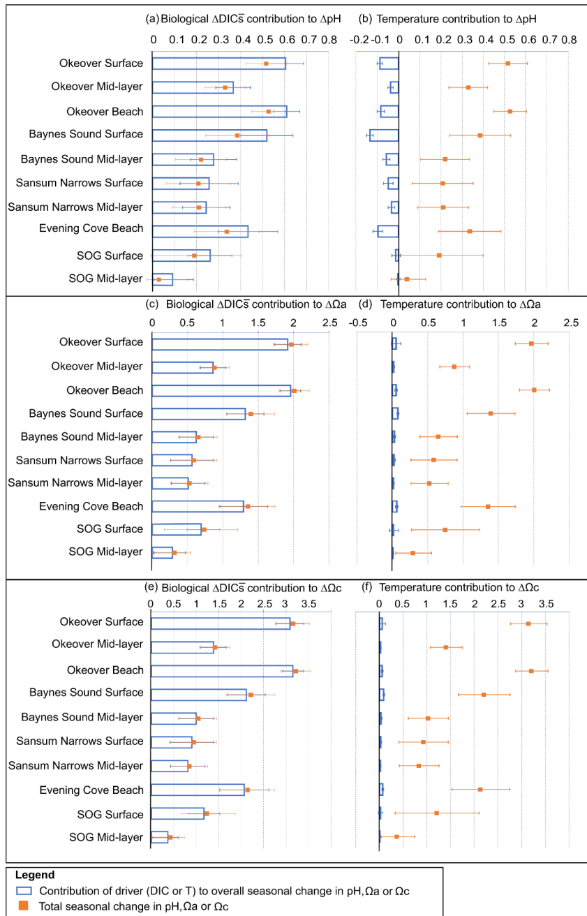
425 Figure 5. For each location, contribution of seasonal (winter to summer) biologically driven change in DIC (DICs) (left column) and seasonal temperature change, (right column) to seasonal change in pH (a,b), \Omega_a (c,d) and \Omega_c (e,f) (blue bars), respectively. Total seasonal change in pH, \Omega_a and \Omega_c resulting from all contributing drivers is shown in orange on each panel for comparison. Error bars are estimated from combining uncertainty from measurement, seasonal averaging, and partial derivative calculations (A3).
