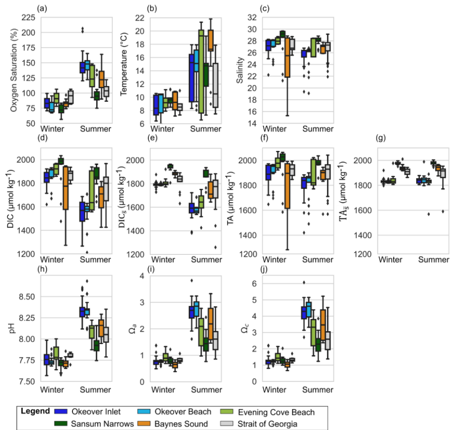
265 Figure 2 Observed variability at shellfish grow sites and adjacent waters in the surface layer (0-5 m) in winter and summer, respectively in a) dissolved oxygen (% saturation), b) temperature c) salinity, d) dissolved inorganic carbon (DIC), e) salinity normalized DIC ( DIC_s ), f) total alkalinity (TA), g) salinity normalized TA ( TA_s ), h) pH, i) \Omega_a and j) \Omega_c at nearshore locations shown in Fig. 1: Okeover (dark blue), Okeover beach (light blue), Evening Cove beach (light green), Sansum Narrows (dark green), Baynes Sound (orange) and ship collected data from the SOG (grey). Data have been split into a summer season capturing phytoplankton blooms (April-September) and winter season (October-March) when productivity is low. The mean annual salinity (Table A3) at each location was used to normalize DIC and TA, to show the impact of dilution. There is inter-seasonal variability at all locations and generally greater variability and range of conditions during the summer season, with the exception of salinity during the winter season in Baynes Sound. Boxes represent the interquartile range in conditions, middle bars are the median value and outer bars the full range in values, and points are outliers. The number of samples used to generate plots is given in Table A8. 270
