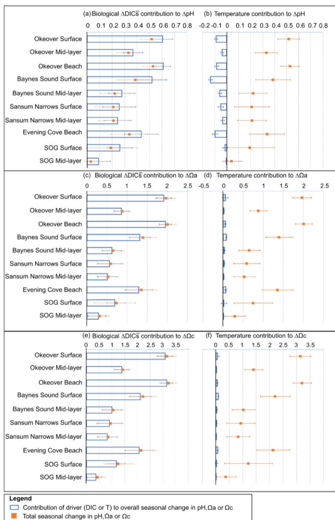
430 Figure 5. For each location, contribution of seasonal (winter to summer) biologically driven change in salinity normalised dissolved inorganic carbon-DIC (DICs) (left column) and seasonal temperature change. (right column) to seasonal change in pH (a,b), \Omega_a (c,d) and \Omega_c (e,f) (blue bars), respectively. Total seasonal change in pH, \Omega_a and \Omega_c resulting from all contributing drivers is shown in orange on each panel for comparison. Error bars are estimated from combining uncertainty from measurement, seasonal averaging, and partial derivative calculations (A3).
