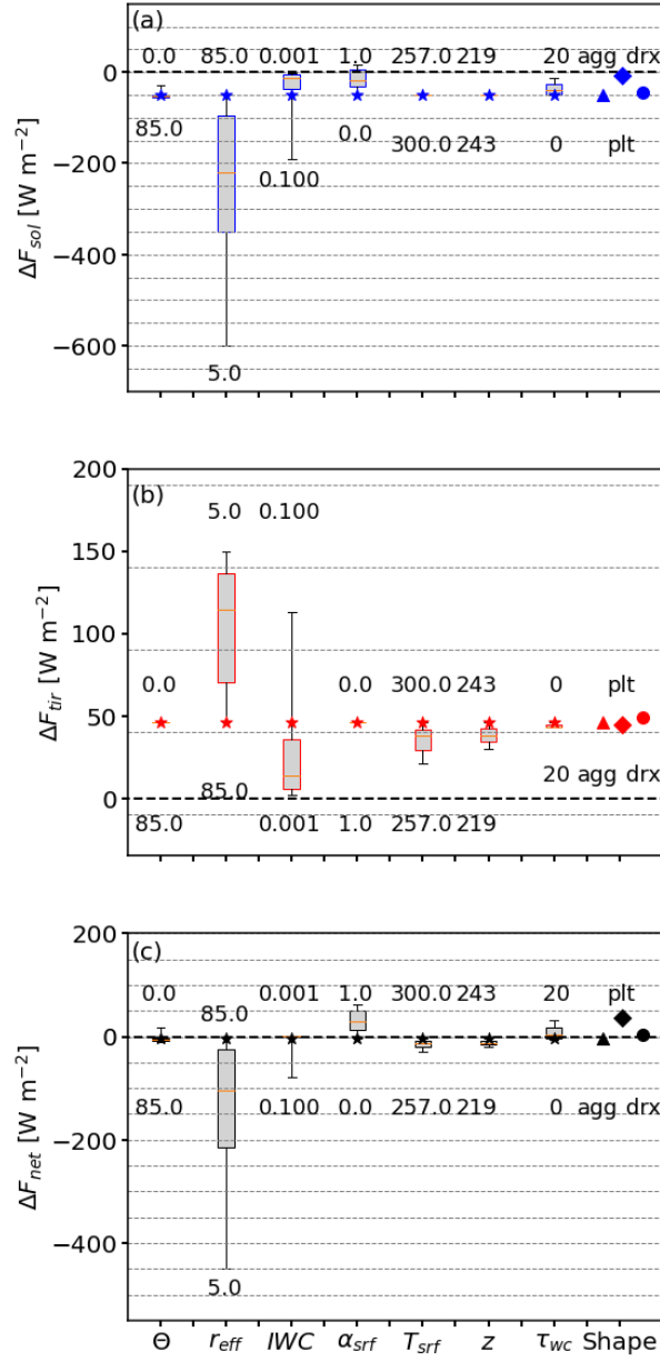
Figure 2. (a–c) Box and whisker plot of solar, TIR, and net \Delta F (in W m -2 ) due to the variation of the parameters indicated as the x -axis. The boxes represent the 25 th – and 75 th -percentiles, while the whiskers indicate the minimum and maximum values. Median values are given in each box by horizontal, orange lines. The stars indicate the reference with solar zenith angle \theta = 0^\circ , effective radius r_{\text{eff}} = 85 \mu\text{m} , ice water content \text{IWC} = 0.024 \text{ g m}^{-3} , surface albedo \alpha_{\text{srf}} = 0 , surface temperature T_{\text{srf}} = 299.7 \text{ K} , ice cloud temperature T_{\text{cld,ice}} = 219 \text{ K} , and liquid water cloud optical thickness \tau_{\text{liq}} = 0 . Minimum and maximum of the parameter ranges are given by the numbers. Plot idea adapted from Meerkötter et al. (1999).
