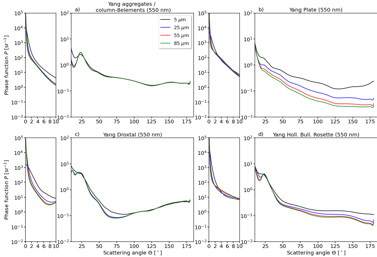
Figure D1. Phase function of four different ice crystal shapes with moderate surface roughness and four particle size distributions at 550 nm wavelength. Plot of the (1,1)-element of the scattering phase matrix. Please note the two different y -scales to account for the different magnitudes in the forward scattering peak. Plotted \mathcal{P} are post-processed phase functions from Emde et al. (2016) that are based on Yang et al. (2013). The phase functions from Emde et al. (2016) assume a crystal size distribution that follows a gamma function.
