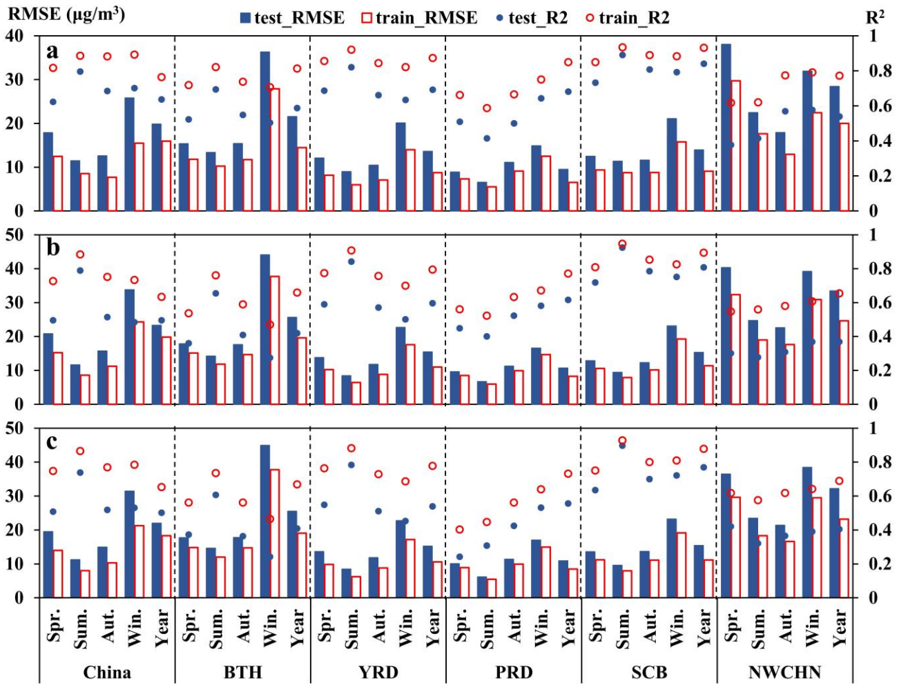
485 Figure 4. Cross validation (5-fold) results of CMAQ bias model training by meteorology (a), PM 2.5 components (b), and source sectors (c). RMSE unit: \mu\text{g}/\text{m}^3 .
