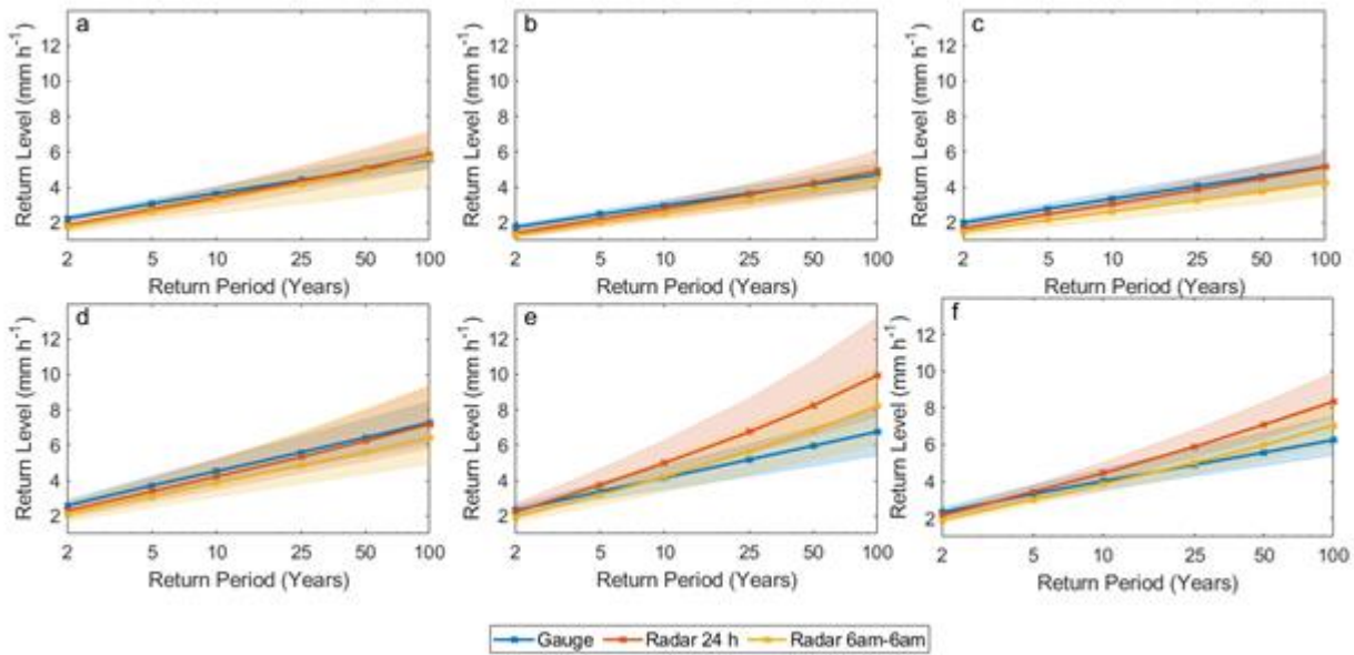
300 Figure 3: Comparison of the 100 km 2 , 24 h precipitation intensity return levels derived from 24 h radar data, daily 06:00 to 06:00 UTC data and from rain gauge data. The location of the 100 km 2 boxes are displayed in Fig. 1.
