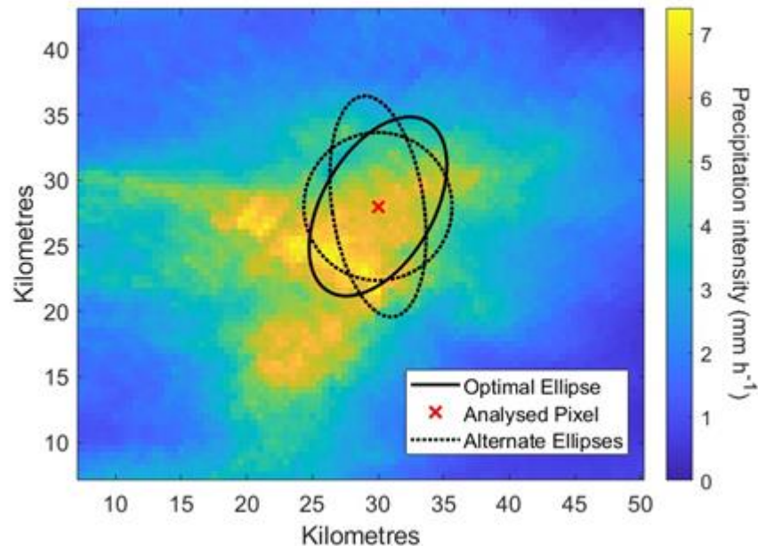
Figure 2: Optimum ellipse identification for an area of 500 km 2 and duration of 1 h around an analysed pixel. The selected optimum ellipse and 2 rejected ellipses are shown.
