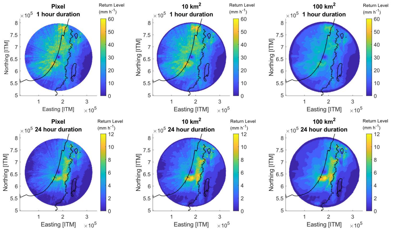
340 Figure 4: Precipitation intensity return levels for varying areas and durations for 25-year return periods. The coastline, the Sea of Galilee in the north, and the Dead Sea in the south are marked by the solid black line. The surface water divide is marked by the black dotted line.
