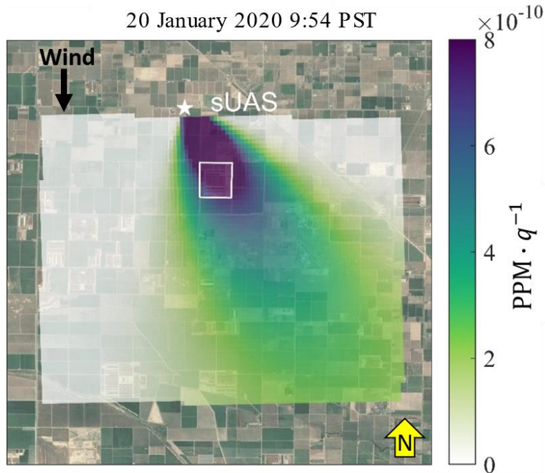
Figure 11. A satellite image from MathWorks overlaid with the footprint map obtained from the dispersion model. The white star shows the location of the UAAS operations, and the white rectangle shows the location of the upwind dairy farm. The color bar units are in ppm per unit of emission.
