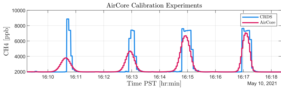
Figure 8. Results from the AirCore calibration experiment.
