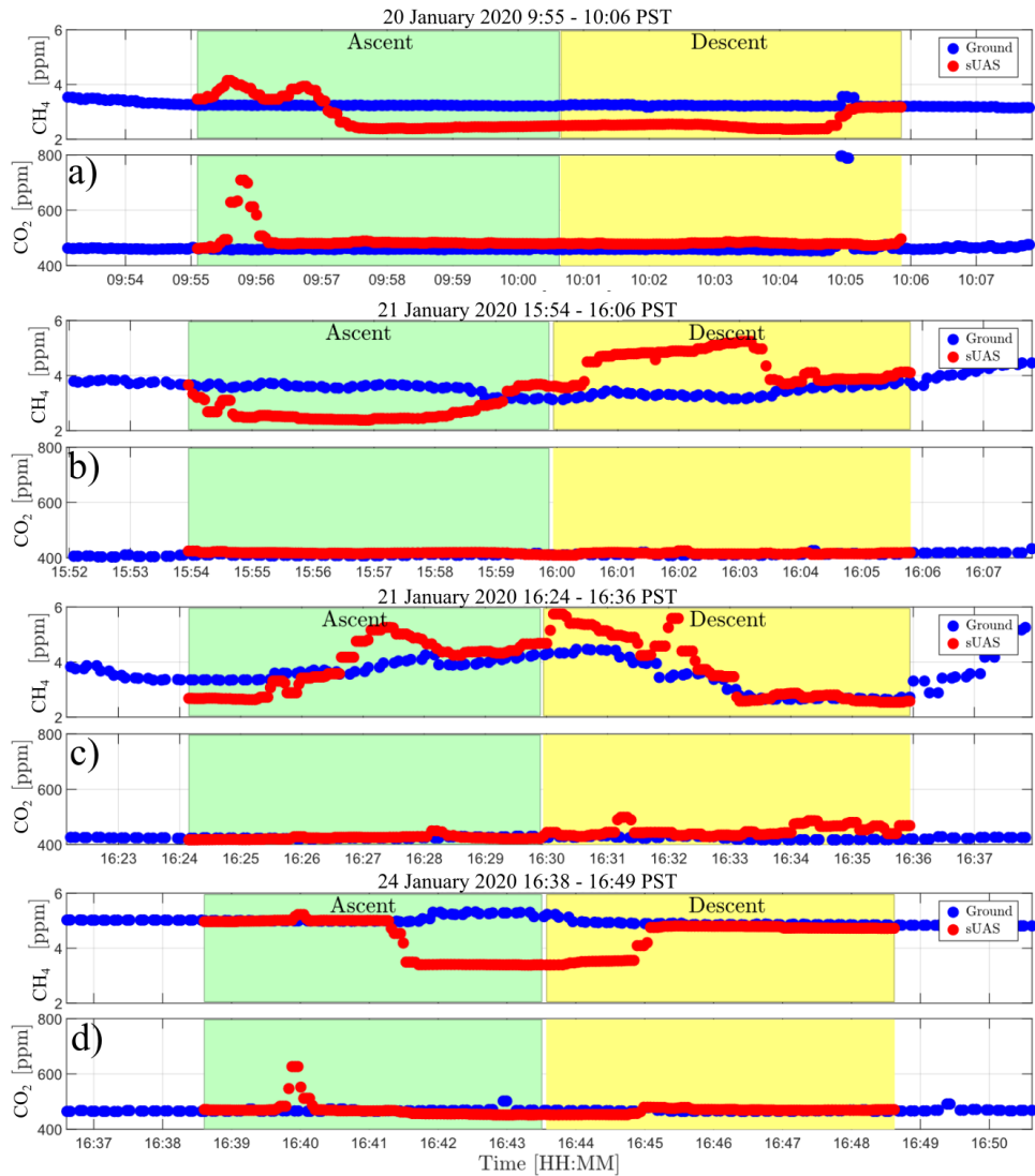
295 Figure 9. Comparison of UAAS (red) and ground-level (blue) observations of CH 4 and CO 2 .
