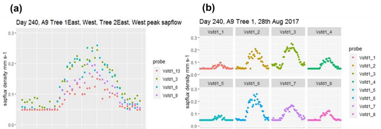
Figure C1: a) Example Stage 4 output showing peak point sap flux density in two trees for one sunny day in August 2017. Tree 1 (vsfd1_3 and vsfd1_6) bark radius is larger than Tree 2 (vsfd1_9 and vsfd1_13). b) Example Stage 4 output showing changes to point sap flux density across the active xylem for E facing (top) and W facing (bottom) probesets of one tree (Tree 1) on the same day in August 2017. The lefthand probe position is nearest to the bark and the righthand probeset position is nearest to the heartwood. Note the peak value occurs at different sensor positions for the two probesets.
