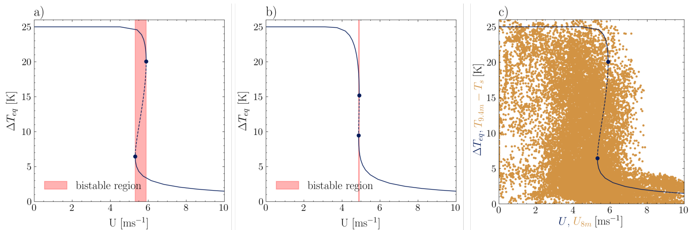
Figure 1. Equilibrium points of the model with a) short-tail and b) long-tail stability function plotted over wind speed. The dotted lines mark unstable equilibria while the solid lines correspond to stable ones. The red region is the region with two possible solutions for the same forcing conditions. In plot c) the orange dots are observational data from Dome C and the blue line corresponds to the equilibrium solutions of the model with a short-tail stability function.
