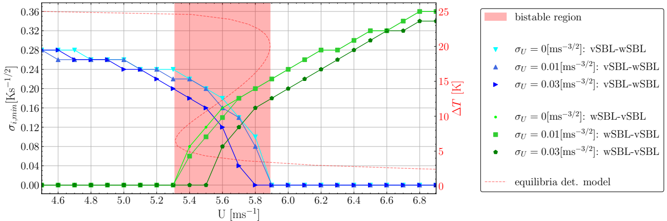
Figure 8. Results of the sensitivity study of model (6). For every U the minimal \sigma_i ( \sigma_{i,min} ) for which at least 80% of the 500 simulations have at least one transition of the indicated type is marked. Simulations with an initial condition \Delta T_0 = 24\text{K} are plotted in green and with \Delta T_0 = 4\text{K} in blue. The red dotted line is the bifurcation diagram of the deterministic model (eq. 2) and its bifurcation region is the red shaded area.
