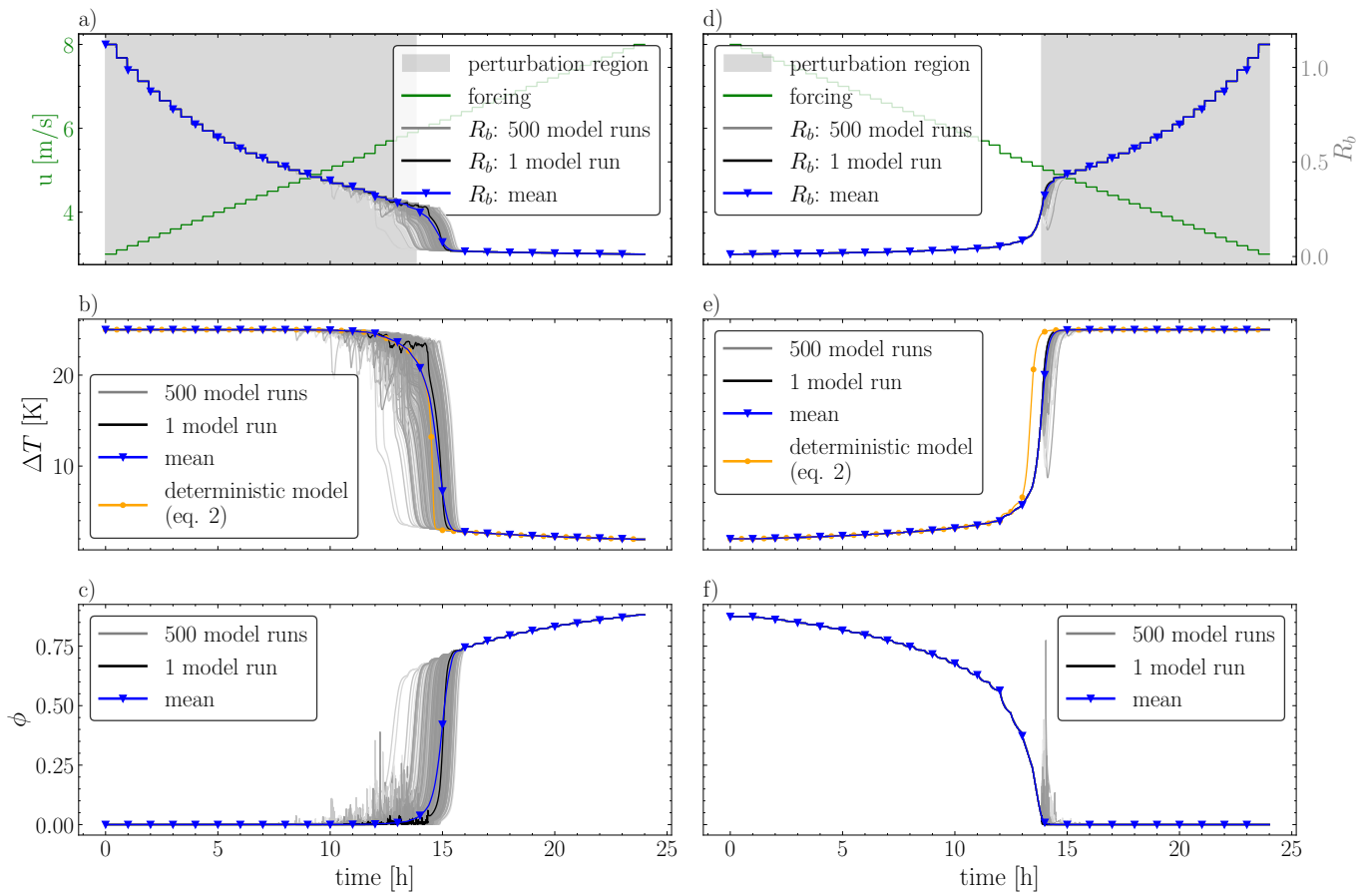
Figure 10. Solution of the model with perturbed stability function and variable forcing parameter U (wind velocity). In the left column the simulations were started in the vSBL state and U increases. In the right column the simulations were started in the wSBL state and U decreases. Panel a) and d) show the time evolution of the forcing, panel b) and e) of \Delta T , and c) and f) of the stability function.
