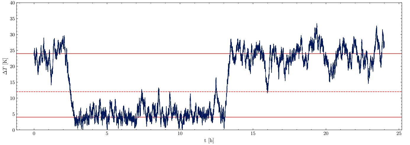
Figure 5. Plot of one solution of equation 4 with U = 5.6 \text{ ms}^{-1} and \sigma_i = 0.18 \text{ Ks}^{-1/2} . The red dotted line marks the unstable equilibria of the deterministic model while the solid lines correspond to stable ones.
