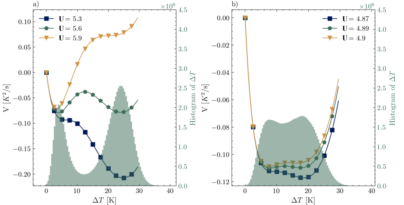
Figure 3. Potentials with a) short-tail and b) long-tail stability function for several wind speeds U and histograms of the results of 1000 simulations of the model with additive noise. In plot a) the mean of the random wind speed used to produce the histograms is equal to 5.6 \text{ ms}^{-1} and in plot b) to 4.89 \text{ ms}^{-1} .
