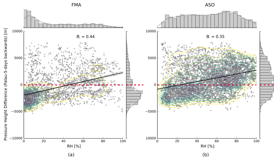
Figure A7. Measured relative humidity (RH) in relation to from observations above Palau versus difference in pressure altitude (measured 5 between measurement date in Palau and five days before measurement) derived-inferred from the backward trajectory analysis for the seasons FMA (a) and ASO (b); grey "+" indicate individual measurements from the trajectory dataset; colored contours show the distribution density; the black line indicates a fit by linear regression with a grey shaded 95 % confidence interval; the red dashed line highlights the zero line for the altitude difference with positive values indicating ascent and negative values descent towards Palau; the correlation coefficient R is shown in the plot; the marginal plots show univariate histograms and kernel-density estimated curves.
