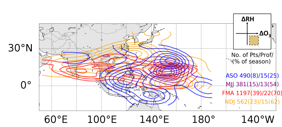
Figure A8. Seasonal distributions of the location of \Delta O_3 + \Delta RH - air masses five days before their measurement in Palau in the 5–10 km altitude range inferred from trajectories , according to the definition shown in Fig. 7 from 5-days backward trajectory-earliest points arriving in Palau within 5–10 km ; numbers in the plot from left to right: absolute number of individual air masses (points/trajectories) per season and profiles as percentage per season given in brackets, absolute values number of profiles per season given and as seasonal fraction percentage per season in brackets; differences to numbers shown in Fig. A6 due to rounding differences; see Fig. 6 for seasons.
