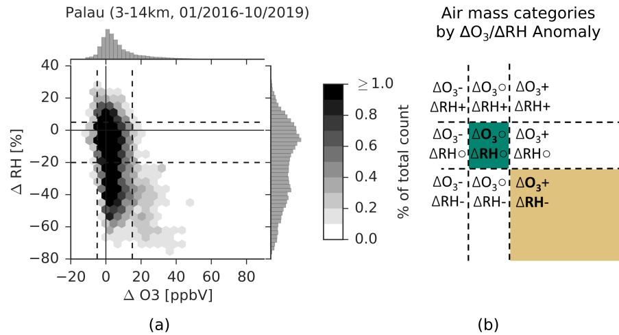
Figure 7. (a) Free-tropospheric (3-14 km) relation between tracer anomalies \Delta O_3 VMR and \Delta RH from the monthly background profiles defined in Section 3.1; color shading indicates percentages of total count of measured O_3/RH data pairs per grid point; marginal plots for individual tracer anomaly distributions are normalized to unity; dashed lines refer to quantitative air mass categories in the three times three quantitative grid as illustrated in (b), with boundary values for the central grid box ( \Delta O_{3\circ}\Delta RH_{\circ} ) of -5/+15 ppb for \Delta O_3 VMR and -20/+5 % for \Delta RH ; two target categories of the analysis are highlighted in color in (b), compare to Fig. 3.
