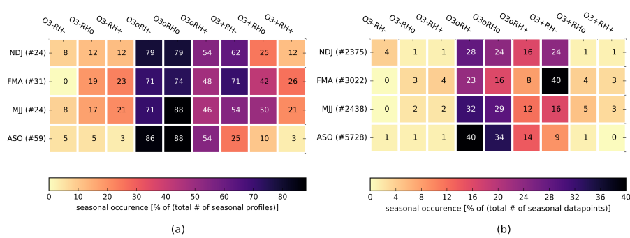
Figure A6. Heat map for the seasonal occurrence of air mass anomaly categories \Delta O_3/\Delta RH regarding based on the definition given in Sect. 3.1.3 and presented in Fig. 7 for Palau observations in the 5-10-5-10 km altitude range (trajectory dataset, see Sect. 2); panel (a) shows the occurrence relative to the total number (#) of seasonal profiles and panel (b) relative to the total number of all data points within the season; total numbers are given in brackets per season.
