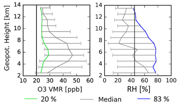
Figure 4. O_3 VMR and RH statistics for the month of March as example for Palau free tropospheric profiles per-km as a function of altitude : the 20th quantile (Q20) for O_3 is shown in green and the 83.3th quantile (Q83) for RH in blue (both vertically smoothed using exponentially weighted moving averages); the median is marked in grey and the central 66.6 % range in grey horizontal bars; number of included individual profiles in brackets, for orientation 20 ppb O_3 VMR and 45 % RH are marked in black (see also Figs. A3 and A4).
