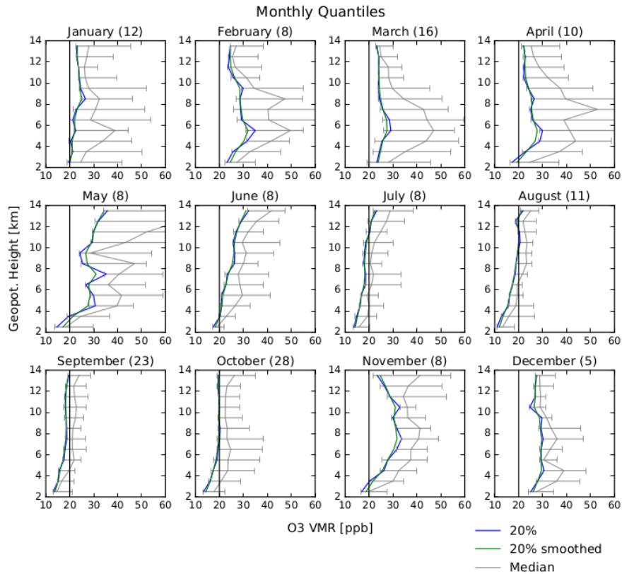
Figure A3. Monthly O 3 VMR statistics for Palau free tropospheric profiles per-km as a function of altitude : 20th quantile (Q20) in blue, vertically smoothed using exponentially weighted averages in green, median in grey and central 66.6 % range in grey horizontal bars; number of included individual profiles in brackets, for orientation 20 ppb O 3 VMR is marked as a black vertical line (compare Figs. 4 and A4).
