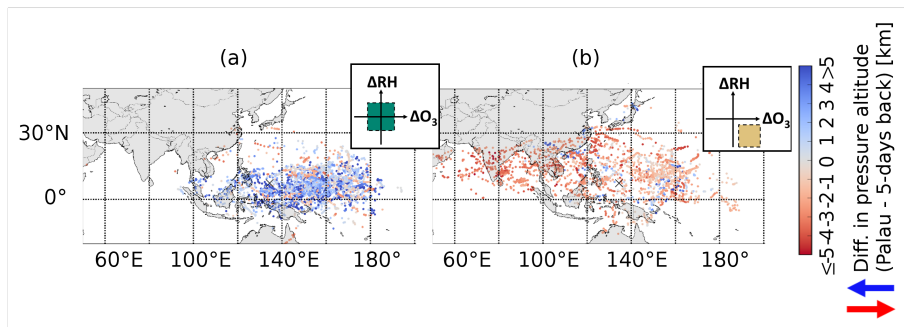
Figure 11. Origin of air masses by air mass anomalies: 5-days backward trajectory earliest points arriving Location of air masses five days before their measurement in Palau in the 5-10-5-10 km altitude range inferred from trajectories for \Delta O_3 \Delta RH (a) and \Delta O_3 + \Delta RH (b) air masses, as indicated by the pictograms, color-coded by difference in pressure altitude sonde endpoint between measurement and five days before measurement , see also Figs. 7 and 10.
