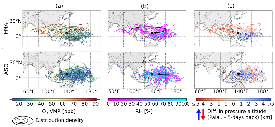
Figure 10. Origin of air masses by season: 5-days-backward-trajectories' earliest-points-arriving Location of air masses five days before their measurement in Palau in the 5-10 km altitude range inferred from trajectories for Palau seasons FMA (upper row) and ASO (lower row); color-coded either by O 3 VMR (a) or, RH (b), both measured at Palau, or and by difference in pressure altitude, measured at Palau minus 5-between measurement and five days before measurement (c); in-addition, black contours in (a) show distribution density and schematic arrows in (b) indicate the pathway as shown by the footprint in Fig. 9; see Fig. 6 for seasons.
