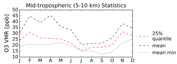
Figure A2. Statistical O 3 VMR measures for the 5-10 5-10 km altitude range highlighting the minimum O 3 season: monthly means from individual soundings' 25 % quantiles (red dashed line), mean (black dashed line) and minimum (black dotted line).
