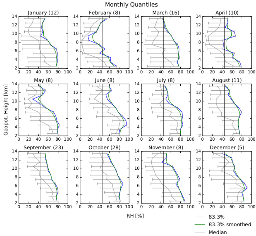
Figure A4. Monthly RH statistics for Palau free tropospheric profiles per km as a function of altitude : 83.3th quantile (Q83) in blue, for more details see Fig. A3; 45% RH is highlighted by a black vertical line (compare Figs. 4 and A3).
