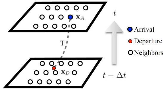
Figure 1. Procedure of time marching in semi-Lagrangian scheme.
