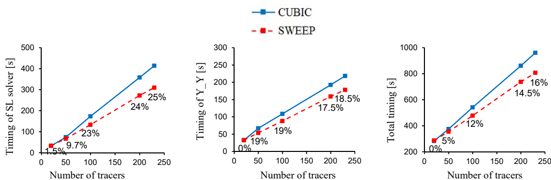
Figure 8. Computational time analysis based on the number of tracers.
