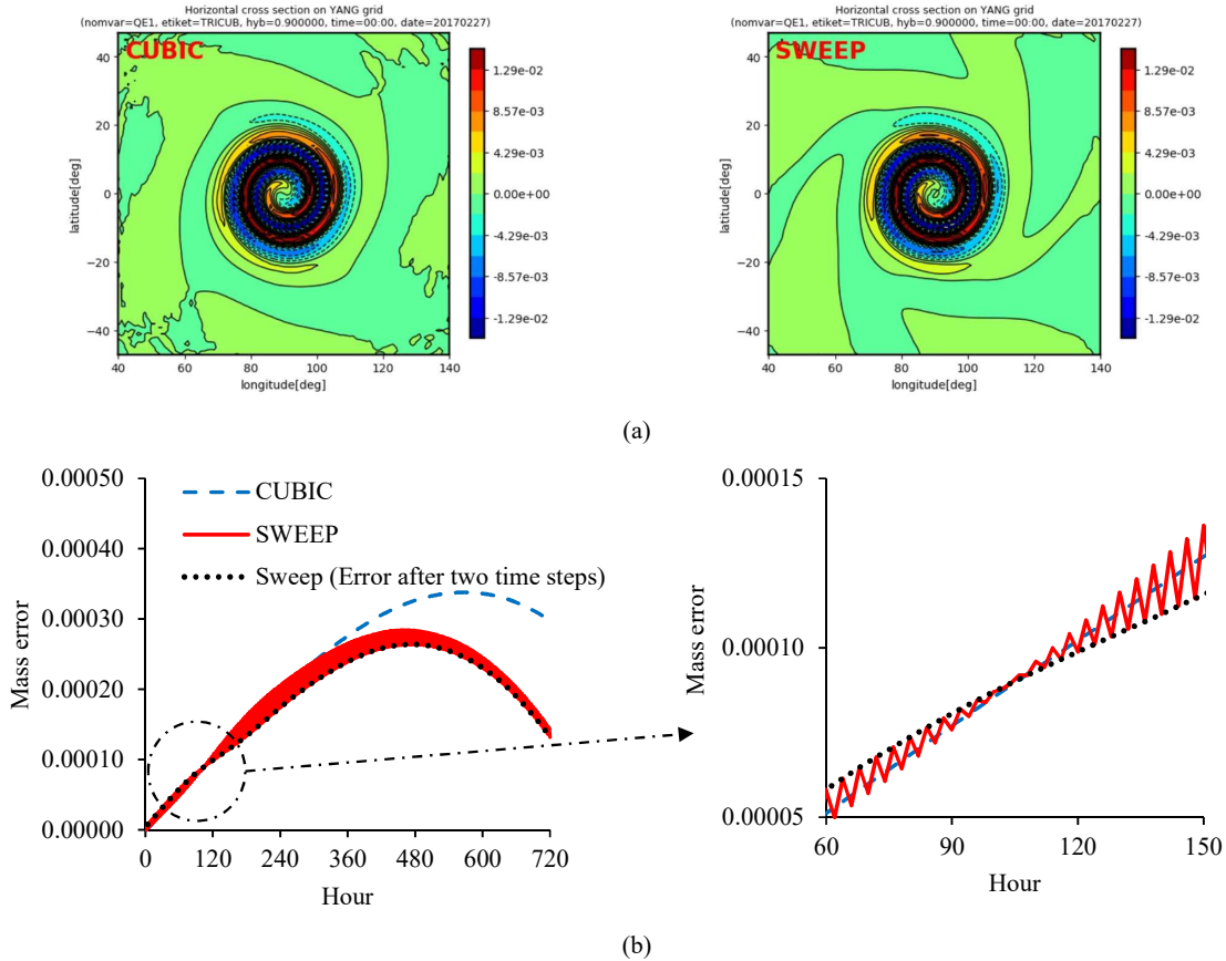
Figure 3. 2D vortex: (a) Errors in tracer distribution at day 12, (b) Mass conservation error (in %) over 1 month period.
