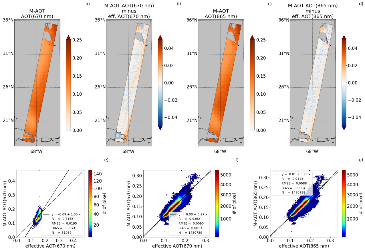
Figure 4. Same as Figure 3 but for the Halifax-Aerosol scene.
