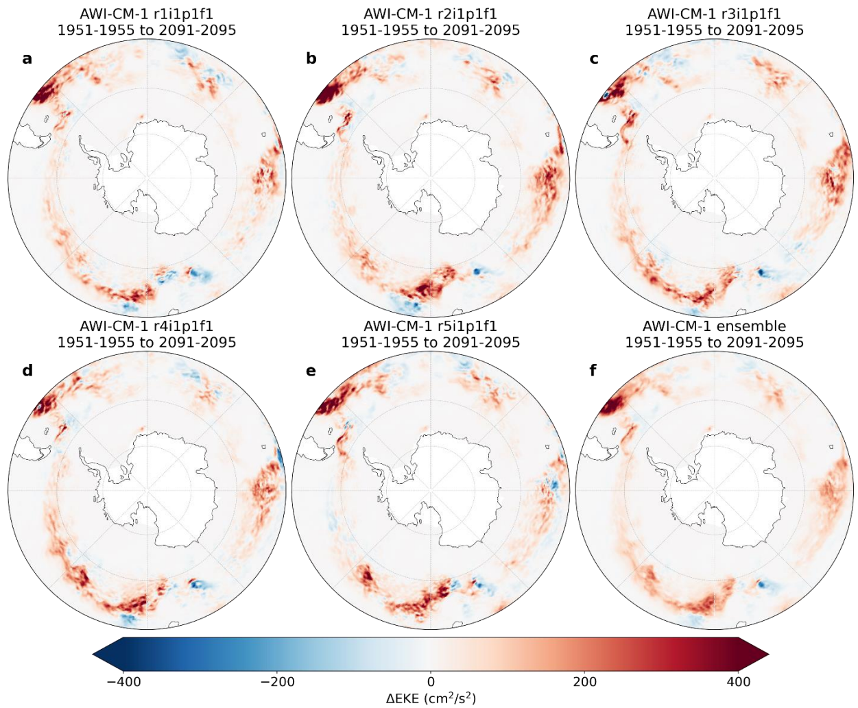
Supplementary Figure 4. Ensemble spread of EKE change between 1951-1955 and 2091-2095. EKE change in (a-e) each member of the AWI-CM-1 ensemble and (f) the ensemble mean.
