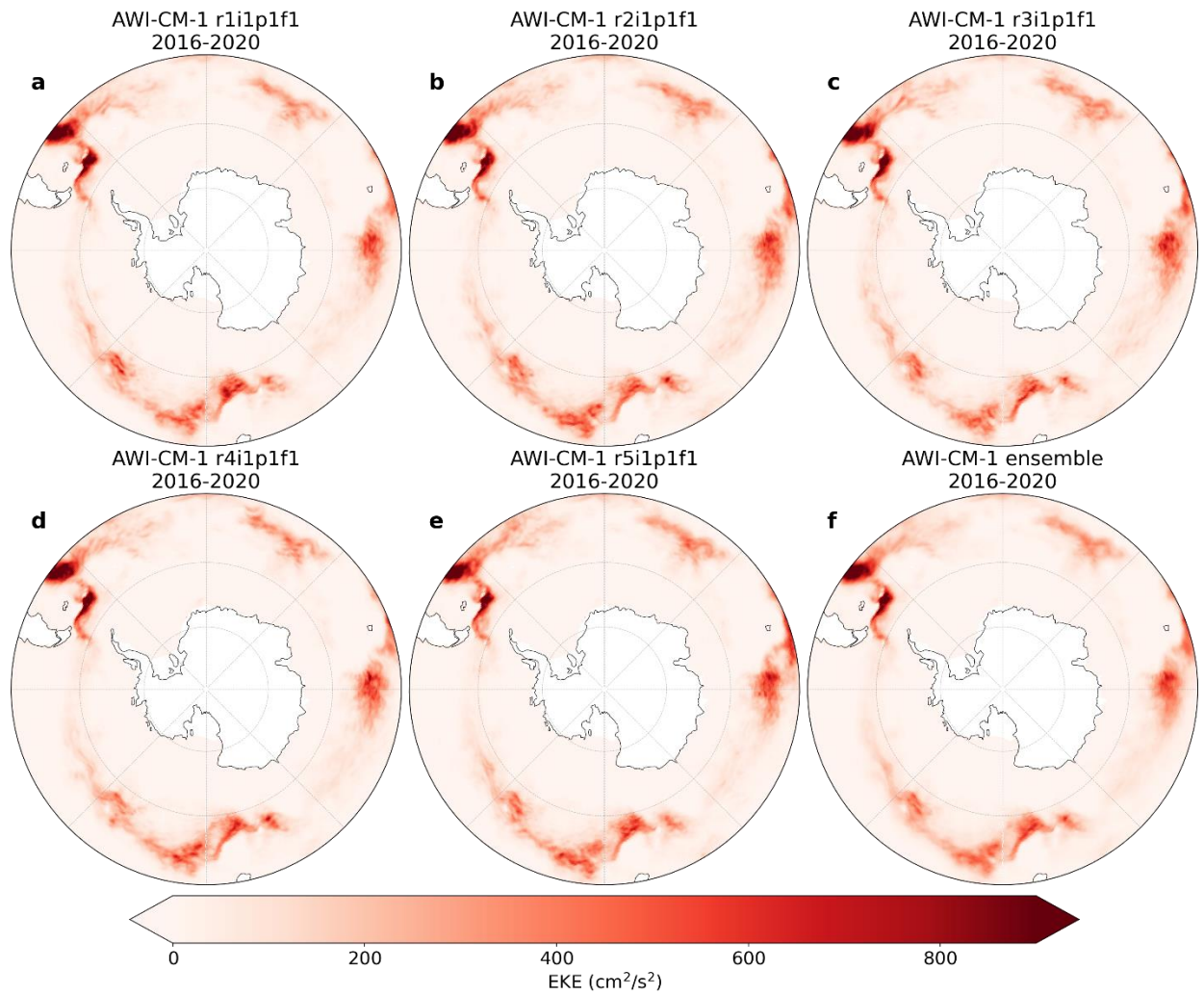
Supplementary Figure 2. Ensemble spread of mean EKE. Mean EKE during 2016-2020 in (a-e) each member of the AWI-CM-1 ensemble and (f) the ensemble mean.
