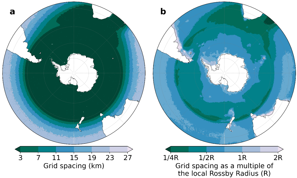
Supplementary Figure 1. Grid resolution of the SO3 mesh. a) grid resolution expressed as approximate node spacing. b) Grid resolution expressed as a multiple of the local Rossby radius.
