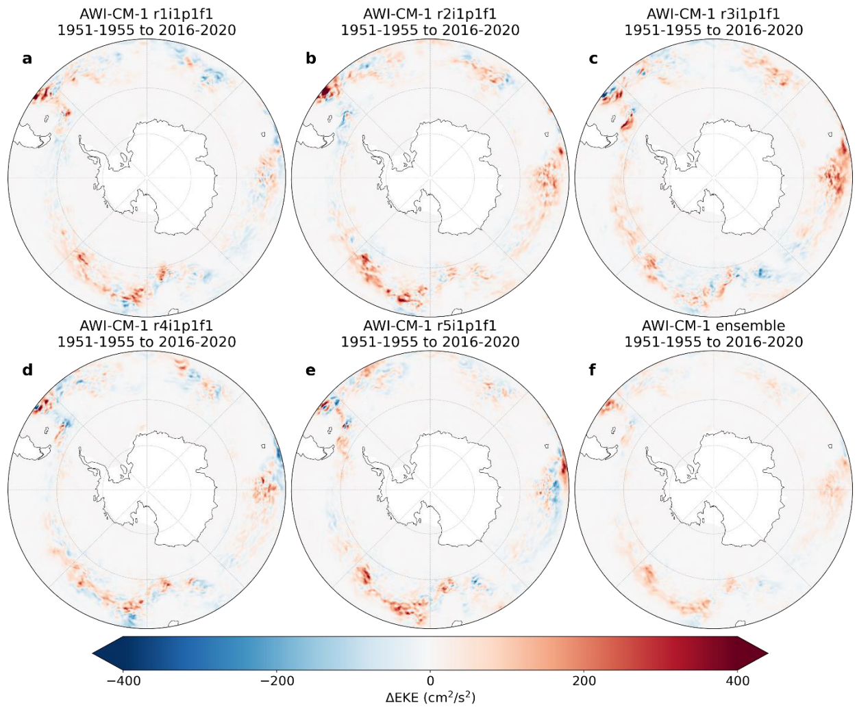
Supplementary Figure 3. Ensemble spread of EKE change between 1951-1955 and 2016-2020. EKE change in (a-e) each member of the AWI-CM-1 ensemble and (f) the ensemble mean.
