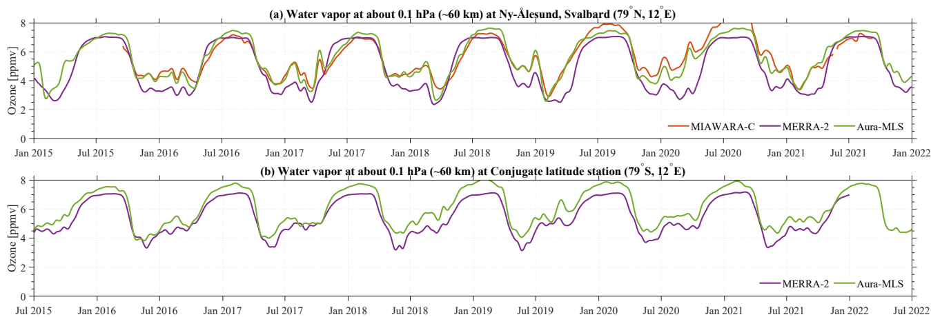
Figure B2. MIAWARA-C, MERRA-2, and Aura-MLS water vapor VMR time series at 0.1 hPa smoothed by a 30-day running mean over Ny-Ålesund, Svalbard (79° N, 12° E) and conjugate latitude station (79° S, 12° E).
