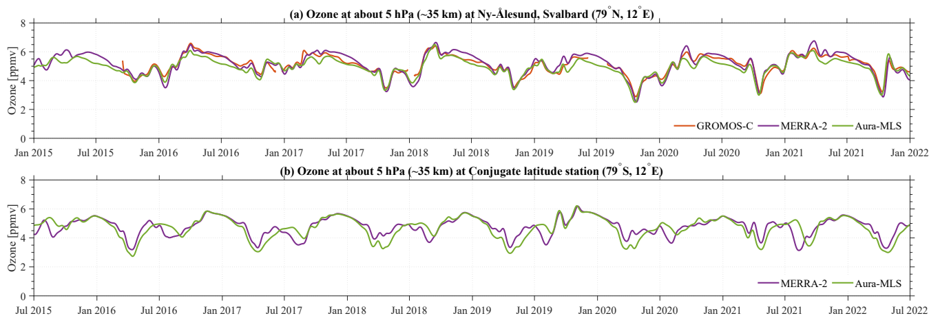
Figure B1. GROMOS-C, MERRA-2, and Aura-MLS ozone VMR time series at about 5 hPa smoothed by a 30-day running mean over Ny-Ålesund, Svalbard (79° N, 12° E) and conjugate latitude station (79° S, 12° E).
