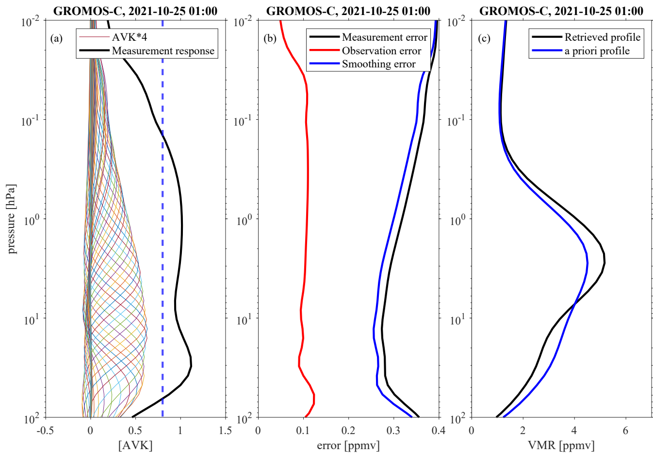
Figure A1. Example of GROMOS-C hourly ozone retrievals on 25 October 2021 around 01:00 UT: (a) shows the averaging kernels together with measurement response, (b) shows the measurement, smoothing, and observation errors, (c) shows the retrieved and a priori ozone profile.
