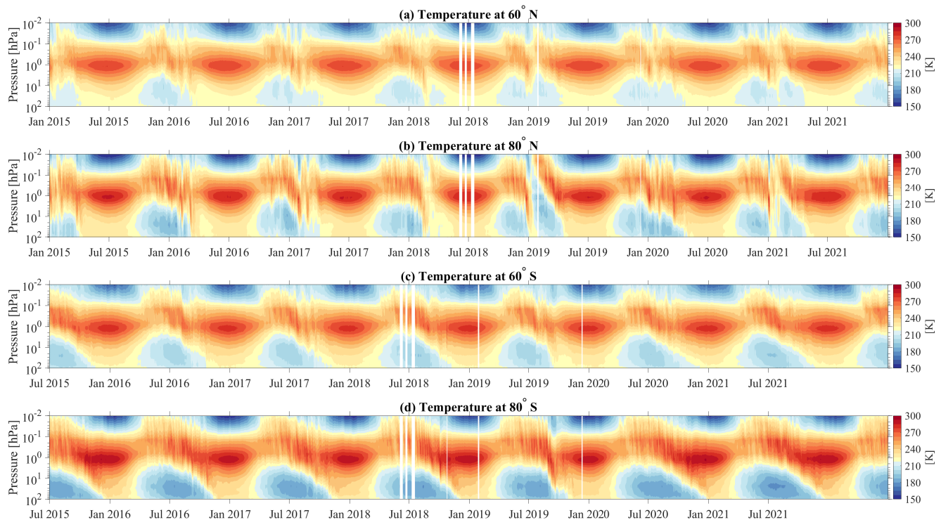
Figure C1. Time series of temperature from Aura-MLS observations as a function of pressure over conjugate polar latitudes ( 80^{\circ} N & 80^{\circ} S) and conjugate mid-latitudes ( 60^{\circ} N & 60^{\circ} S) in both hemispheres.
