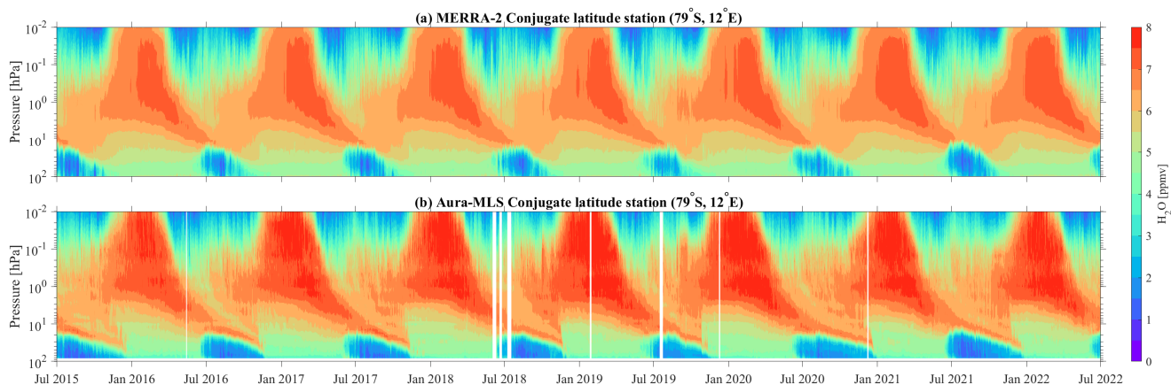
Figure 10. Same as Fig. 8 (without MIAWARA-C measurements) but for the SH at conjugate latitude station (79° S, 12° E).
