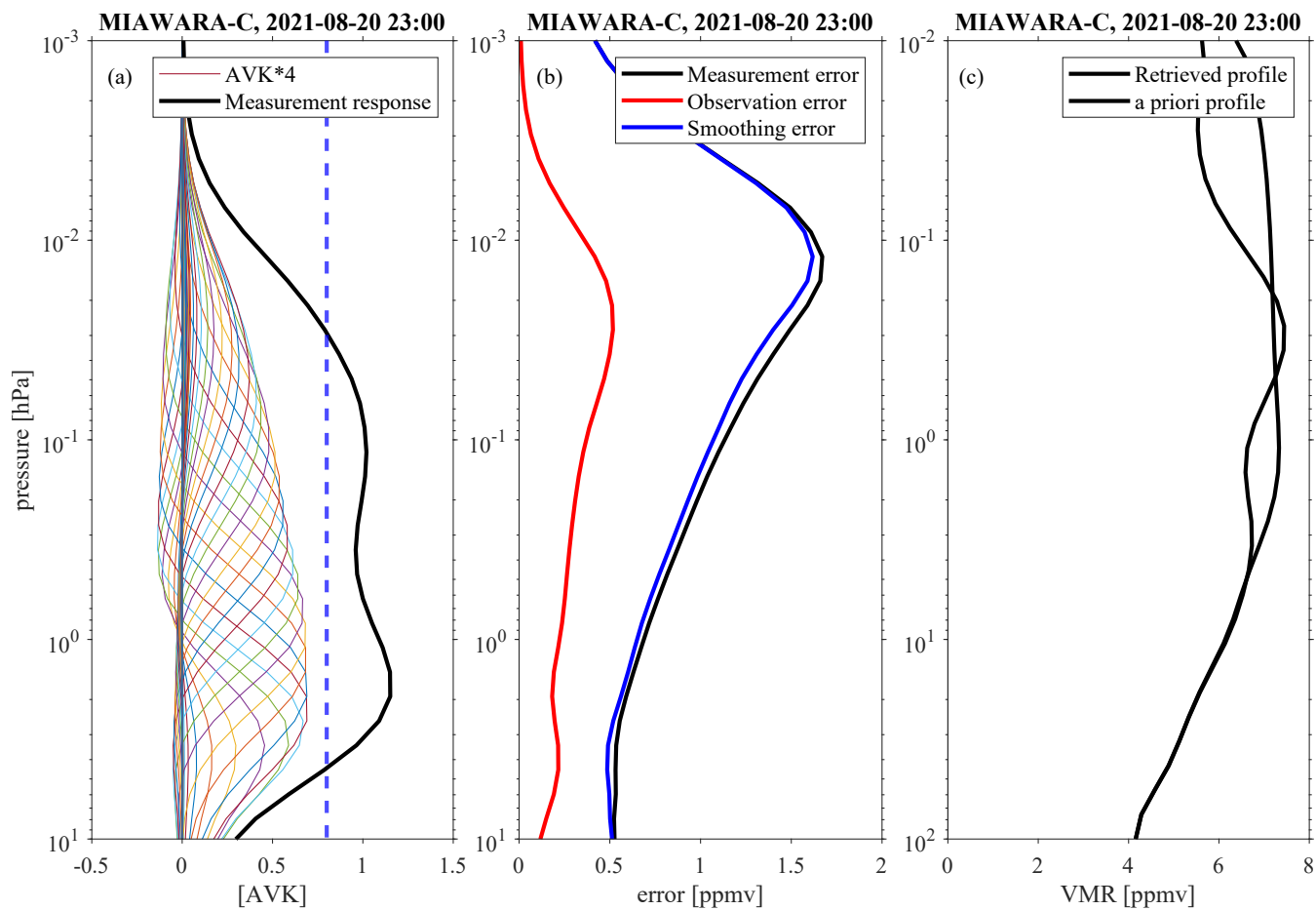
Figure A2. Example of MIAWARA-C hourly water vapor retrievals on 20 August 2021 around 23:00 UT: (a) shows the averaging kernels together with measurement response, (b) shows the measurement, smoothing, and observation errors, (c) shows the retrieved and a priori water vapor profile.
