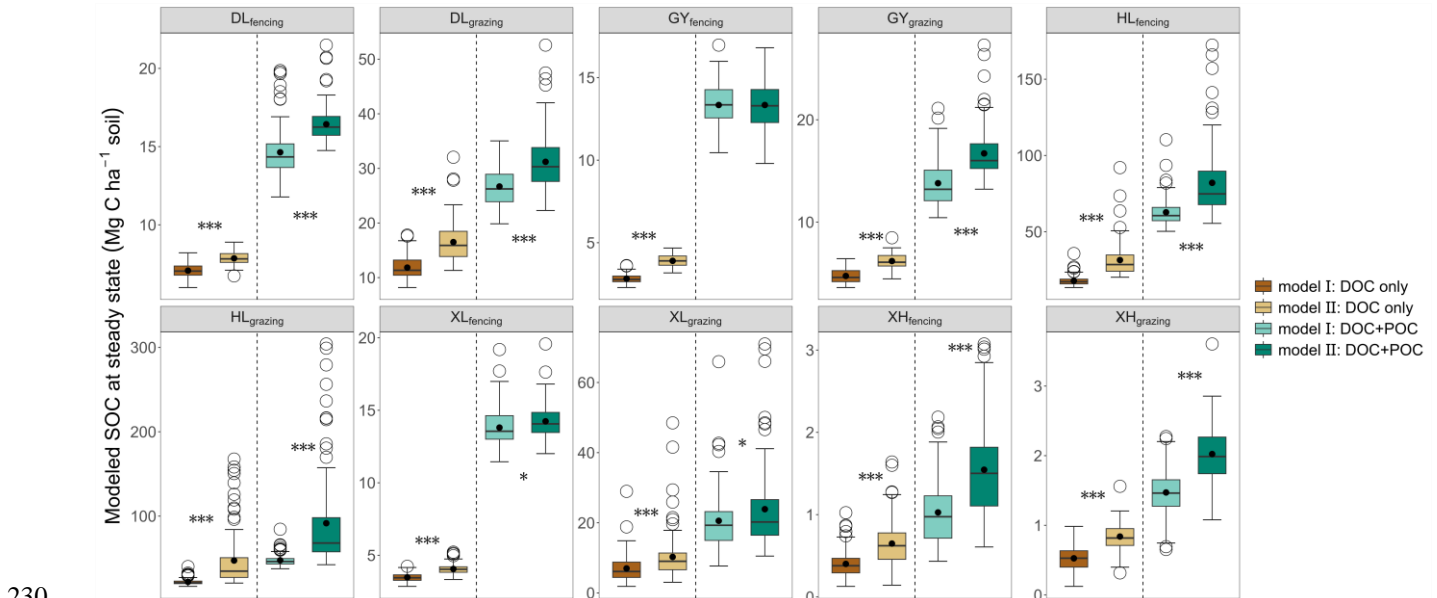
Figure 4: Modeled SOC content at steady state under two types of C input conditions. The two different C input scenarios for each site are separated by a dotted line. The upper and lower ends of boxes denote the 0.25 and 0.75 percentiles, respectively.
