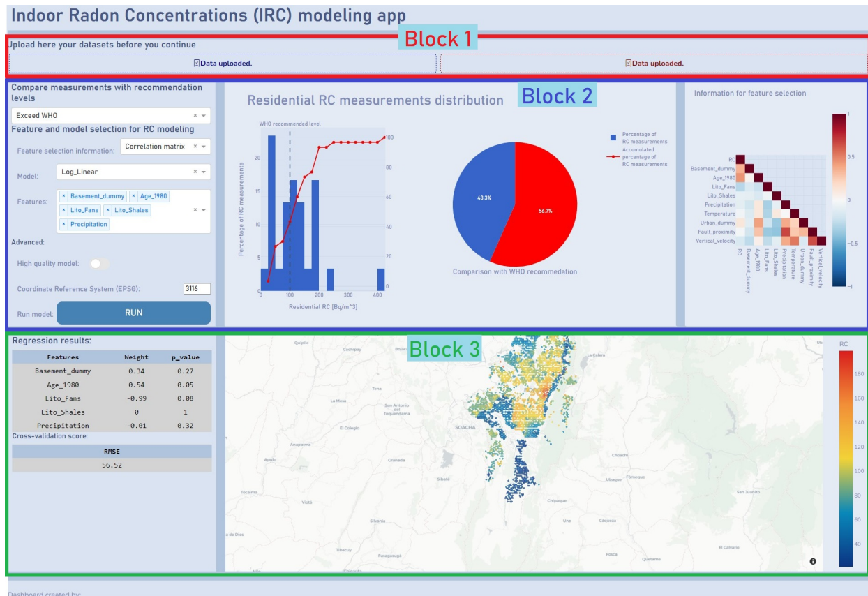
Figure 5. Overview of layout of the indoor radon concentration modeling dashboard developed. The three blocks that make up the dashboard are highlighted in red (1), blue (2) and green (3). Block 1 is the data uploading block, where the user can upload both datasets use for modeling (The in-situ measurements and the cadaster dataset). Block 2 presents visualizations of the in situ data and allows the user to chose the parameters and run the model. In this block the IRC distribution can be observed and some statistics from the in-situ dataset can be obtained (i.e. the percentage of measurements exceeding reference levels and correlations between covariates). Block 3 is the results block, where on the left panel the feature importance can be observed and on the right panel the prediction map is presented. The dashboard can be accessed at https://ircmodelingdashboard.eu.pythonanywhere.com/ . Figure created by authors.
