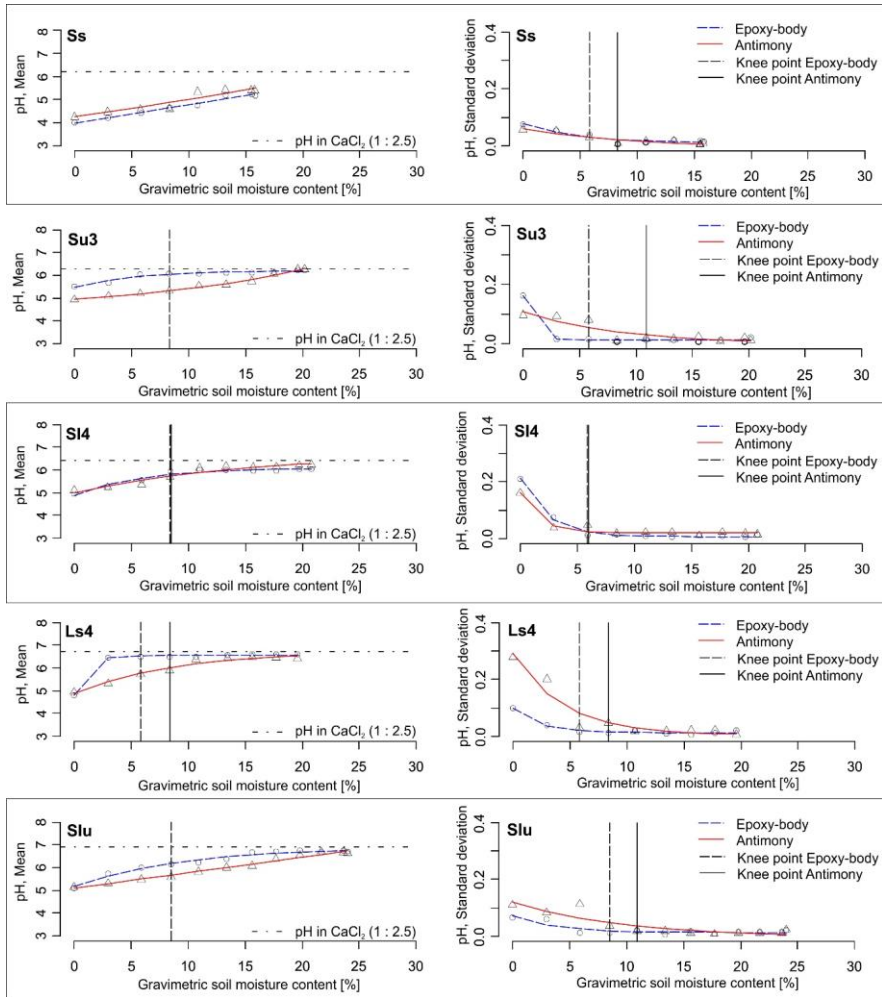
330 Figure 4. pH – SMC plots for different soil textures measured with the epoxy-body electrode and the antimony electrode. Left: Mean pH values, right: Standard deviations (n=5). Knee points are indicated by vertical lines.
