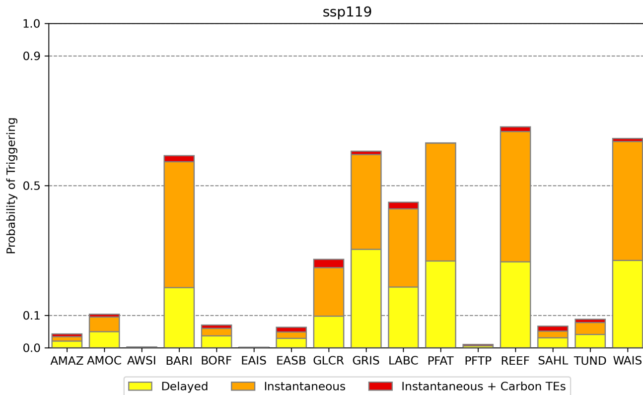
Figure 8. Probabilities of triggering the TEs by 2500 under SSP1-1.9 for the case of delayed triggering, instantaneous triggering and instantaneous triggering including the additional warming from carbon TEs.
