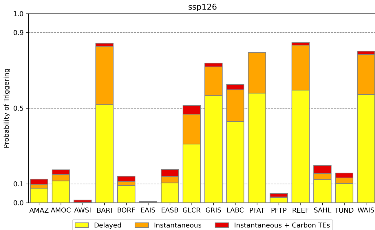
Figure 7. Probabilities of triggering the TEs by 2500 under SSP1-2.6 for the case of delayed triggering, instantaneous triggering and instantaneous triggering including the additional warming from carbon TEs.
