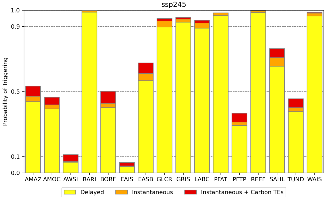
Figure 6. Probabilities of triggering the TEs by 2500 under SSP2-4.5 for the case of delayed triggering, instantaneous triggering and instantaneous triggering including the additional warming from carbon TEs.
