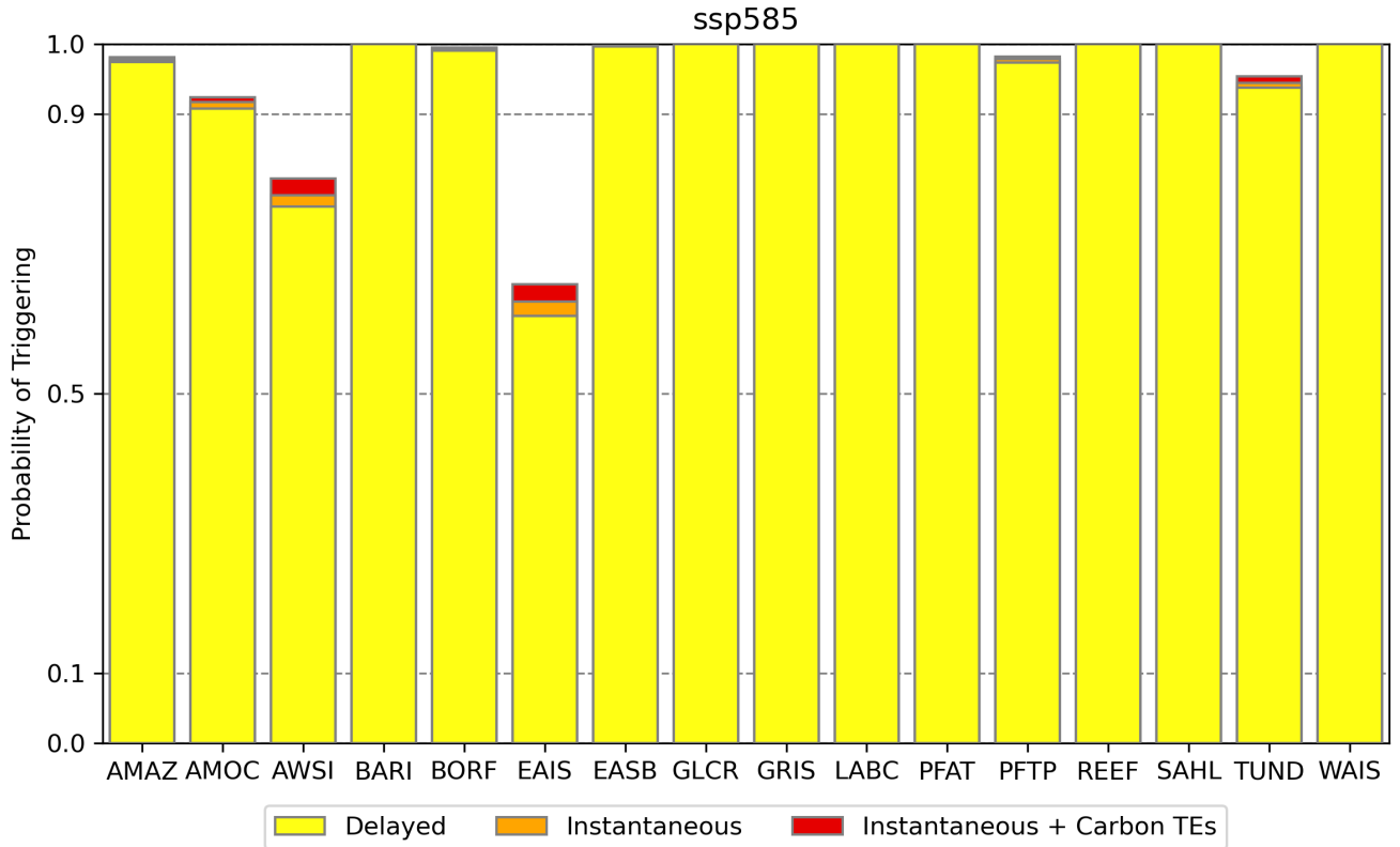
Figure 5. Probabilities of triggering the TEs by 2500 under SSP5-8.5 for the case of delayed triggering, instantaneous triggering and instantaneous triggering including the additional warming from carbon TEs.
