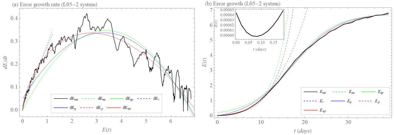
820 Figure 6. (a) Initial error growth tendency (rate) dE/dt as a function of the error magnitude E ( dE_{tot} , black), approximation of the early part of the growth by exponential growth rate dE_{ex} (Eq. (1), green, dashed), exponential growth rate with model error dE_r (Eq. (5), blue, dashed), power law dE_p (Eq. (3), red, dashed) and approximation of the full curve by growth rate of quadratic hypothesis dE_{qu} (Eq. (2), green), growth rate of hypothesis with model error dE_q (Eq. (6), blue) and extended power law dE_{ep} (Eq. (4), red) for the L05-2 system. (b) Initial error growth E as a function of time t ( E_{tot} , Eq. (11), black), approximation of the early part of the growth by integration of dE_{ex} ( E_{ex} , green, dashed) with \lambda_{ex} = 0.29 1/day, integration of dE_r ( E_r , blue, dashed) with \lambda_r = 0.26 1/day and \beta_r = 0.02 unit/day, integrations of dE_p ( E_p , red, dashed) with a = 0.25 unit 0.32 /day and b = 0.32 and approximation of the full curve by integration of dE_{qv} ( E_{qv} , green) with \lambda_{qv} = 0.2 1/day and E_{lim} = 6.8 unit, integration of dE_q ( E_q , blue) with \lambda_q = 0.18 1/day, \beta_q = 0.05 unit/day and E_{lim} = 6.8 unit and integration of dE_{ep} ( E_{ep} , red) with a = 0.28 unit 0.34 /day, b = 0.34 and E_{lim} = 7 unit for the L05-2 system. The inset shows transient behavior before the error magnitude grows (for more details, see Section 2.1). 825
