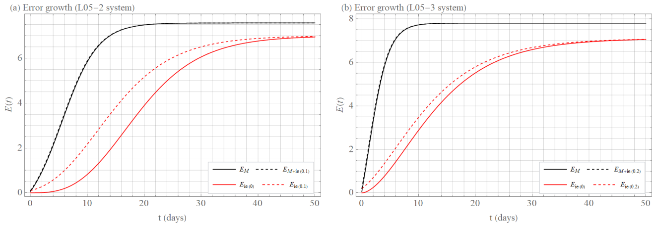
875 Figure 10. Error growth E as a function of time t . The full black curve shows model error growth E_M (Eq. (14)), the dashed black 880 curve shows initial and model error growth E_{M+ie} (Eq. (15)), the full red curve displays initial error growth E_{ie} for E(0) \rightarrow 0 (Eq. (11)), and the dashed red curve displays initial error growth E_{ie} for (a) E(0) \approx 0.1 and (b) E(0) \approx 0.2 (Eq. (11)). Shown are calculations of the best-fit approximations for given types of error growth (see Section 3 for more details). The initial error growth E_{ie} is calculated for (a) the L05-2 system and (b) the L05-3 system. The model error growth E_M and initial + model error growth E_{M+ie} is calculated as (a) the difference between the L05-1 system and the L05-2 system and (b) between the L05-1 system and the 880 L05-3 system.
