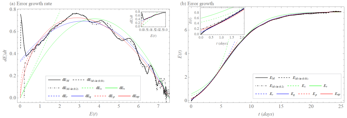
870 Figure 8. (a) Model error growth tendency (rate) dE/dt as a function of the error magnitude E ( dE_M , black), initial and model error growth tendency dE/dt as a function of the error magnitude E ( dE_{M+ie(0.01)} , black, dashed for E(0)=0.01 and dE_{M+ie(0.2)} , black, dot-dashed for E(0)=0.2 ), approximation of the early part of the model growth by exponential growth rate dE_{ex} (Eq. (1), green, dashed), exponential growth rate with model error dE_r (Eq. (5), blue, dashed), power law dE_p (Eq. (3), red, dashed) and approximation of the full curve by growth rate of quadratic hypothesis dE_{qu} (Eq. (2), green), growth rate of quadratic hypothesis with model error dE_q (Eq. (6), blue) and extended power law dE_{ep} (Eq. (4), red) for the L05-2 system as the "reality" and the L05-1 system as the "model." The inset shows the early phase. (b) Model error growth E as a function of time t ( E_M , Eq. (14), black), initial and model error growth E as a function of time t ( E_{M+ie(0.01)} , Eq. (15), black, dashed for E(0)=0.01 and E_{M+ie(0.2)} , Eq. (15), black, dot-dashed for E(0)=0.2 ), approximation of the early part of the growth by integration of dE_{ex} ( E_{ex} , green, dashed) with \lambda_{ex}=0.39 1/day, integration of dE_r ( E_r , blue, dashed) with \lambda_r=0.17 1/day and \beta_r=0.33 unit/day, integrations of dE_p ( E_p , red, dashed) with a=0.52 unit 0.64 /day and b=0.64 and approximation of the full curve by integration of dE_{qu} ( E_{qu} , green) with \lambda_{qu}=0.38 1/day and E_{lim}=7.5 unit, integration of dE_q ( E_q , blue) with \lambda_q=0.27 1/day, \beta_q=0.34 unit/day and E_{lim}=7.6 unit and integration of dE_{ep} ( E_{ep} , red) with a=0.61 unit 0.39 /day, b=0.39 and E_{lim}=7.6 unit for the L05-2 system as the "reality" and the L05-1 system as the "model." The inset shows the early phase of the time evolution. 880
