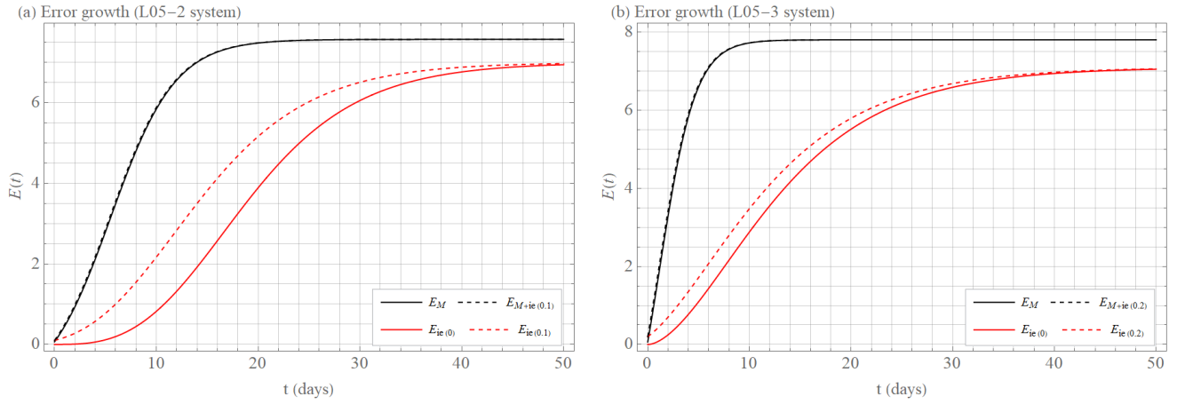
Figure 10. Error growth E as a function of time t . The full black curve shows model error growth E_M (Eq. (14)), the dashed black curve shows initial and model error growth E_{M+ie} (Eq. (15)), the full red curve displays initial error growth E_{ie} for E(0) \rightarrow 0 (Eq. (11)), and the dashed red curve displays initial error growth E_{ie} for (a) E(0) \approx 0.1 and (b) E(0) \approx 0.2 (Eq. (11)). Shown are calculations of the best-fit approximations for given types of error growth (see Section 3 for more details). The initial error growth E_{ie} is calculated for (a) the L05-2 system and (b) the L05-3 system. The model error growth E_M and initial + model error growth E_{M+ie} is calculated as (a) the difference between the L05-1 system and the L05-2 system and (b) between the L05-1 system and the L05-3 system.
