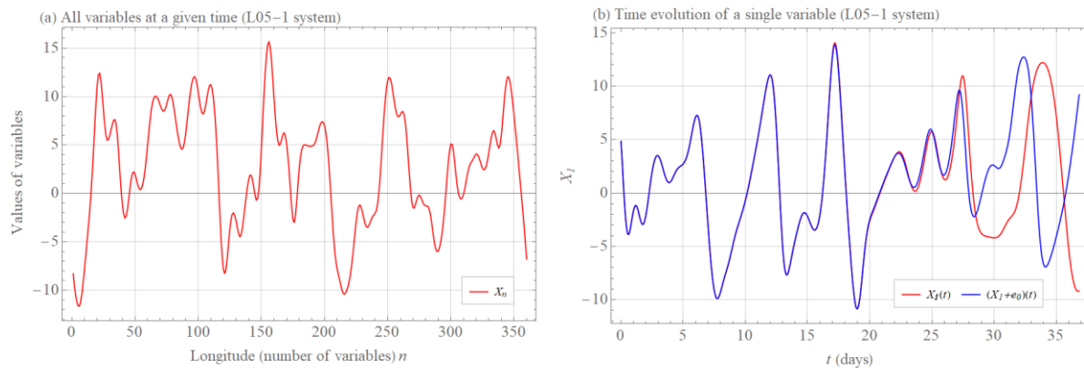
810 Figure 1. (a) Values of X_n , n = 1, \dots, 360 variables (red curve) of the L05-1 system at a given time (see Appendix A for more information on the system and its settings). (b) The time evolution t of the variable X_1(t) (red curve) and the time evolution of the initially nearby trajectory (X_1(0) + e_0)(t) (blue curve) of the system L05-1, where e_0 = 0.01 .
