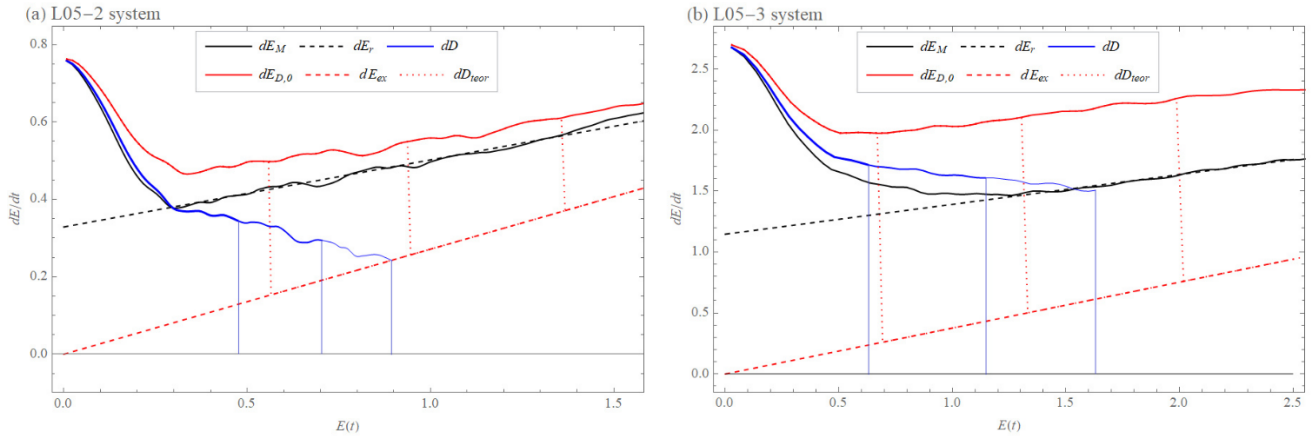
Figure 14. The validity of Eq. (23) ( dD/dt(D(t_k)) = dD/dt(E_{D,0}(t_k)) = \frac{dE_{D,0}}{dt}(E_{D,0}(t_k)) - \lambda \cdot E_{D,0}(t_k) ) is shown by vertical lines, where 930 the length of the blue ones is the same as the length of the red dotted dD_{teor} ones at times t_1 = 1 day, t_2 = 1.75 day, and t_3 = 2.5 day (from left to right) for (a) the difference between the L05-1 and L05-2 systems and at times t_1 = 0.3 day, t_2 = 0.6 day, and t_3 = 0.9 day (from left to right) for (b) difference between L05-1 and L05-3 systems, where dD = dD/dt(D) (Eq. (18), blue curve) is time difference of drift, dE_M = dE_M/dt(E_M) (Eq. (14), black curve) is model error growth, dE_{D,0} = dE_{D,0}/dt(E_{D,0}) is a hypothesis Eq. 935 dE_{r,L05-3} = 0.25 \cdot E + 1.15 ), and dE_{ex} (Eq. (1), red dashed line) is exponential growth with the value of \lambda determined from the quadratic hypothesis with model error dE_q (Eq. (6)) ( \lambda_{L05-2} \rightarrow dE_q = (0.27 \cdot E + 0.34)(1 - E/7.6) , and \lambda_{L05-3} \rightarrow dE_q = (0.38 \cdot E + 1.47)(1 - E/7.8) ).
