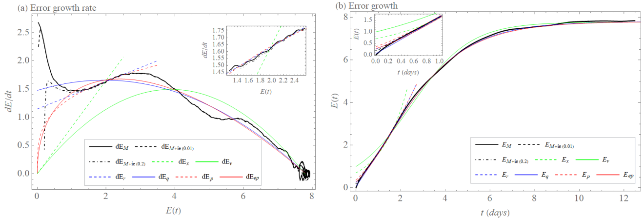
Figure 9. (a) Model error growth tendency (rate) dE/dt as a function of the error magnitude E ( dE_M , black), initial and model error growth tendency dE/dt as a function of the error magnitude E ( dE_{M+ie(0.01)} , black, dashed for E(0)=0.01 and dE_{M+ie(0.2)} , black, dot-dashed for E(0)=0.2 ), approximation of the early part of the model growth by exponential growth rate dE_{ex} (Eq. (1), green, dashed), exponential growth rate with model error dE_r (Eq. (5), blue, dashed), power law dE_p (Eq. (3), red, dashed) and approximation of the full curve by growth rate of quadratic hypothesis dE_{qu} (Eq. (2), green), growth rate of quadratic hypothesis with model error dE_q (Eq. (6), blue) and extended power law dE_{ep} (Eq. (4), red) for the L05-3 system as the "reality" and the L05-1 system as the "model." The inset shows the early phase. (b) Model error growth E as a function of time t ( E_M , Eq. (14), black), initial and model error growth E as a function of time t ( E_{M+ie(0.01)} , Eq. (15), black, dashed for E(0)=0.01 and E_{M+ie(0.2)} , Eq. (15), black, dot-dashed for E(0)=0.2 ), approximation of the early part of the growth by integration of dE_{ex} ( E_x , green, dashed) with \lambda_{ex}=0.83 1/day, integration of dE_r ( E_r , blue, dashed) with \lambda_r=0.25 1/day and \beta_r=1.15 unit/day, integrations of dE_p ( E_p , red, dashed) with a=1.35 unit 0.72 /day and b=0.72 and approximation of the full curve by integration of dE_{qv} ( E_{qv} , green) with \lambda_{qv}=0.77 1/day and E_{lim}=7.8 unit, integration of dE_q ( E_q , blue) with \lambda_q=0.38 1/day, \beta_q=1.47 unit/day and E_{lim}=7.8 unit and integration of dE_{ep} ( E_{ep} , red) with a=1.64 unit 0.55 /day, b=0.55 and E_{lim}=7.8 unit for the L05-3 system as the "reality" and the L05-1 system as the "model." The inset shows the early phase of the time evolution.
