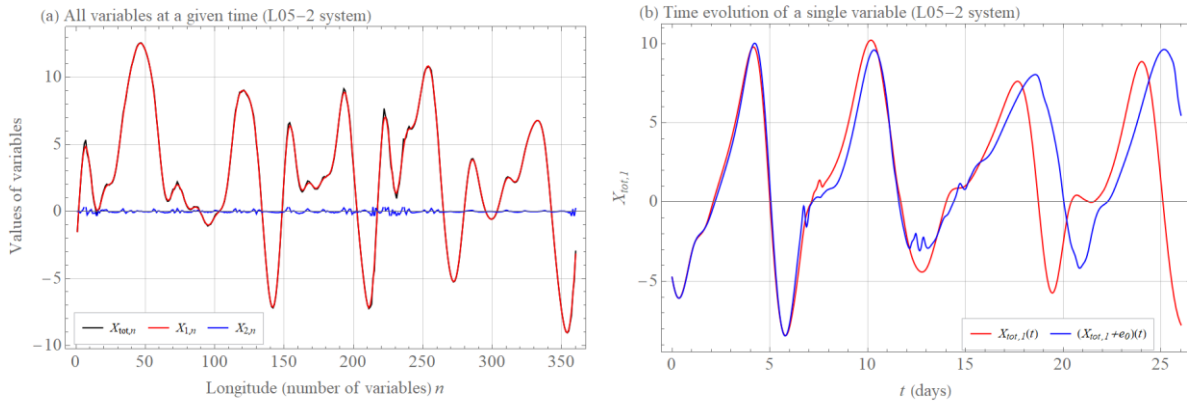
815 Figure 2. (a) Values of X_{1,n} (large scale, red curve), X_{2,n} (small scale, blue curve), X_{tot,n} (overall curve, black curve), n = 1, \dots, 360 variables of the L05-2 system at a given time (see Appendix A for more information on the system and its settings). (b) The time evolution t of the variable X_{tot,1}(t) (red curve) and the time evolution of the initially nearby trajectory (X_{tot,1}(0) + e_0)(t) (blue curve) of the system L05-2, where e_0 = 0.01 .
