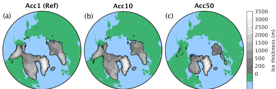
Figure 18. Simulated ice sheet extent and thickness at 115 ka for simulations with different climate acceleration factors: (a) reference run without climate acceleration, (b) acceleration factor 10 and (c) acceleration factor 50.
