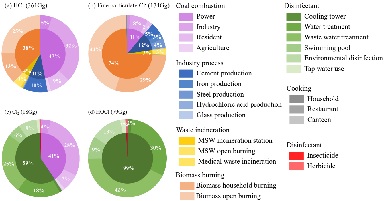
990 Figure 1 Contributions of different source categories to the anthropogenic emissions of HCl (a), fine particulate Cl - (b), Cl 2 (c), and HOCl (d) in 2019. The aggregation of 7 primary source categories from 41 specific sources can be found in Table S1.
