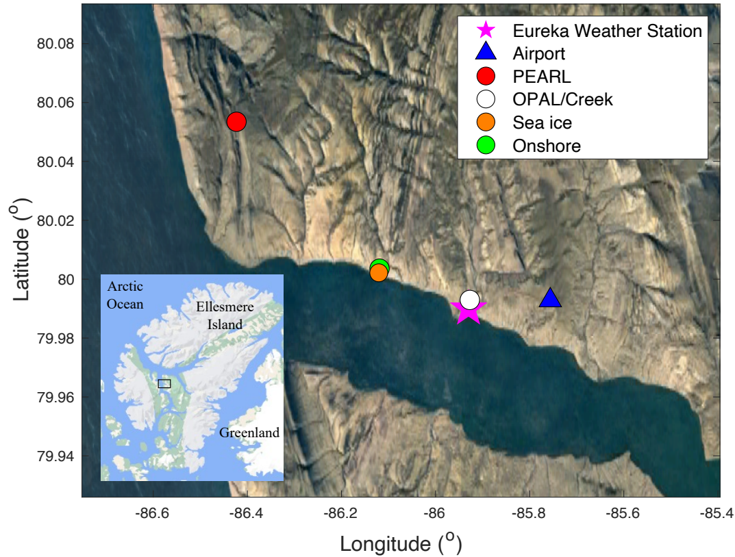
Figure 1. Local map with location of snow sampling sites marked by circles. The Eureka Weather Station (EWS) is marked by a star and the Eureka airport is marked by a triangle. The small inset box shows the location of the main map of Ellesmere Island, Canada. Image copyright: ©Google Earth/Google Maps.
