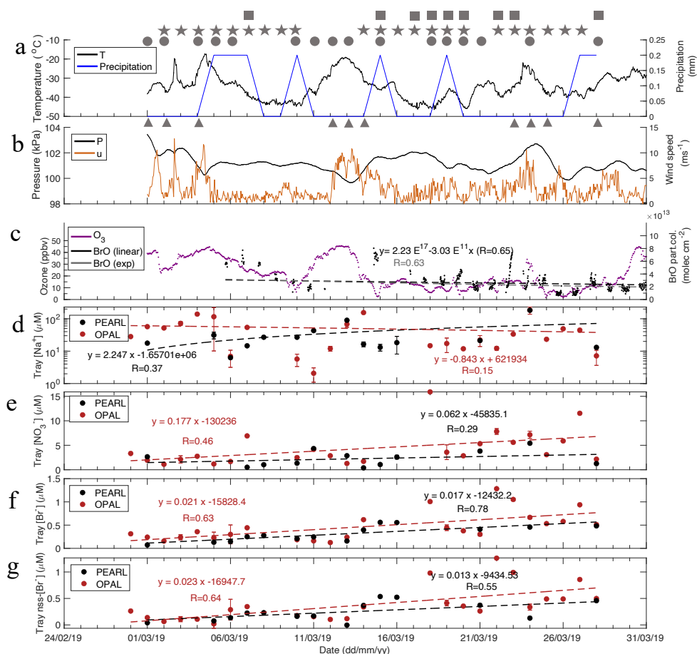
Figure 6. Same as Figure 5 but for 2019 snow time series. Note that the meteorology data are only from the Eureka Weather Station and the ionic data are tray samples [\text{Na}^+] (d), [\text{NO}_3^-] (e), [\text{Br}^-] (f), and non-sea-salt (nss) [\text{Br}^-] (g). Table S5 gives more statistical details of the linear regressions in each panel. Local weather conditions are marked by symbols in panels a and b. Squares represent fog, stars represent ice crystals, circles represent trace precipitation, and triangles represent blowing snow.
