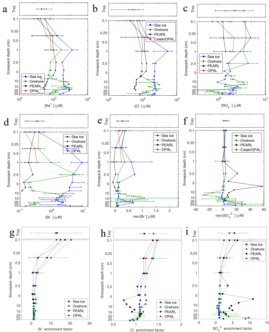
Figure 4. Vertical profiles of 2019 snow ions [\text{Na}^+] (a), [\text{Cl}^-] (b), [\text{NO}_3^-] (c), [\text{Br}^-] (d), non-sea-salt (nss)[ \text{Br}^- ] (e), nss[ \text{SO}_4^{2-} ] (f) and enrichment factor of [\text{Br}^-] (g), [\text{Cl}^-] (h) and [\text{SO}_4^{2-}] (i) (see Section 3.2 for details).
