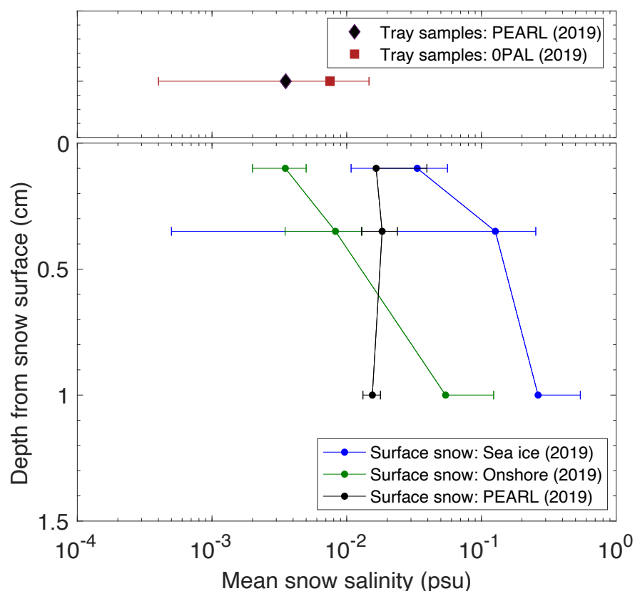
985 Figure 3. Mean snow salinity from the top 1.5 cm in three sub-layers: 0–0.2 cm, 0.2–0.5 cm, and 0.5–1.5 cm at the Sea ice, Onshore, and PEARL sites (lower panel), and tray sample salinity at the OPAL and PEARL sites (upper panel). The horizontal error bar represents one standard deviation. Note that tray samples at OPAL were from a mounted tray outside the OPAL building, approximately 1 m above the ground. Tray samples at PEARL were from a mounted tray (~1.5 m) on the roof of the PEARL Ridge Laboratory (~11 m above the ground).
