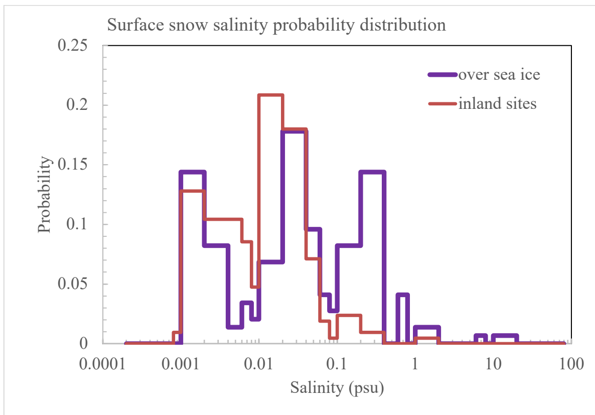
980 Figure 2. Eureka snow salinity probability distribution. The data include 2018 and 2019 snow sample measurements. The distribution over sea ice includes 146 snow samples, and the distribution at inland sites includes 211 snow samples (see Table 1).
