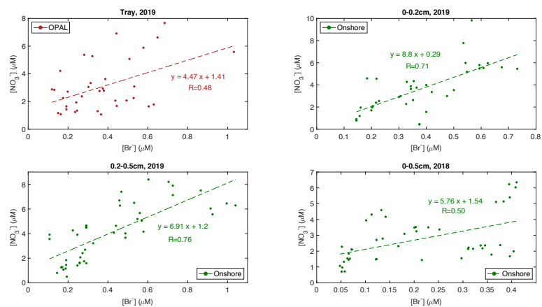
1100 Figure 9. Scatter plot of surface snow nitrate versus bromide in (a) tray samples (2019), (b) 0–0.2 cm layer (2019), (c) 0.2–0.5 cm layer (2019), and (d) 0–0.5 cm layer (2018). Linear regressions and corresponding correlation coefficients R are given.
