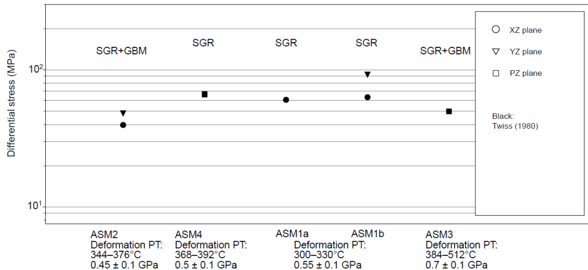
560 Figure 13: Differential stress for plane stress conditions estimated using piezometers by Twiss (1980). The vertical axis indicates differential stress. Stress estimated by microstructures formed by SGR+GBM is clearly lower than stress estimated by microstructures formed by SGR. Applied grain sizes were arithmetic mean and were calculated from the grain boundaries for Shimizu (2012).
