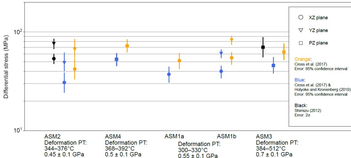
Figure 12: Differential stress for plane stress conditions estimated using piezometers based on recrystallized quartz grain size. The vertical axis indicates differential stress. Black points were calculated following Shimizu (2012), orange points were calculated following Cross et al. (2017), and blue points were calculated following Cross et al. (2017) using a correction for measured values by Griggs apparatus, which is proposed by Holyoke and Kronenberg (2010). Circle, triangle, and square points indicate measurements in the XZ, YZ, and PZ planes. The black, orange, and blue lines show uncertainties associated with differential stress associated with the black ( 2\sigma ), orange (95% confidence interval), and blue points (95% confidence interval).
