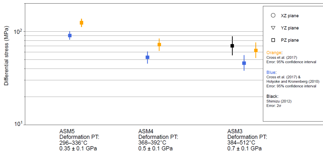
615 Figure 14: Differential stress for plane stress conditions estimated using piezometers based on recrystallized quartz grain size. The vertical axis indicates differential stress. Black points were calculated following Shimizu (2012), orange points were calculated following Cross et al. (2017), and blue points were calculated following Cross et al. (2017) using a correction for measured values by Griggs apparatus, which is proposed by Holyoke and Kronenberg (2010). Circle, triangle, and square points indicate measurements in the XZ, YZ, and PZ planes. The black, orange, and blue lines show uncertainties associated with differential stress associated with the black ( 2\sigma ), orange (95% confidence interval), and blue points (95% confidence interval).
