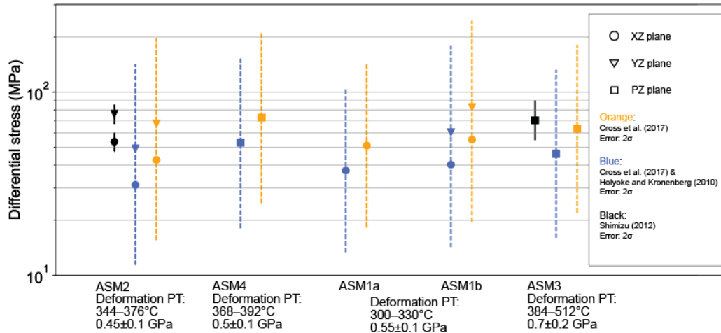
530 Figure 12: Differential stress for plane stress conditions estimated using piezometers based on recrystallized quartz grain size. The vertical axis indicates differential stress. Black points were calculated following Shimizu (2012), orange points were calculated following Cross et al. (2017), and blue points were calculated following Cross et al. (2017) using a correction for measured values by Griggs apparatus, which is proposed by Holyoke and Kronenberg (2010). Circle, triangle, and square points indicate measurements in the XZ, YZ, and PZ planes. The black, orange, and blue lines show uncertainties associated with differential stress associated with the black ( 2\sigma ), orange ( 1\sigma ), and blue ( 1\sigma ) points
