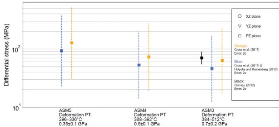
Figure 14: Differential stress for plane stress conditions estimated using piezometers based on recrystallized quartz grain size. The vertical axis indicates differential stress. Black points were calculated following Shimizu (2012), orange points were calculated following Cross et al. (2017), and blue points were calculated following Cross et al. (2017) using a correction for measured values by Griggs apparatus, which is proposed by Holyoke and Kronenberg (2010). Circle, triangle, and square points indicate measurements in the XZ, YZ, and PZ planes. The black, orange, and blue lines show uncertainties associated with differential stress associated with the black ( 2\sigma ), orange ( 1\sigma ), and blue ( 1\sigma ) points.
