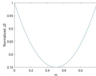
695 Figure B1: Value of J_2 normalized by max value. The horizontal axis indicates m in the above equation. 0.5: plane stress, 0 or 1: uniaxial.
