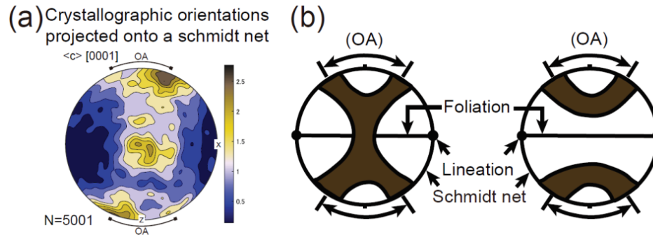
Figure 5: (a) Crystallographic orientations (c-axes) projected onto a Schmidt net (c-axis fabric pattern) (b) Definition of OA. The dark regions correspond to high concentrations of quartz c-axes plotted on the Schmidt net. The left figure shows crossed girdle and the right figure shows a small girdle.
