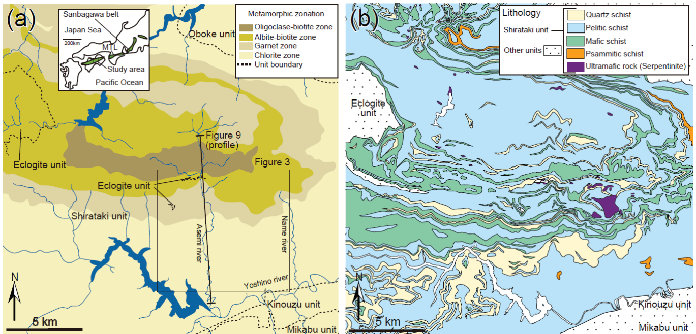
Figure 1: (a) Location, geological units, and metamorphic zonation map of the Sanbagawa metamorphic belt in central Shikoku (after Kouketsu et al., 2021; Aoya et al., 2013b; Endo et al., 2018; Higashino, 1990). (b) Geological map of the Shirataki unit (after Endo and Yokoyama, 2019; Hara et al., 2018).
