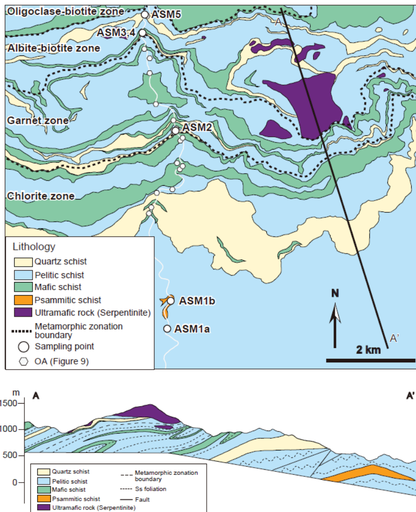
Figure 3: Geological map, cross-section, metamorphic zonation of study area, with sampling and data points (after Endo and Yokoyama, 2019).
