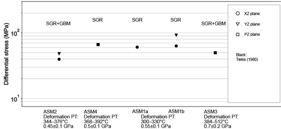
Figure 13: Differential stress for plane stress conditions estimated using piezometers by Twiss (1980). The vertical axis indicates differential stress. Stress estimated by microstructures formed by SGR+GBM is clearly lower than stress estimated by microstructures formed by SGR. Applied grain sizes were arithmetic mean and were calculated from the grain boundaries for Shimizu (2012).
