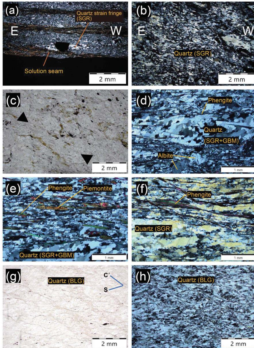
330 Figure 7: E and W indicate the eastern and western sides of the thin section. Except for (c) and (e), the up direction on the page corresponds to the up direction in the field. (a) Pelitic schist close to sample ASM1a. XZ plane. Crossed nicols. (b) Sample ASM1b. XZ plane. Crossed nicols. (c) Sample ASM2. XY plane. Opened nicols. Elongated phengite and quartz form weak lineation (arrow direction). (d) Sample ASM2 XZ plane. Crossed nicols. (e) Sample ASM3. PZ plane. Crossed nicols. (f) Sample ASM4. PZ plane. Crossed nicols. (g, h) Sample ASM5. PZ plane. (g) Opened nicols. (h) Crossed nicols.
