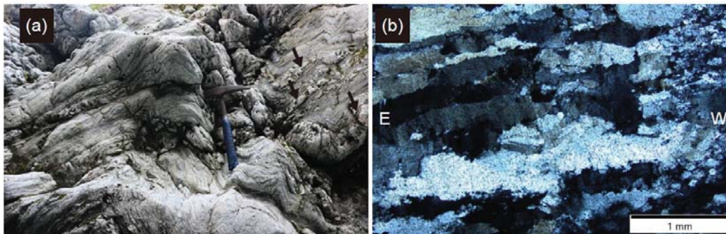
Fig. 6 (a) Outcrop photo showing foliation-subparallel veins (black arrows) in psammitic schist. Both foliation and veins were folded by later deformation (Du), but partly preserved unfolded structure, in which we collected sample ASM1b.
