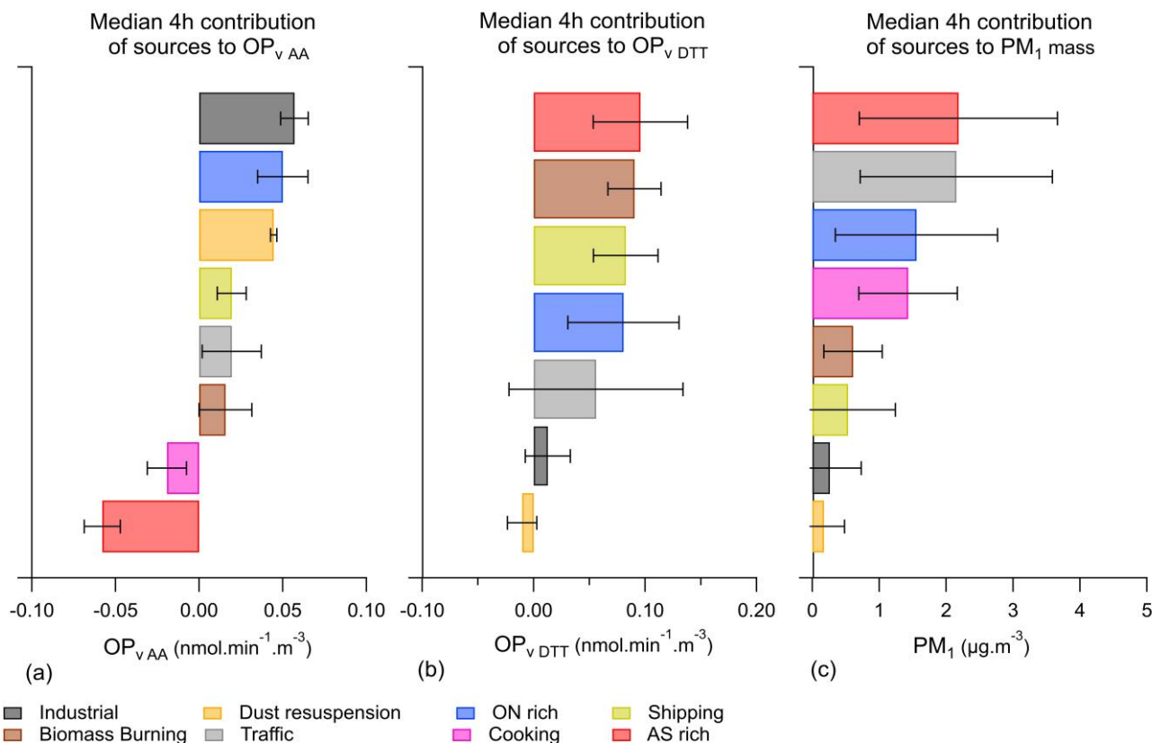
625 Figure 7. Median contribution of the sources identified by PMF_{PM1} over the OP sampling campaign without fireworks episode ( n = 78 samples) to (a) OP_{vAA} , (b) OP_{vDTT} , (c) PM_1 . Error bars represent the standard deviation of the data distribution.
