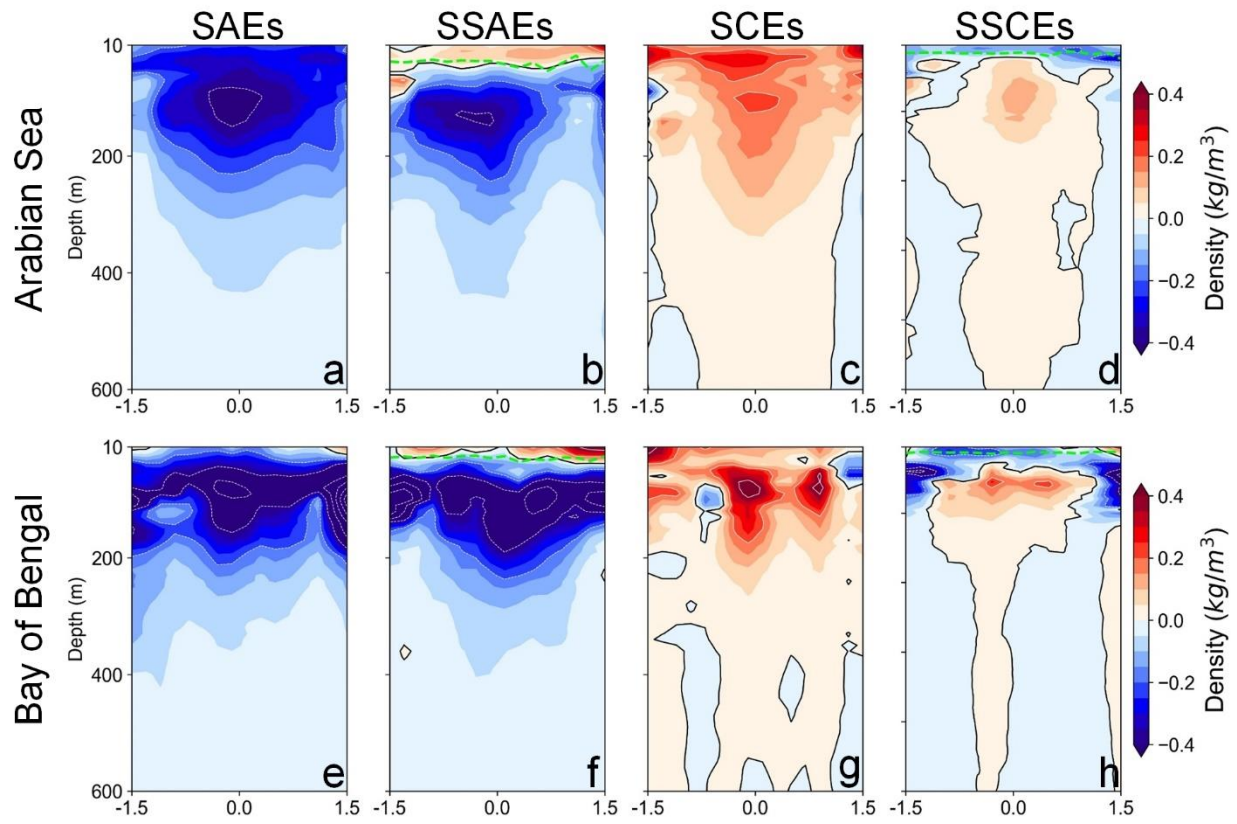
585 Figure 9. Composite zonal sections of the vertical potential density structure within SAEs, SSAEs, SCEs, and SSCEs in the AS (a-d) and the BoB (e-h) from 2000-2015. Black lines denote potential density in 0 \text{ kg/m}^3 . The lime dashed lines in SSAEs and SSCEs denote the MLD.
