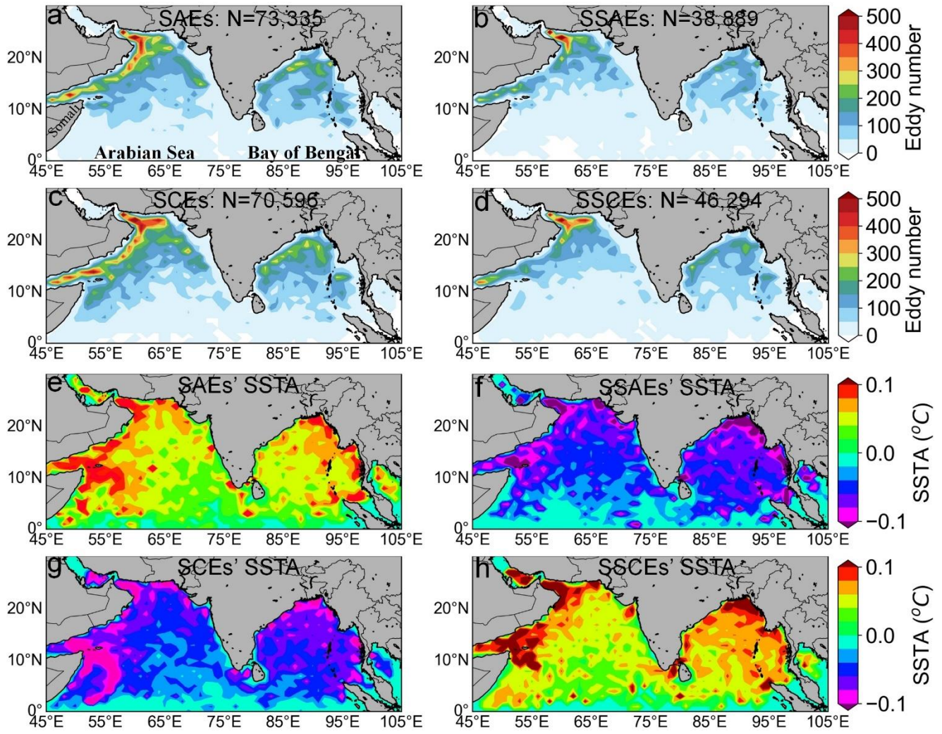
565 Figure 4. The spatial distribution of eddy concentration (a-d) and SSTA (e-h) within SAEs, SSAEs, SCEs, and SSCEs. N is the sum of eddies of the same kind observed in the NIO during 2000-2015.
