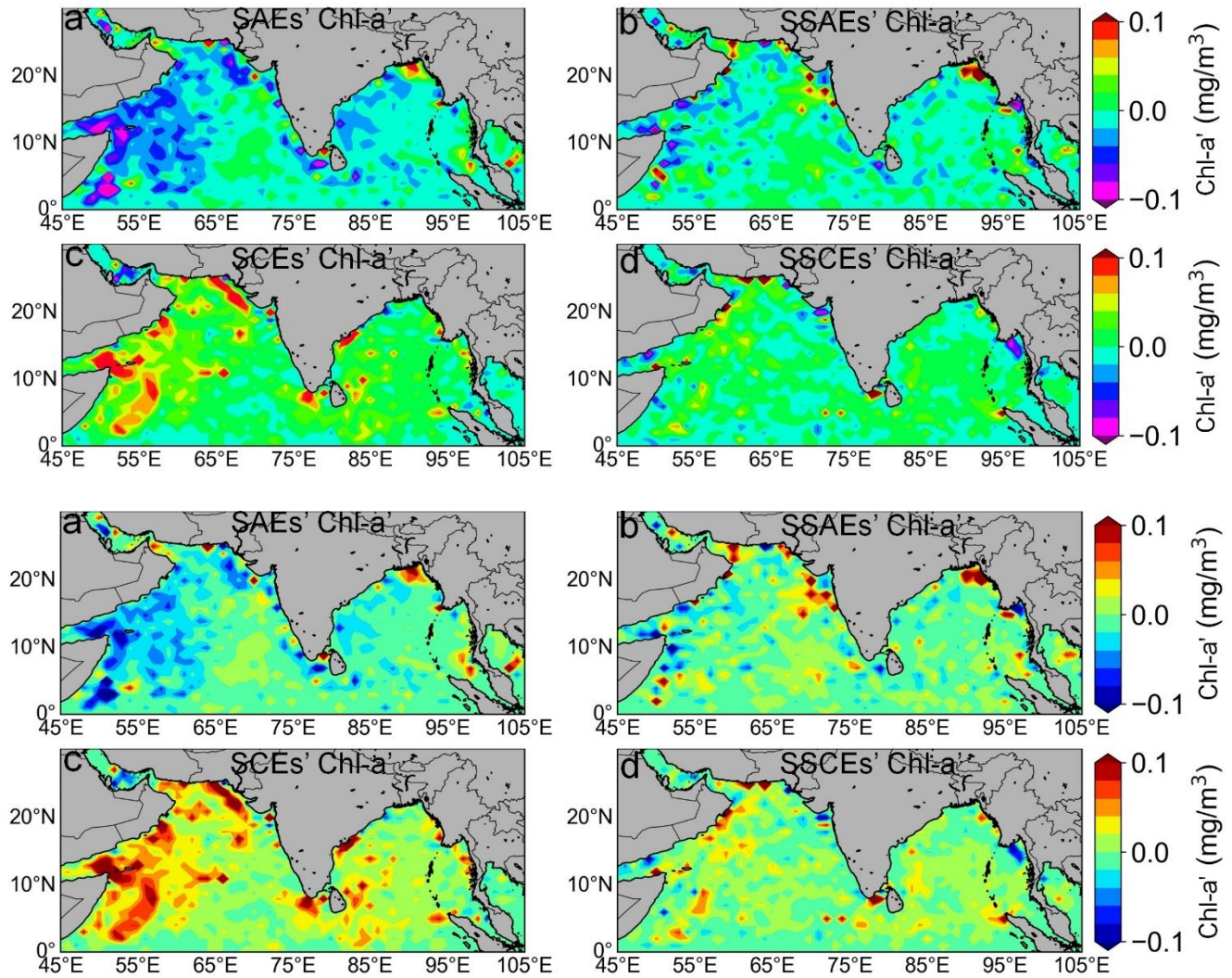
Figure 5. Spatial distribution of eddy-induced Chl-a' for SAEs (a), SSAEs (b), SCEs (c), and SSCEs (d) in the NIO during 2000-2015.
