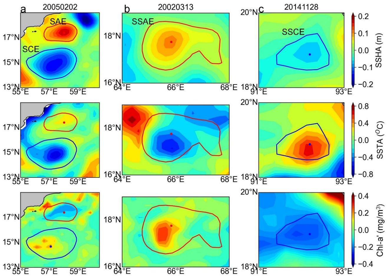
670 Figure 3. Case study of eddy imprints on SSHA, SSTA, and Chl-a' maps for an SAE and an SCE (a), an SSAE (b), and an SSCE (c). Red and blue lines denote eddy edges.
