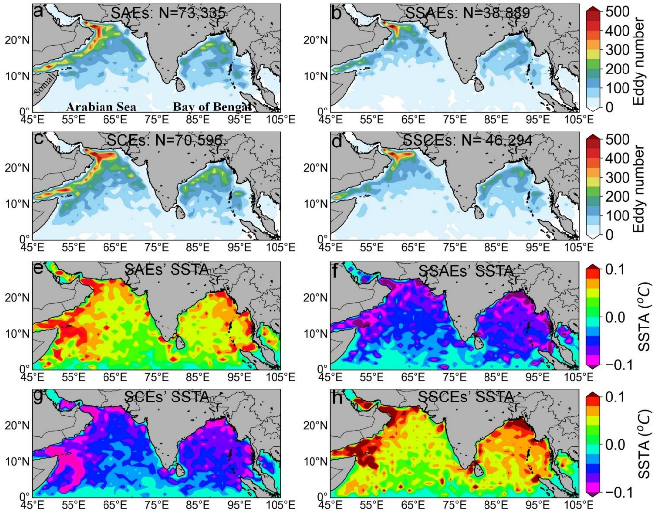
Figure 4. The spatial distribution of eddy concentration (a-d) and SSTA (e-h) within SAEs, SSAEs, SCEs, and SSCEs. N is the sum of eddies of the same kind observed in the NIO during 2000-2015.
