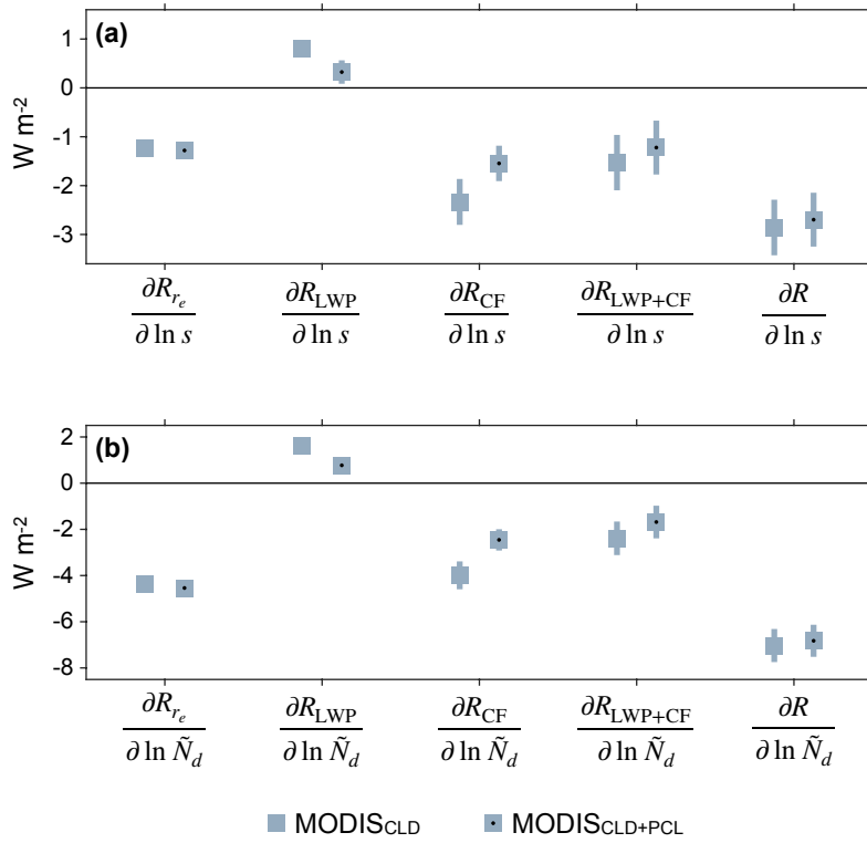
695 Figure 3. Spatial averages of the regression coefficients that represent aerosol indirect effects. Averages are computed over ocean between 55°S and 55°N. (a) Aerosol indirect effects estimated with s as the CCN indicator. \partial R_{LWP+CF}/\partial \ln s represents the total cloud adjustment ( R'_{LWP+CF} \equiv R'_{LWP} + R'_{CF} ). The MODIS CLD case is computed with only fully cloud- covered pixels included in the cloud histograms, and the MODIS CLD+PCL case is computed with both fully and partly cloud- covered pixels included. (b) Similar to (a), except that \tilde{N}_d is the CCN indicator. Squares show mean values, and vertical lines 700 show 95% CIs.
