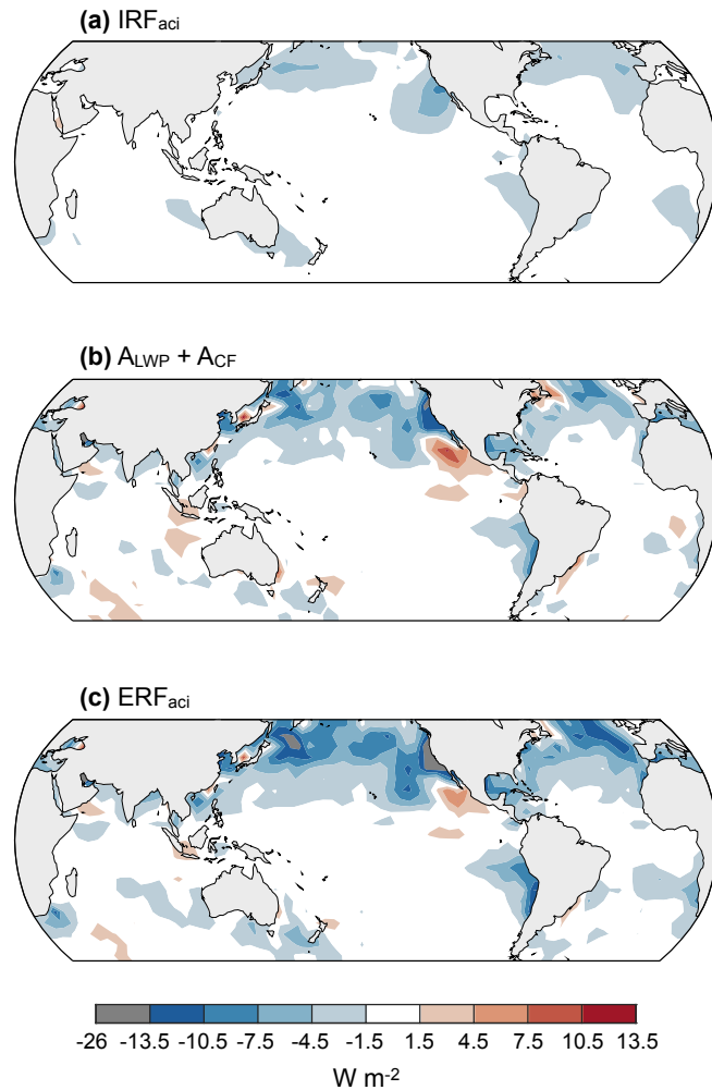
Figure 4. Components of historical ERF_{aci} from liquid clouds, including (a) the Twomey effect ( IRF_{aci} ), (b) the total cloud adjustment ( A_{LWP} + A_{CF} ), and (c) the overall ERF_{aci} . The estimates represent SW forcing, and they are computed with only fully cloud-covered pixels included in the cloud histograms ( MODIS_{CLD} ).
