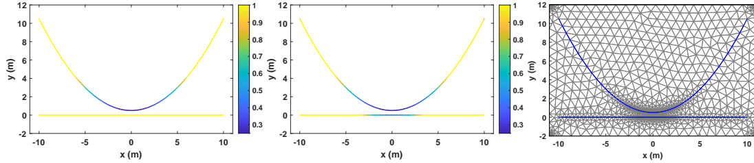
Figure 12. Example of 2D gradient limiting on internal constraints. Target mesh size without and with gradient limiting ( left and center , respectively), and the 2D mesh generated with given internal constraint ( right ).
