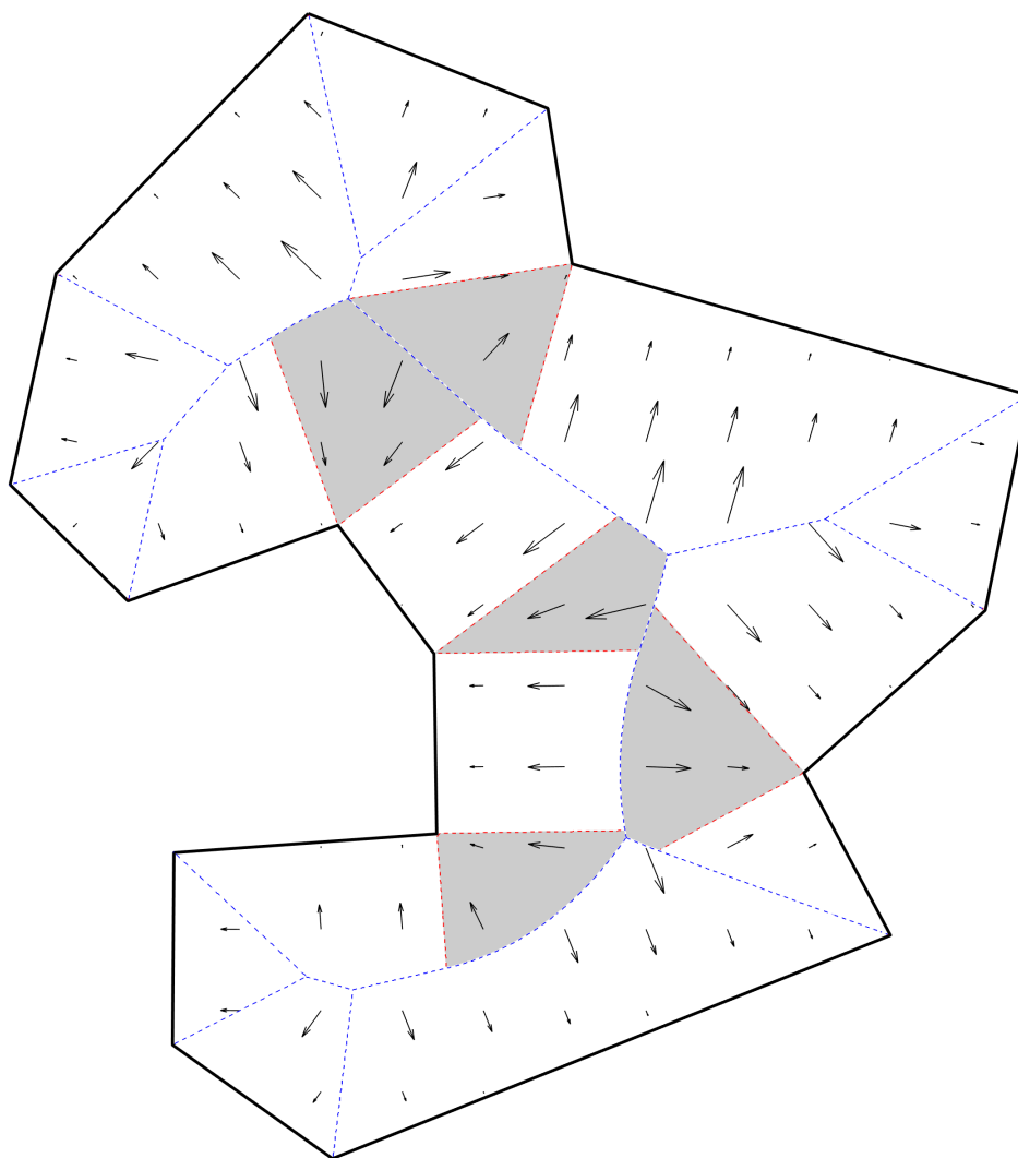
Figure A2. Voronoi polygons of a simple polygon, where boundaries of Voronoi polygons are shown as dashed lines ( blue lines are the medial axis (a subset of the Voronoi edges) and red dashed lines are Voronoi edges which are not part of the medial axis). The vector distance transform is shown by black arrows (scaled for visualization purpose). White and gray polygons indicate lateral and wedge type Voronoi polygons, respectively.
