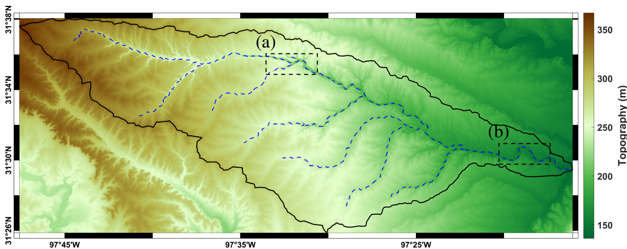
Figure 15. Domain of Middle Bosque River watershed (boundary of domain ( black solid line ), open-channels extracted with TopoToolbox ( blue dashed lines ), and zoom boxes ( black dashed lines ).
