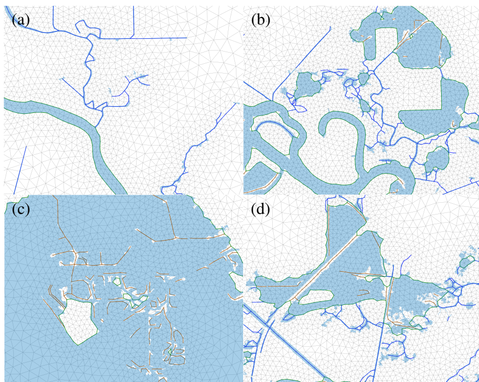
Figure 24. Zoom-in figures on corresponding boxes of Figure 23, where again channel centerlines are shown in blue , internal boundaries in brown , and shorelines in green .
