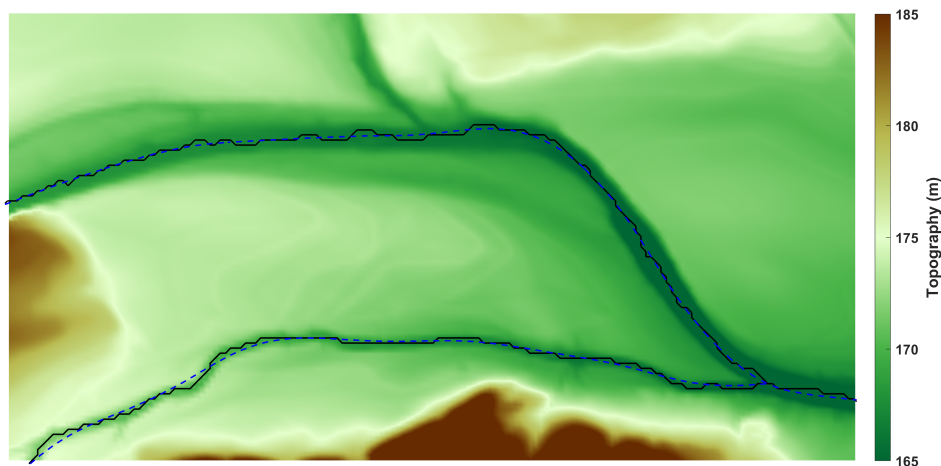
Figure 11. Example of extracted channel centerlines with TopoToolbox ( black solid line ) and smoothed line ( dashed blue line , with RMSE_{\text{desired}} = 10 m).
