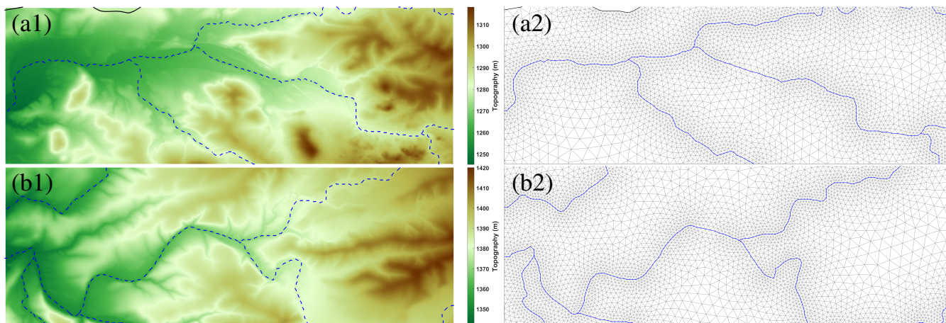
Figure 20. (a1,a2) Zoom-in figure on box (a) in Fig. 19 with open-channels (a1) and 2D mesh (a2). (b1,b2) Zoom-in figure on box (b) in Fig. 19 with open-channels (b1) and 2D mesh (b2).
