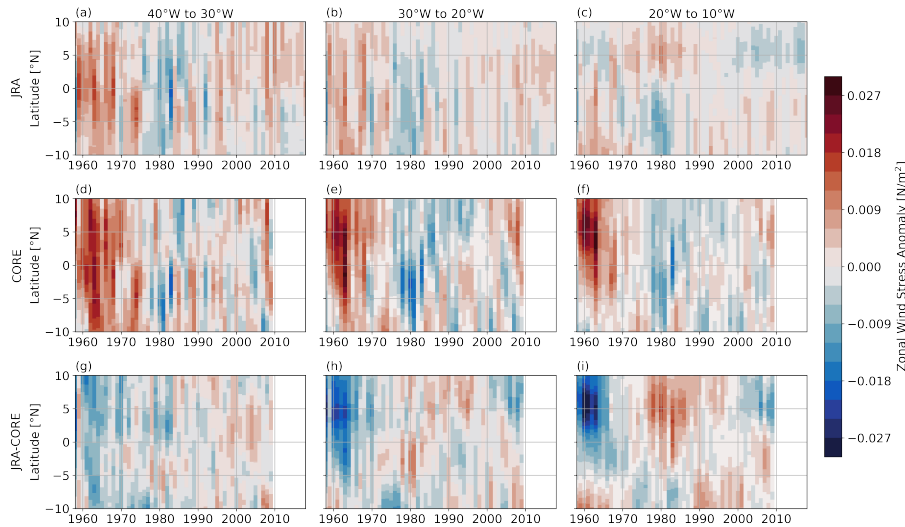
Figure 8. Hovmoeller diagram of annual mean zonal wind stress anomalies zonally averaged between 40°W and 30°W (left), 30°W and 20°W (centre) and 20°W and 10°W (right) for JRA_{sim} (upper), CORE_{sim} (middle), and the difference JRA_{sim}-CORE_{sim} (lower). The anomalies are calculated by removing the seasonal cycle (1980-2009) from the monthly mean output before temporally averaging to annual resolution.
