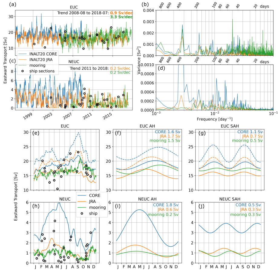
Figure 5. (a,c) Fixed box (EUC: 30m-300m, 1.2°S-1.2°N; NEUC: 60m-270m, 4.25°N-5.25°N) eastward transport time series (solid lines) and (b,d) power spectra of the EUC (a,b) and NEUC (c,d) calculated from CORE_{sim} (EUC: Jun 1996-Dec 2009, NEUC: Nov 2001-Dec 2009, blue lines), JRA_{sim} (EUC: Jun 2005-Dec 2018, NEUC: Nov 2010-Dec 2018, orange lines), moored observations (EUC: Jun 2005-Dec 2018, NEUC: Nov 2010-Dec 2018, green lines) and ship sections (black circles) at 23°W. (e,h) Seasonal cycle, (f,i) annual harmonic and (g,j) semi-annual harmonic of (e-g) EUC and (h-j) NEUC. Numbers in (f,g,i,j) represent the amplitude of the fitted harmonic cycle for each time series, respectively. The dashed lines in (e-g) show the results derived from eastward transports for the EUC calculated using Equ. 2 with a half mean width W of 3° ( CORE_{sim} : Jun 1996-Dec 2009, blue dashes lines, JRA_{sim} : Jun 2005-Dec 2018, orange dashes lines).
