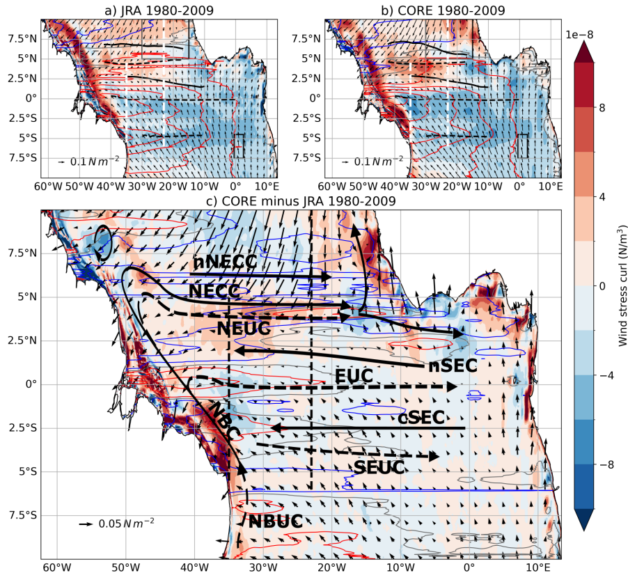
Figure 1. (a-c) 1980 to 2009 mean maps of wind stress (black arrows), wind stress curl (colour shading) and associated Sverdrup stream function (contour lines) calculated using (a) JRA_{sim} , (b) CORE_{sim} , (c) difference between the two forcings. Blue contour lines show negative, red contour lines positive values of Sverdrup stream function, zero line marked as grey contour. A negative stream function presents an anticlockwise rotation, this means that a zero-contour of the stream function with negative values in the south (north) marks maximum westward (eastward) velocities. In (a-b) the contour line interval is 2Sv , in (c) the \pm 1.5Sv , \pm 0.5Sv isolines are shown. Zonal black lines in (a,b) mark the mean latitude ( Y_{CM} , Equ. 1) of the simulated surface (solid) and subsurface (dashed) currents for the respective periods, meridional white dashed lines in (a-b) and black dashed lines in (c) mark 35^{\circ}W and 23^{\circ}W sections. The black rectangles in (a,b) mark the upwelling regions of the Guinea Dome in the northern and the Angola Dome in the southern hemisphere. (c) Superimposed in black are surface (solid) and thermocline (dashed) currents (adapted from Burmeister et al., 2019, based on observations): North Equatorial Countercurrent (NECC), northern branch of the NECC (nNECC), North Equatorial Undercurrent (NEUC), northern branch of the South Equatorial Current (nSEC) and central branch of the South Equatorial Current (cSEC), Equatorial Undercurrent (EUC), South Equatorial Undercurrent (SEUC), North Brazil Undercurrent (NBUC) and North Brazil Current (NBC).
