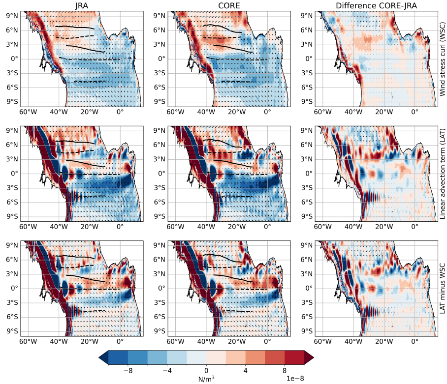
Figure A1. 1980 to 2009 mean maps of wind stress curl (WSC, colour shading, upper panel), wind stress (arrows), the linear advection term \beta\rho_0 \int_{H=500\text{m}}^0 vdz (LAT, colour shading, middle panel) and the difference of the two terms (colour shading, lower panel) calculated using JRA_{sim} (left), CORE_{sim} (centre), difference between the two forcings (right). Under Sverdrup balance LTA and WSC should be equal. Zonal black lines in mark the mean latitude ( Y_{CM} , Equ. 1) of the simulated surface (solid) and subsurface (dashed) currents for the respective periods.
