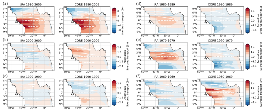
Figure 9. Sverdrup stream function calculated from (a) the 1980-2009 mean wind stress curl field, (b-f) annual mean wind stress curl anomalies averaged for the period (b) 2000-2009, (c) 1990-1999, (d) 1980-1989, (e) 1970-1979, (f) 1960-1969. In (b-f) we calculate first the Sverdrup stream function from the annual mean wind stress curl anomalies and average then over the respective periods. A negative stream function presents an anticlockwise rotation, this means that a zero-contour of the stream function with negative values in the south (north) marks maximum westward (eastward) velocities. Zonal white lines mark the mean latitude ( Y_{CM} , Equ. 1) of the simulated surface (solid) and subsurface (dashed) currents for the respective periods.
