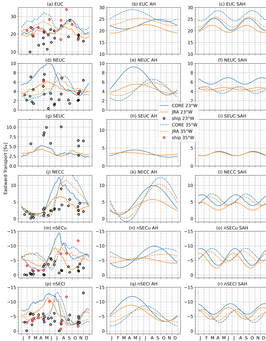
Figure 4. (left) Seasonal cycle, (middle) annual harmonic and (right) semi-annual harmonic fitted to the transport time series (Equ. 2) estimated from JRA_{sim} (orange lines), CORE_{sim} (blue lines) at 23^\circ W (solid lines) and 35^\circ W (dashed lines) averaged over the period 1980 to 2009. Black and red circles in the left column mark transports estimated from ship sections along 23^\circ W (black) and 35^\circ W (red).
