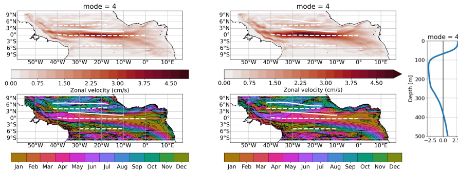
Figure 6. Amplitude (upper) and phase (lower) the fourth baroclinic mode, annual cycle of the zonal velocity from JRA_{sim} (left, 2000-2018) and CORE_{sim} (right, 1991-2009). To derive the 3D zonal velocity field associated with the specific baroclinic mode, the amplitudes must be multiplied by the corresponding vertical structure function shown on the right. The phase is given in month of the year when maximum eastward velocity occurs at the surface. Zonal white lines mark the mean latitude ( Y_{CM} , Equ. 1) of the simulated surface (solid) and subsurface (dashed) currents for the respective periods.
