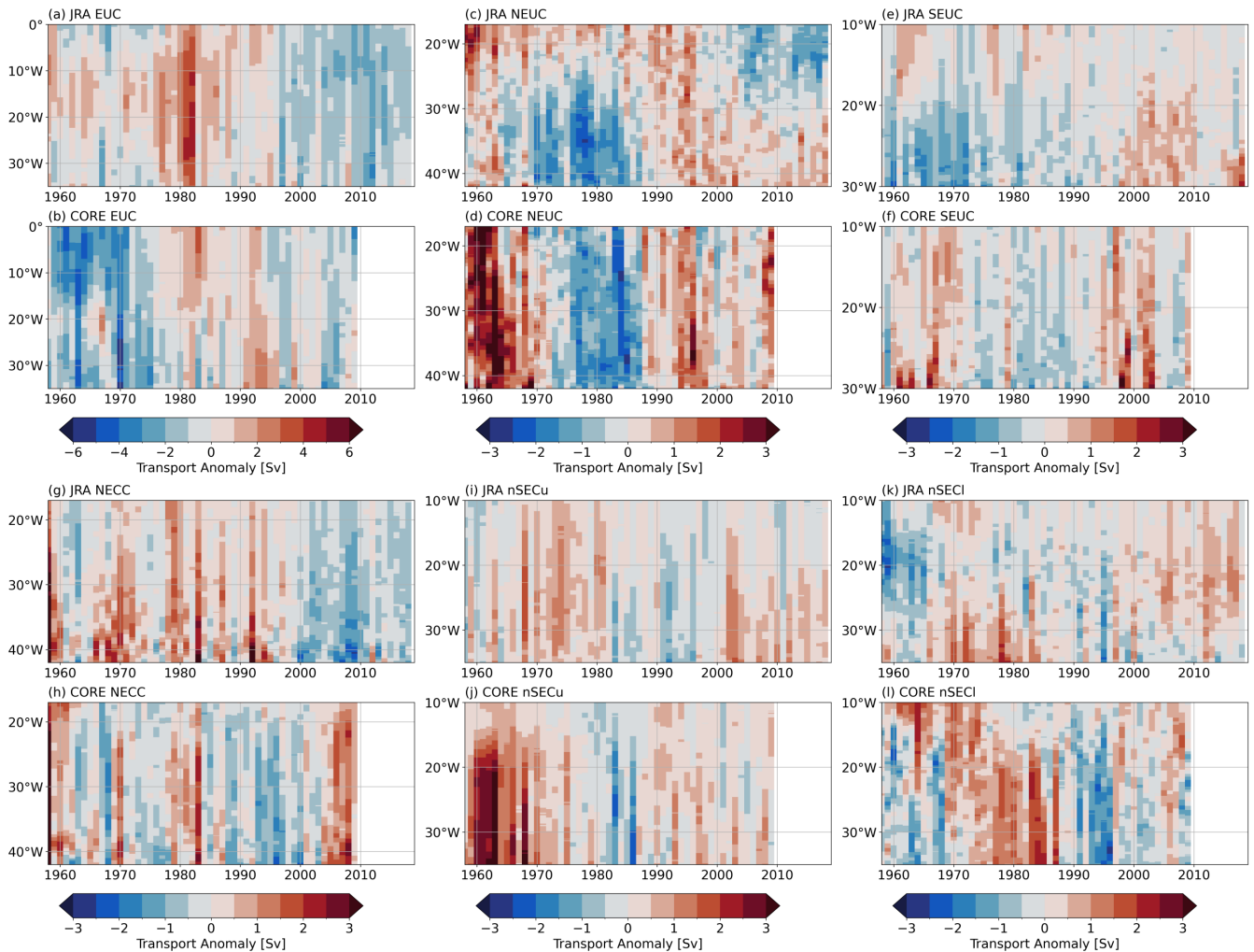
Figure 10. Hovmoller diagram of annual mean transport anomaly (Sv) for (a,b) EUC (eastward current), (c,d) NEUC (eastward current), (e,f) SEUC (eastward current), (g,h) NECC (eastward current), (i,j) nSECu (westward current) and (k,l) nSECI (westward current). The anomalies are calculated by removing the seasonal cycle (1980-2009) from the monthly mean output before temporally averaging to annual resolution.
