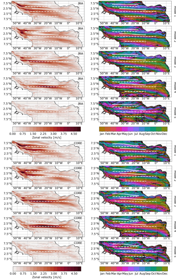
Figure A3. Amplitude (left) and phase (right) of first five baroclinic modes, annual cycle of zonal velocity from JRA_{sim} and CORE_{sim} (1980-2009). To derive the 3D zonal velocity field associated with the specific baroclinic mode, the amplitudes must be multiplied by the corresponding vertical structure function. The phase is given in month of the year when maximum eastward velocity occurs at the surface. Zonal white lines mark the mean latitude ( Y_{CM} , Eq. 2) of the simulated surface (solid) and subsurface (dashed) currents for the respective periods.
