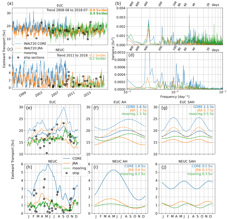
Figure 5. (a,c) Fixed box (EUC: 40m-300m, 1^{\circ}12'S - 1^{\circ}12'N ; NEUC: 60m-270m, 4.25^{\circ}N - 5.25^{\circ}N ) eastward transport time series (solid lines) and (b,d) power spectra of the EUC (a,b) and NEUC (c,d) calculated from CORE_{sim} (EUC: Jun 1996-Dec 2009, NEUC: Jun 2001-Dec 2009, blue lines), JRA_{sim} (EUC: Jun 2005-Dec 2018, NEUC: Nov 2010-Dec 2018, orange lines), moored observations (EUC: Jun 2005-Dec 2018, NEUC: Nov 2010-Dec 2018, green lines) and ship sections (black circles) at 23^{\circ}W . (e,h) Seasonal cycle, (f,i) annual harmonic and (g,j) semiannual harmonic of (e-g) EUC and (h-j) NEUC. Numbers in (f,g,i,j) represent the amplitude of the fitted harmonic cycle for each time series, respectively. The dashed lines in (e-g) show the results derived from eastward transports for the EUC calculated using Equ. 2 with a half mean width W of 3^{\circ} ( CORE_{sim} : Jun 1996-Dec 2009, blue line, JRA_{sim} : Jun 2005-Dec 2018, orange line).
