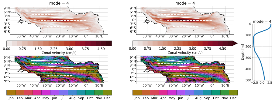
Figure 6. Amplitude (upper) and phase (lower) of fourth baroclinic mode, annual cycle of zonal velocity from JRA_{sim} (left, 2000-2018) and CORE_{sim} (right, 1991-2009) simulation. To derive the 3D zonal velocity field associated with the specific baroclinic mode, the amplitudes have to be multiplied by the corresponding vertical structure function shown on the right. The phase is given in month of the year when maximum eastward velocity occurs at the surface. Zonal white lines mark the mean latitude ( Y_{CM} , Equ. 1) of the simulated surface (solid) and subsurface (dashed) currents for the respective periods.
