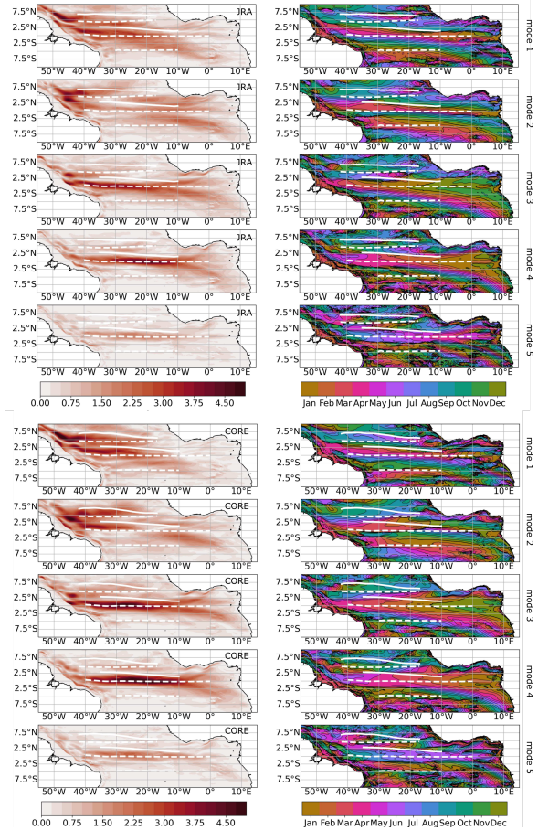
Figure A3. Amplitude (left) and phase (right) of first five baroclinic modes, annual cycle of zonal velocity-velocity from JRA and CORE (1980-2009) simulation. To derive the 3D zonal velocity field associated with the specific baroclinic mode, the amplitudes have to be multiplied by the corresponding vertical structure function. The phase is given in month of the year when maximum eastward velocity occurs at the surface. Zonal white lines mark the mean latitude ( Y_{CM} , Equ. 2) of the simulated surface (solid) and subsurface (dashed) currents for the respective periods.
