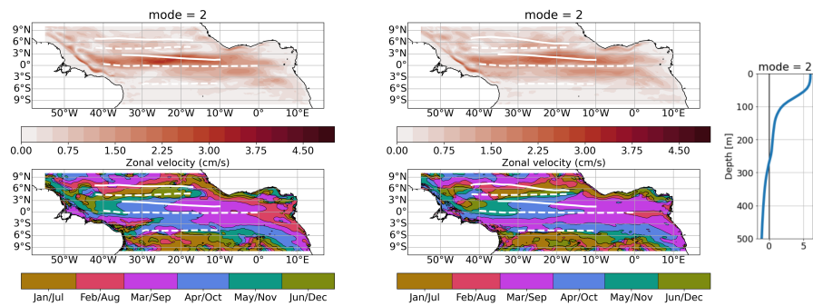
Figure A2. Amplitude (upper) and phase (lower) of second baroclinic mode, semiannual cycle of zonal velocity from JRA (left, 2000-2018) and CORE (right, 1991-2009) simulation. To derive the 3D zonal velocity field associated with the specific baroclinic mode, the amplitudes have to be multiplied by the corresponding vertical structure function shown on the right. The phase is given in month of the year when maximum eastward velocity occurs at the surface. Zonal white lines mark the mean latitude ( Y_{CM} , Equ. 2) of the simulated surface (solid) and subsurface (dashed) currents for the respective periods.
