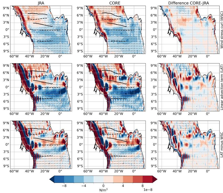
Figure A1. Amplitude–1980 to 2009 mean maps of wind stress curl (WSC, colour shading, upper panel) and phase–, wind stress (lower arrows) of second baroclinic mode, semi-annual cycle the linear advection term \beta \rho_0 \int_{H=500m}^0 v dz (LAT, colour shading, middle panel) and the difference of zonal velocity from both (colour shading, lower panel) calculated using JRA sim (left, 2000–2018) and CORE sim (right centre), 1991–2009 difference between both forcings (right) simulation. To derive the 3D zonal velocity field associated with the specific baroclinic mode, the amplitudes have to Under Sverdrup balance LTA and WSC should be multiplied by the corresponding vertical structure function shown on the right equal. The phase is given in month of the year when maximum eastward velocity occurs at the surface. Zonal white-black lines in mark the mean latitude ( Y_{CM} , Equ. 21) of the simulated surface (solid) and subsurface (dashed) currents for the respective periods.
