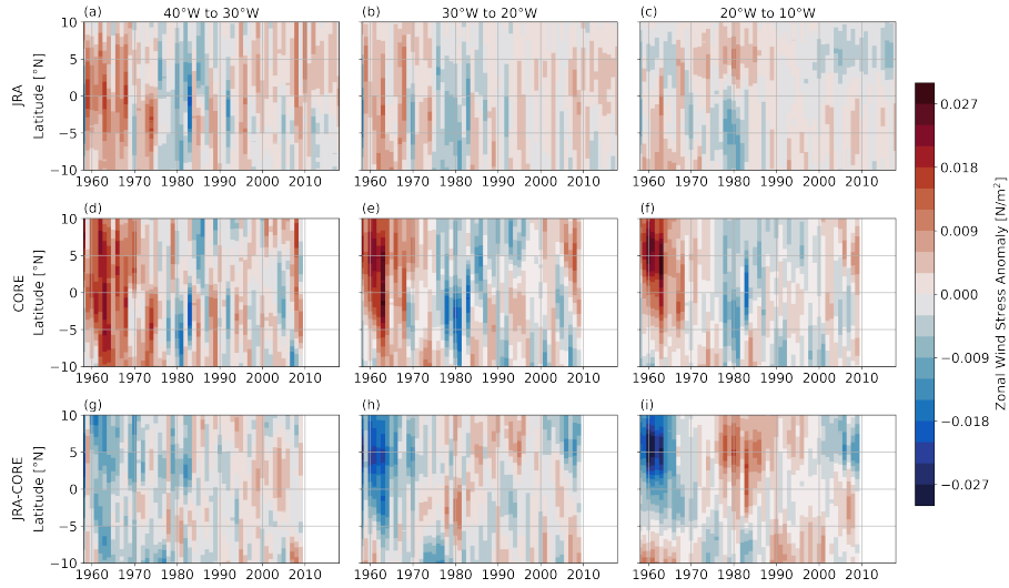
Figure 8. Hovmoeller diagram of annual mean zonal wind stress anomalies with respect to the seasonal cycle (1980-2009) zonally averaged between 40^{\circ}\text{W} and 30^{\circ}\text{W} (left), 30^{\circ}\text{W} and 20^{\circ}\text{W} (centre) and 20^{\circ}\text{W} and 10^{\circ}\text{W} (right) for \text{JRA}_{sim} (upper), \text{CORE}_{sim} (middle), and the difference \text{JRA}_{sim}-\text{CORE}_{sim} (lower).
