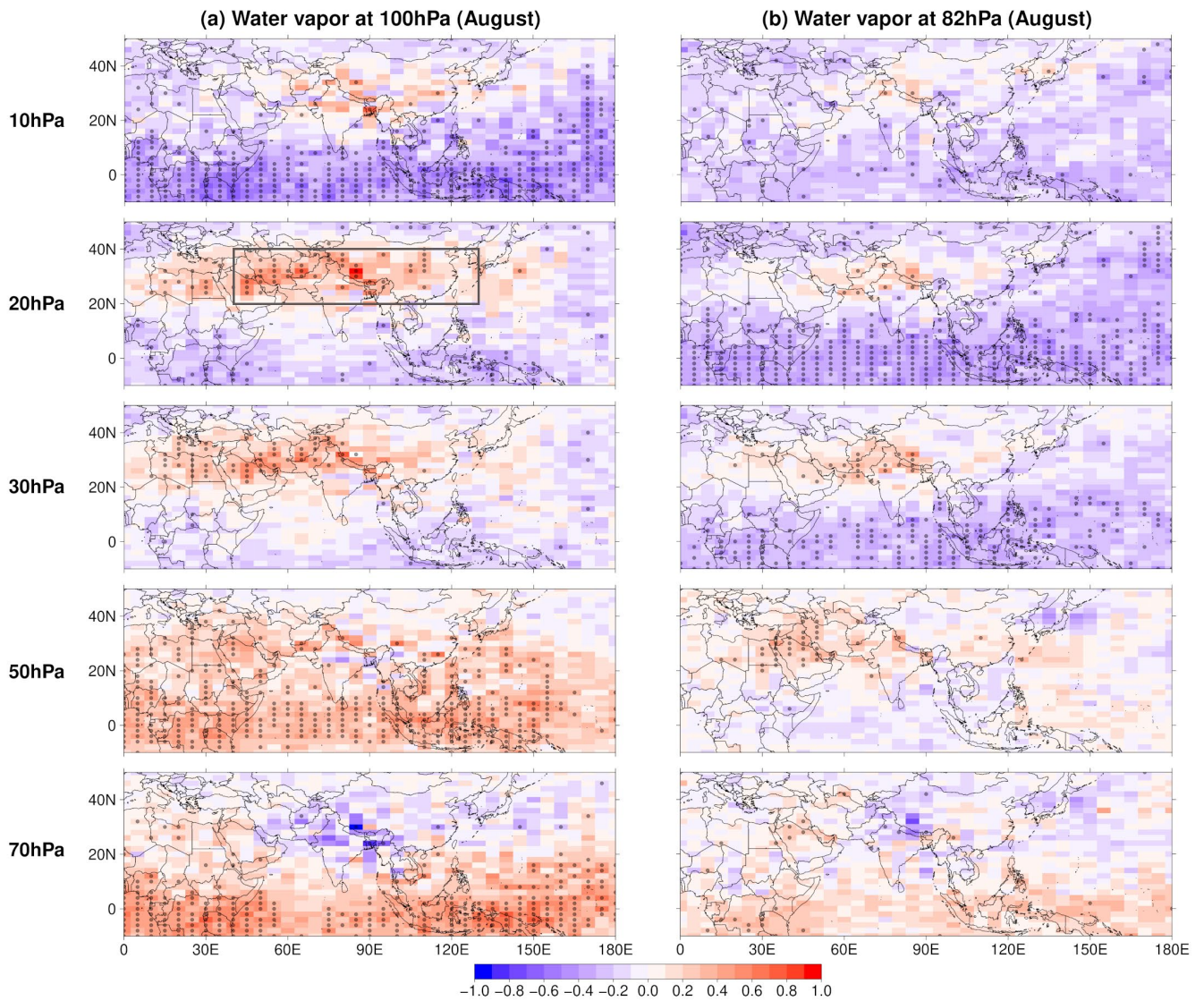
640 Figure A2: QBO-W minus QBO-E differences for MLS water vapour at 100hPa (a) and 82hPa (b) for August over the period 2005-2020. Each row corresponds to a different level at which the QBO phases were defined from 10hPa (top row) to 70hPa (bottom row). Dots indicate significance at the 95% confidence level. The region inside the grey box corresponds to the Asian monsoon region during the QBO phase in which we have identified a stronger signal on the water vapour of this area.
