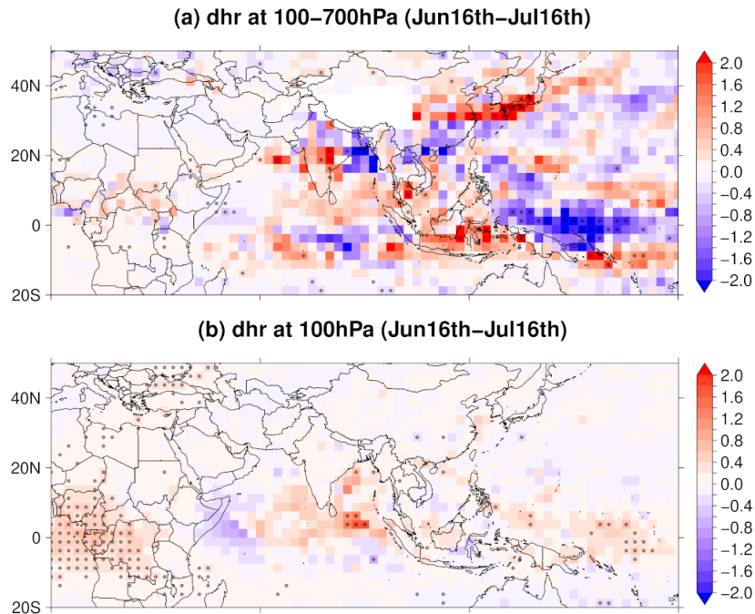
Figure 6: QBO-W minus QBO-E differences for diabatic heating rate in K/day (color shades) averaged between 100hPa and 700hPa (a) and at 100hPa (b) for the period 16th June - 16th July. Blue/red contour lines show negative/positive anomalies of the temperature eddy field with contour intervals at every 1K/day starting at 1K/day and -1K/day for positive and negative anomalies respectively. Dots indicate significance at the 95% confidence level.
