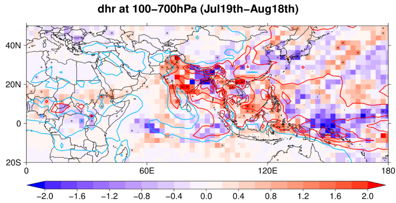
675 Figure A5: QBO-W minus QBO-E differences for diabatic heating rate (color shades) averaged between 100hPa and 700hPa over the period between 19th July and 18th August. Blue/red contour lines show negative/positive anomalies of the temperature eddy field with contour intervals at every 1K/day starting at 1K/day and -1K/day for positive and negative anomalies respectively. Dots indicate significance at the 95% confidence level.
