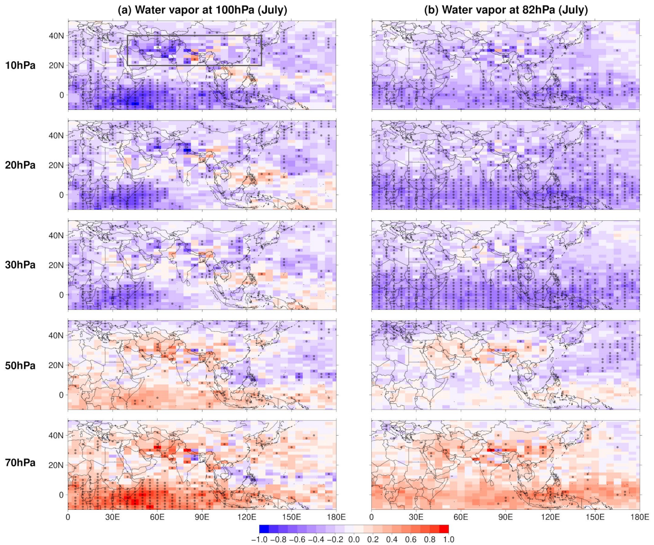
630 Figure A1: QBO-W minus QBO-E differences for MLS water vapour at 100hPa (a) and 82hPa (b) for July over the period 2005-2020. Each row corresponds to a different level at which the QBO phases were defined from 10hPa (top row) to 70hPa (bottom row). Dots indicate significance at the 95% confidence level. The region inside the grey box corresponds to the Asian monsoon region during the QBO phase in which we have identified a stronger signal on the water vapour of this area.
