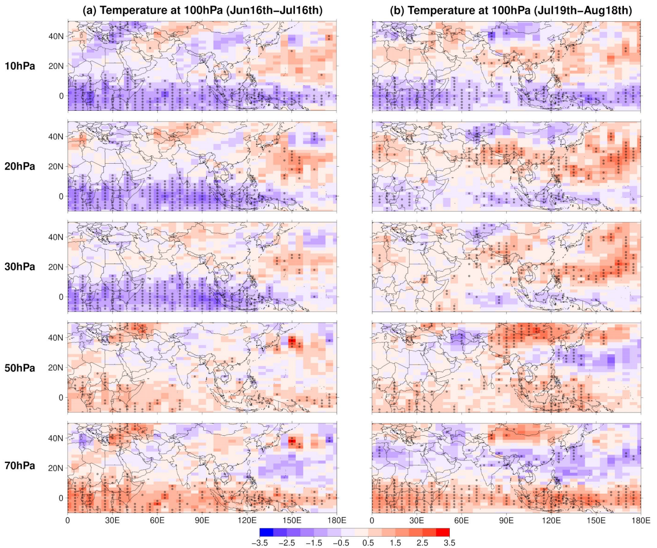
645 Figure A3: QBO-W minus QBO-E differences for MLS temperature at 100hPa averaged over the 31-day period between 16 June and 16 July (a) and between 19 July and 18 August (b), over 2005-2020. Each row corresponds to a different level at which the QBO phases were defined from 10hPa (top row) to 70hPa (bottom row). Dots indicate significance at the 95% confidence level.
