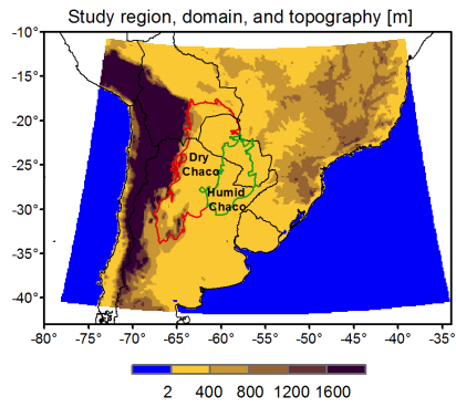
810 Figure 1: Model domain and topography. The coloured lines highlight the Gran Chaco subregions: Dry Chaco (red) and Humid Chaco (green).
