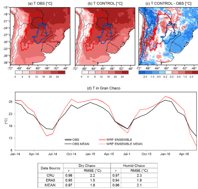
835 Figure 7: Time average of (a) the observed 2m temperature (mean between ERA5, CRU), (b) the CONTROL ensemble 2m temperature, and (c) their differences. (d) Temperature time series averaged over the Gran Chaco. The bands represent the dispersion among observational (grey) and ensemble members (pink), while the solid lines depict their respective means.
