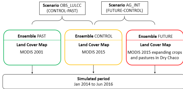
Figure 3: Experimental design.
