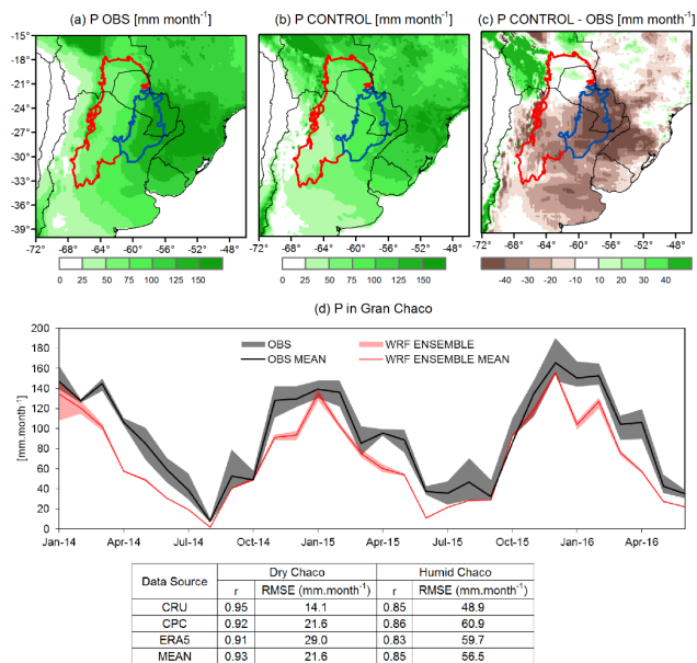
Figure 5: Time average of (a) the observed precipitation (mean between ERAS , CRU, and CPC), (b) the CONTROL ensemble precipitation, and (c) their differences. (d) Precipitation time series averaged in the Gran Chaco region. The bands represent the dispersion among observational (grey) and ensemble members (pink), while the solid lines depict their respective means.
