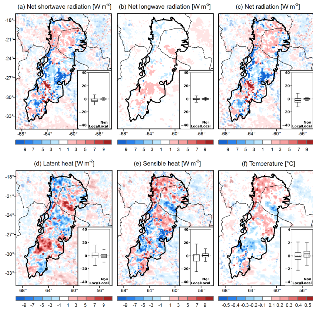
845 Figure 9: Differences in the summer energy budget components in the OBS_LULCC scenario (CONTROL-PAST): (a) net shortwave radiation, (b) net longwave radiation, (c) net radiation, (d) latent heat, (e) sensible heat, and (f) 2m temperature. Opacity was used to highlight the region of interest. The boxplots in the insets show the percentage differences of grid cells with land cover changes (Local) and without land cover changes in Dry Chaco (Non-Local).
