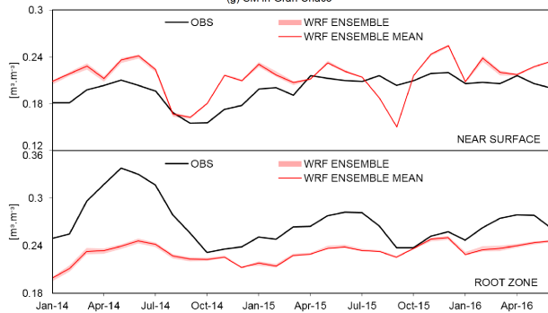
Figure 6: Time average of near-surface soil moisture for (a) the SMOPS product, (b) the CONTROL ensemble, (c) their differences, and time average of DJF root-zone soil moisture for (d) the HSAF product, (e) the CONTROL ensemble, and (f) their differences. (g) Observed and simulated soil moisture time series averaged over the Gran Chaco. The pink band represent the dispersion among ensemble members, while the solid red line depicts the respective mean.
