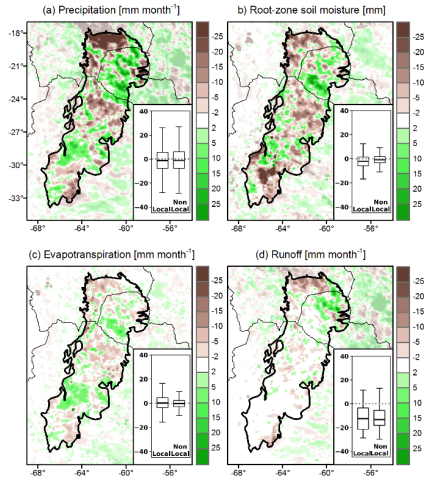
850 Figure 10: Differences in the summer water budget components in the OBS_LULCC scenario (CONTROL-PAST): (a) precipitation, (b) soil moisture, (c) evapotranspiration, and (d) runoff. Opacity was used to highlight the region of interest. The boxplots in the insets show the percentage differences of grid cells with land cover changes (Local) and without land cover changes in Dry Chaco (Non-Local).
