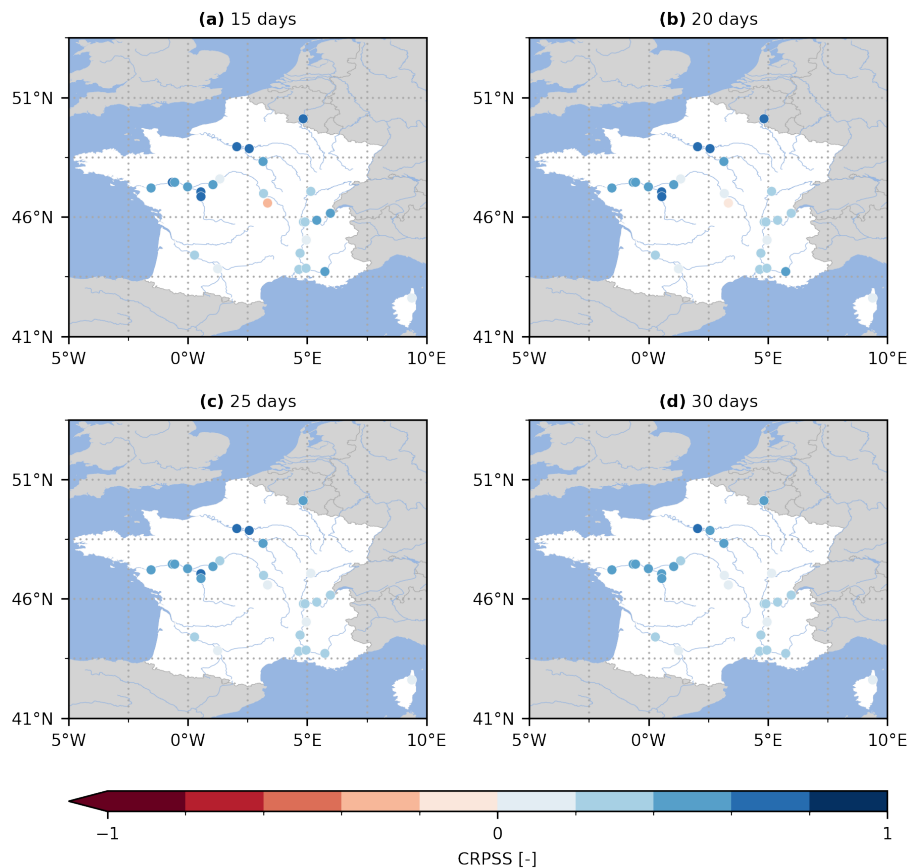
Figure 5. Continuous Rank Probability Skill Score (CRPSS) for the GloFAS reforecasts (v2.2) against the climatology benchmark. The CRPSS is computed with evalhyd for all 23 GloFAS stations located in France, and for four lead times (i.e. (a) 15 d, (b) 20 d, (c) 25 d, and (d) 30 d), mirroring a zoomed-in version of Figure 7 in Harrigan et al. (2023).
