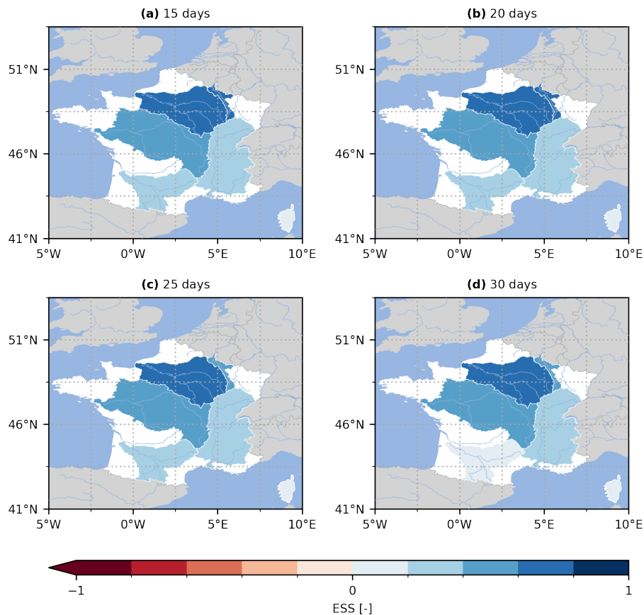
Figure 9. Energy Skill Score (ESS) for the GloFAS reforecasts (v2.2) against the persistence benchmark. The ESS is computed using the multi-dimensional design of evalhyd for six main French hydrographic basins (from North to South, Meuse, Seine, Loire, Rhône, Garonne, Corse), and for four lead times (i.e. (a) 15 d, (b) 20 d, (c) 25 d, and (d) 30 d).
