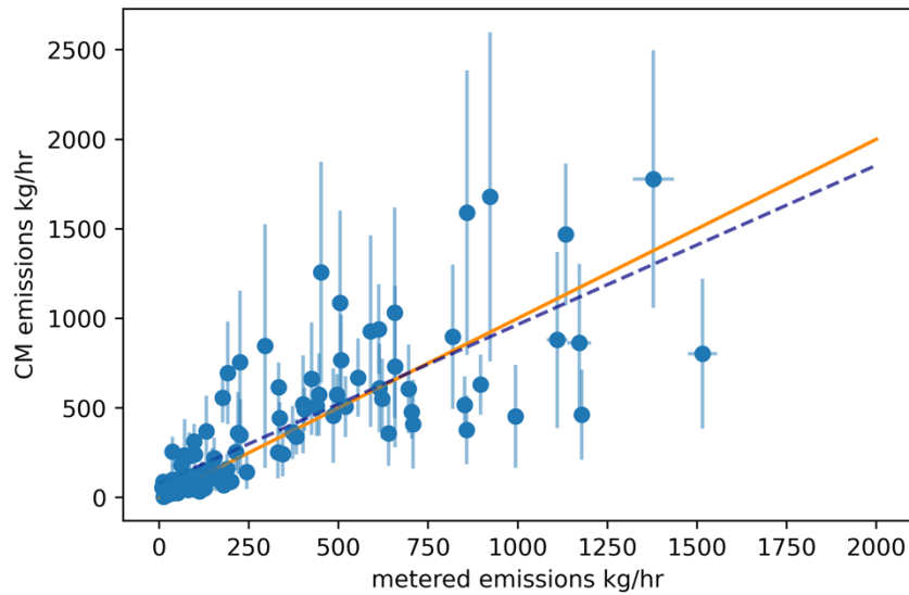
25 Figure S1: Metered emission rates versus the emission estimates for the 2022 controlled release using Duren e al 2019 methods. An OLS fit to CMF results in y = 0.89x + 77 with R^2 = 0.62 . For both figures the solid line represents the 1:1 line and the dashed line is the OLS fit.
