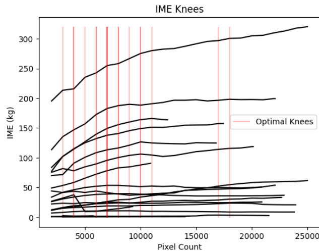
Figure S3: Pixel count versus the IME for all scenes used in the analysis as well as the optimal know for each scene (red).
