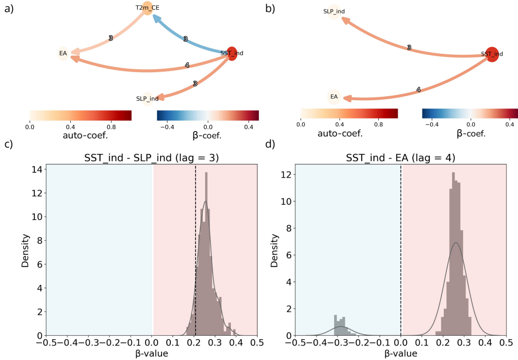
Figure 3. Causal Effect Network analysis for the late period (1958–2008) in ERA-20C. Causal graphs between a) SST index, EA teleconnection, SLP index and T2m CE and b) SST index, EA teleconnection and SLP index only. The strength and direction of the causal links is given by the \beta -coefficient and is represented by the arrows, whereas the auto-correlation path coefficient is represented for each variable by the respective circle colour. The numbers over each arrow represent the time lag (in months) when the strongest causal link between each variable pair is detected. c-d) Sensitivity of the causal links shown as the PDF of \beta -coefficients calculated for a random sample selection of 45 years, iterated 500 times, between the variables: SST and SLP indices at lag 3 (c), and SST index and EA at lag 4 (d). Only causal links with p-value < 0.1 are shown in (a) and (b). Red lines show the correspondent \beta -coefficients represented in (a).
