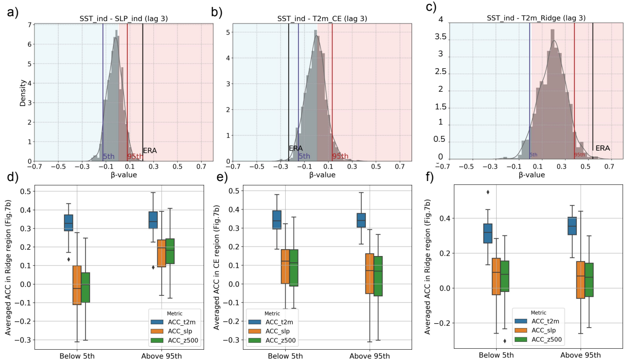
Figure 8. Influence of Spring (AM) SST Index on Summer (JA) Predictive Skill in MR-30. The upper row shows the sensitivity of causal link strength in MR-30 for a) \beta_{SST_{ind} \rightarrow SLP_{ind} | T2m_{CE}} , b) \beta_{SST_{ind} \rightarrow T2m_{CE} | SLP_{ind}} , and c) \beta_{SST_{ind} \rightarrow T2m_{Ridge} | SLP_{ind}} . Each distribution is generated from 1000 bootstrap samples, with a random selection of 45 years and one ensemble member from the 30-member set per year. The lower row compares the predictive skill of MR-30 against ERA-20C, highlighting time series that best match the observed causal link strength (above the 95th percentile for positive values, below the 5th percentile for negative values) versus those furthest from the observed strength (below the 5th percentile for positive links, above the 95th for negative links). Mean ACCs are shown for July-August sea level pressure (SLP), 2-metre air temperature (T2m), and 500 hPa geopotential height (Z500), averaged over the region highlighted by the grey box. Further details are provided in Sect.3.5.
