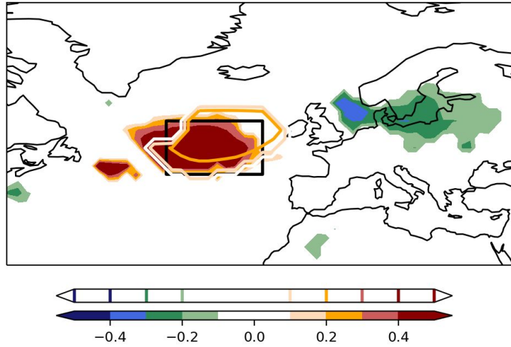
Figure A2. Causal map for 4-month lag, showing causal links between March-April SST index and July-August temperature in shading \beta_{\text{SST}_{\text{ind}} \rightarrow \text{T2m}|EA} and March-April SST index and July-August SLP \beta_{\text{SST}_{\text{ind}} \rightarrow \text{SLP}|EA} in contours. Black box highlights the region of strongest causal influence and represents the area used to calculate the T2m index denoted \text{T2m}_{\text{Ridge}} in the text.
