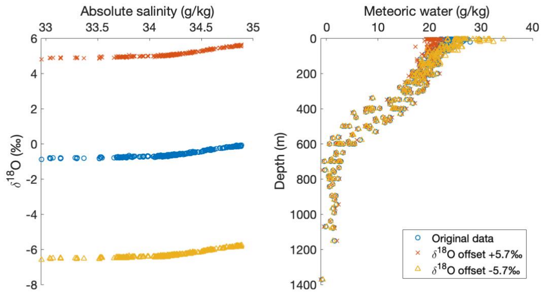
580 Figure A3: Impact on inter-lab offsets on calculated meteoric (glacial melt) water fraction for NBP20-02 data. The left panel shows the \delta^{18}\text{O} offset ( \pm 5.7\text{‰} ) necessary to significantly affect calculated meteoric water fractions, when using mCDW and meteoric water endmembers calculated from that data. The right panel shows the calculated meteoric water fractions produced using the original, and offset data. The calculated meteoric water fractions are impacted very little because two of the three endmembers (mCDW and meteoric water) are defined by the offset data.
