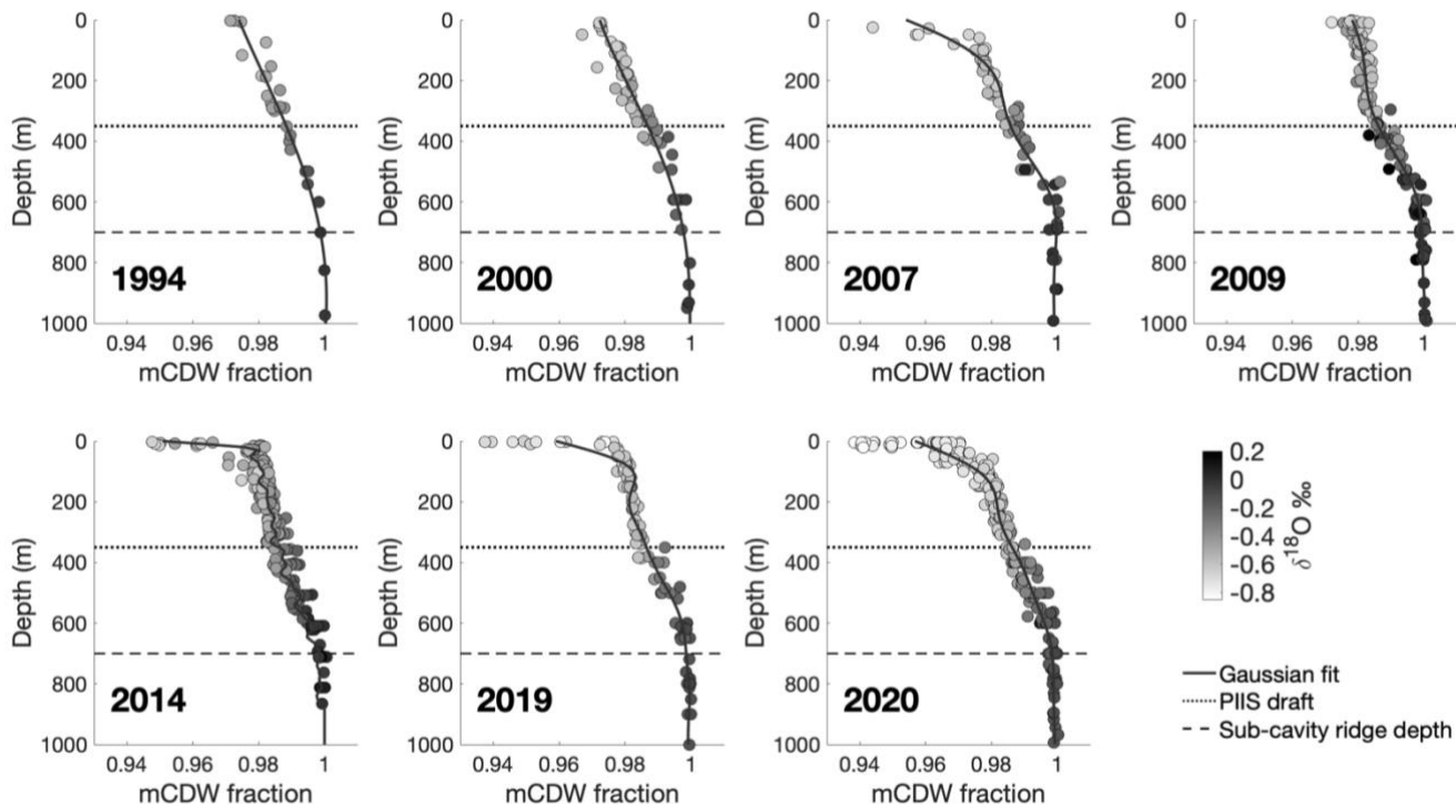
785 Figure A7: mCDW fractions vs depth. Calculated mCDW fractions using salinity and \delta^{18}\text{O} measurements in 3-endmember mixing model. Shading of dots indicates the measured \delta^{18}\text{O} of that sample. Deep waters (>800 m) characterize relatively unadulterated mCDW, while near surface waters contain the highest concentrations of sea ice melt and meteoric water. Dotted horizontal lines show the depth of the PIIS draft, and dashed lines show the depth of the PIIS sub-cavity ridge.
