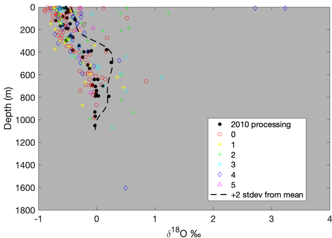
825 Figure A9: \delta^{18}\text{O} vs depth of all 2009 samples, coded by amount of precipitate present. Each bottle was graded by eye based on the volume of precipitate present with 0 being no precipitate present, and 5 being the most precipitate present. As with Figure A8 , the dashed line represents +2 standard deviations from the mean \delta^{18}\text{O} at each depth.
