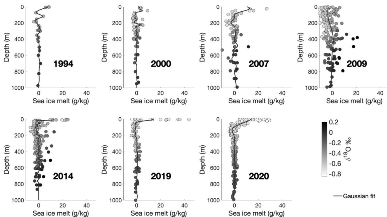
250 Figure 4: Sea ice melt fractions (g of sea ice melt per kg of seawater) vs depth. Shading shows \delta^{18}\text{O} value, and solid lines represent Gaussian Process regression fits. Sea ice melt fractions are highest at the surface. Negative sea ice melt fractions, occurring mostly below 100 m, are the product of earlier sea ice formation.
