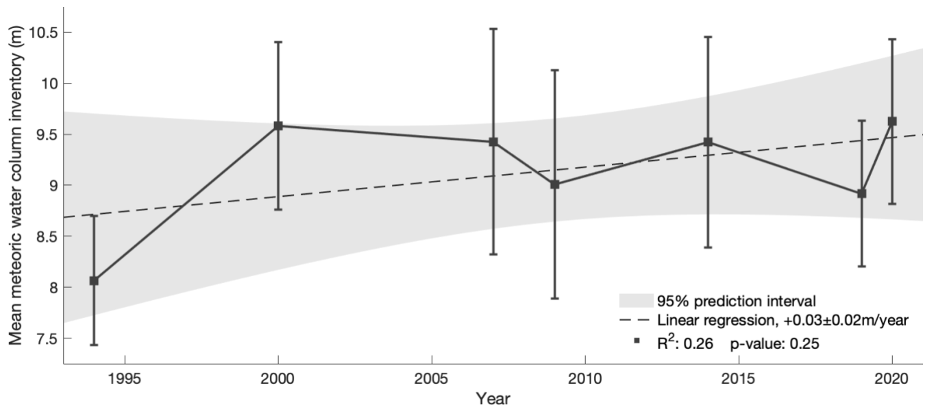
Figure 5: Average meteoric water column inventory. Depth-integrated meteoric water content from the Gaussian Process fit ( Figure 3 ) between the sea surface and 800 m. Error bars show the uncertainty ( Results 3.5 ) associated with data volume, analytical precision, and uncertainty in endmember values ( Data and Methods 2.2 ). A linear regression of the mean values shows an increase of 0.03 \pm 0.02 m/year (p-value 0.25). Grey shading shows the 95% prediction interval for the linear regression.
