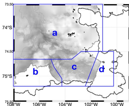
320 Figure 6: Boundaries of geographic groupings used for spatial sensitivity analysis. Blue lines show boundaries of geographic areas analyzed separately. Gray shading shows bathymetry, with isobaths drawn at 800 m. More detailed maps for each year are in Appendix A4.1.
