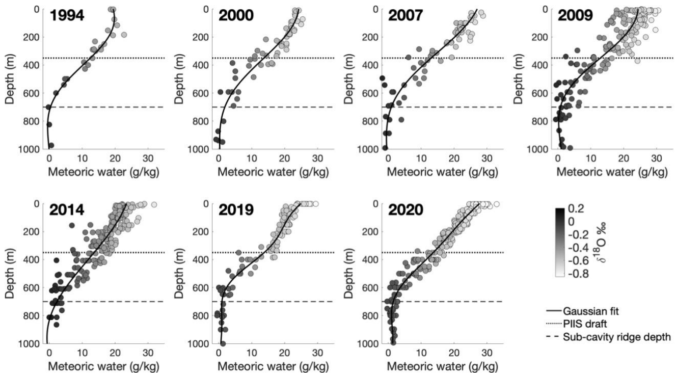
Figure 3: Meteoric water fractions (g of meteoric water per kg of seawater) vs depth. Shading shows \delta^{18}\text{O} value, and solid lines represent Gaussian Process regression fits. Dotted and dashed lines show the depth of the PIIS draft and sub-cavity ridge (Jenkins et al., 2010). Small false negative meteoric water fractions in deep waters are the result of sample salinity and/or \delta^{18}\text{O} values that are higher than the mCDW endmember value(s) ( Table 2; Data and Methods 2.2 ), the result of spatial variability in mCDW properties (discussed in further detail in Results 3.5 ).
