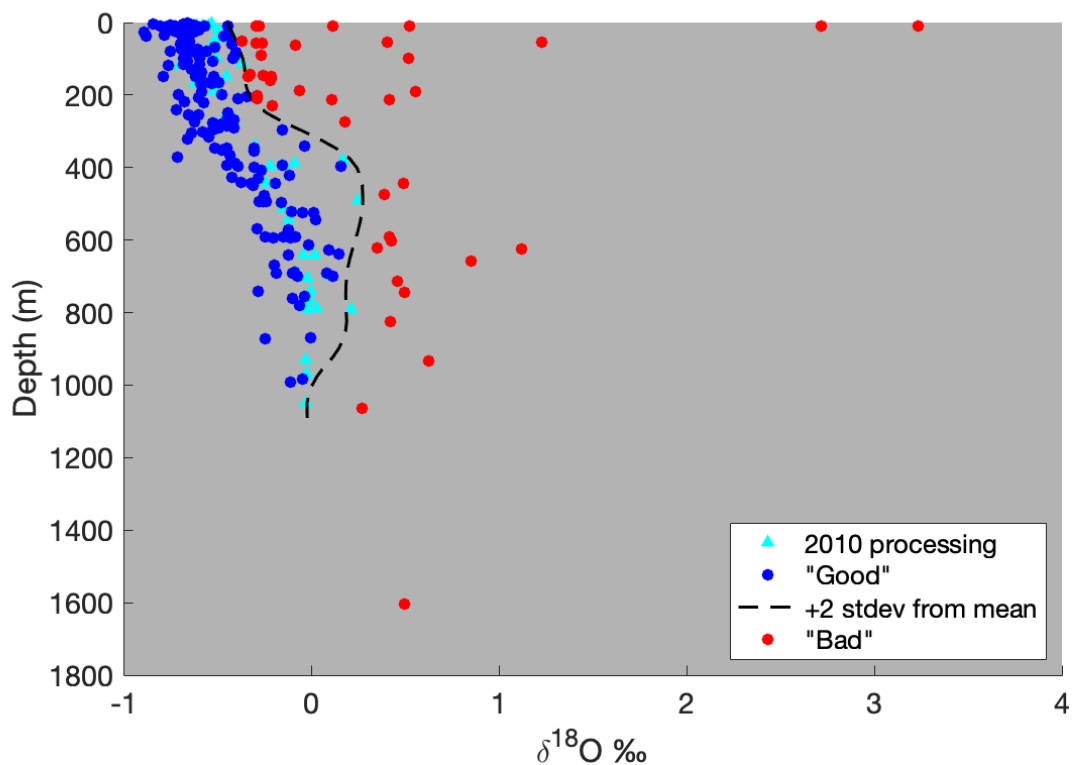
Figure A8: \delta^{18}\text{O} vs depth for all 2009 samples, coded for likelihood of evaporation. The dashed line represents +2 standard deviations from a moving depth-averaged \delta^{18}\text{O} based on the 2010 processing, beyond which the results are unacceptable. Archivable data will be made available upon publication.
