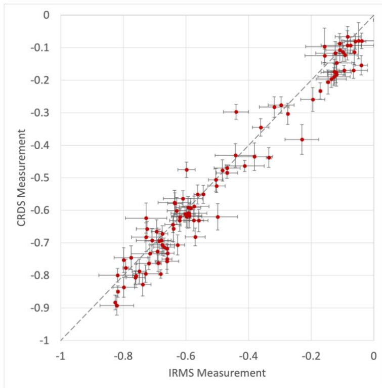
Figure A11: 101 seawater δ 18 O samples collected in 2019 and 2020 analyzed with both CRDS and IRMS. Each point represents the value obtained by measuring the same sample on the IRMS (x-axis) and the CRDS (y-axis). Error bars represent the corresponding standard deviation of the IRMS and CRDS measurements. The dashed grey line is a 1:1 slope.
