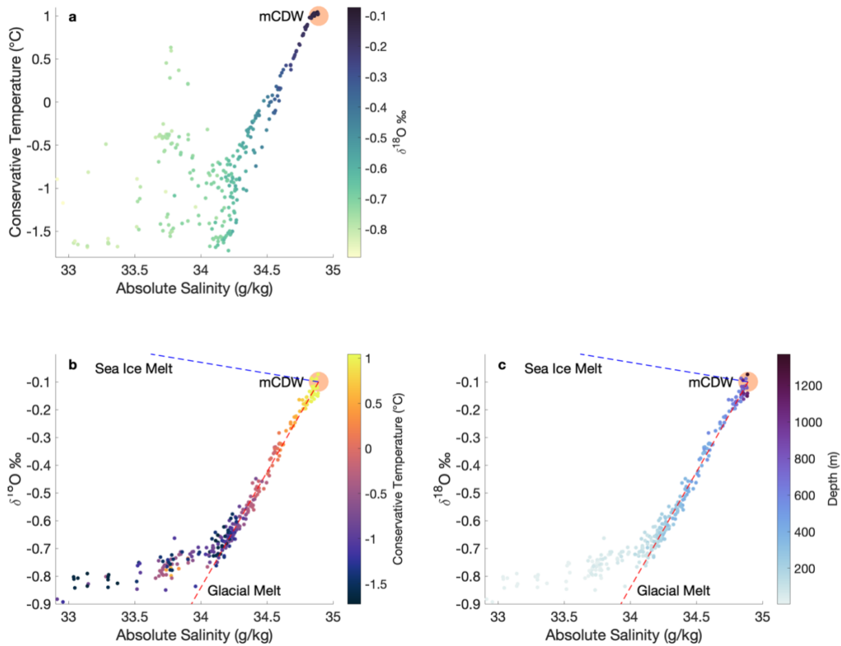
545 Figure A1: Temperature, salinity, and \delta^{18}\text{O} and depth from 2020 data. A) T-S diagram with colorbar showing \delta^{18}\text{O} . b) \delta^{18}\text{O} vs salinity with colorbar showing temperature. C) \delta^{18}\text{O} vs salinity with colorbar showing sample depth. Data diverge from the mCDW-glacial melt mixing line at depths shallower than 200 m due to the presence of sea ice melt in the admixture. In Panels b and c, dashed lines show the associated property mixing lines for mCDW mixing with sea ice melt, or GMW.
