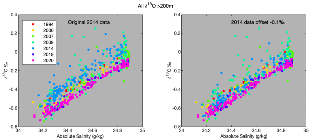
Figure A2: \delta^{18}\text{O} vs Absolute salinity for all years, from data >200\text{ m} . Left panel: All \delta^{18}\text{O} vs salinity data, with the 2014 data as published in (Biddle et al., 2019). Right panel: same, with a -0.1\text{‰} offset correction applied to the 2014 data.
