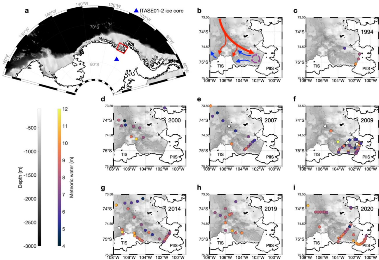
70 Figure 1: Study area bathymetry, circulation, and \delta^{18}\text{O} sampling locations each of 7 years between 1994 and 2020. 800 m isobaths are shown as thin gray lines. (a) SE Amundsen study area, and location of the ITASE01-2 ice core. (b) Location of the Pine Island Bay gyre (purple), pathways of warm deep mCDW (red) toward the ice shelves and pathways of shallower meltwater rich waters (blue) from beneath Pine Island Ice Shelf (PIIS) (Nakayama et al., 2019; Wählin et al., 2021; Dotto et al., 2022). (c-i) Colored dots show sample locations, with colors representing depth-integrated glacial meltwater inventories between 0 m and 800 m from 1994 to 2020. Thick gray lines indicate seaward boundaries of Thwaites Ice Shelf (TIS) and the PIIS. Calving fronts are referenced to 2000 (Schaffer et al., 2014; Fretwell et al., 2013), a relatively stable location before a \sim 20 km retreat following calving events between 2017 and 2020 (Joughin et al., 2021a). Stations where sampling did not extend to the seafloor show only partial water column inventories, and stations shown as white dots (2007, 2009, 2014) had two or fewer depths sampled. In 2000, 2007, and 2019, access to sampling along the front of PIIS 80 calving front was precluded by fast ice.
