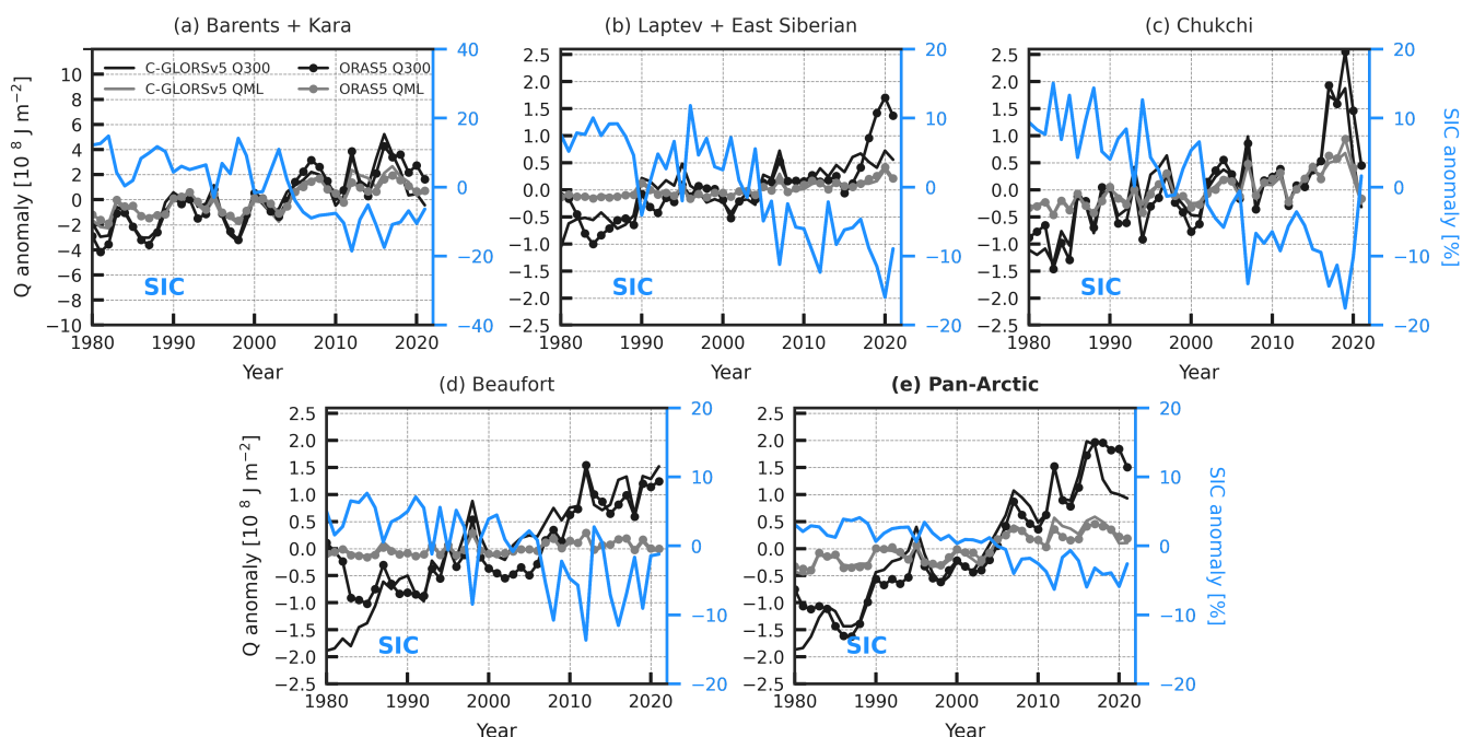
Figure 3. Anomaly time series of SIC, Q_{300} and Q_{ml} in C-GLORSv5 and ORAS5 for the Arctic regional seas and for the total Arctic. The pan-Arctic region (e) is defined as the area bounded by the Fram, BSO, Bering and Davis straits. Note the different y-axes used for the Barents-Kara region.
