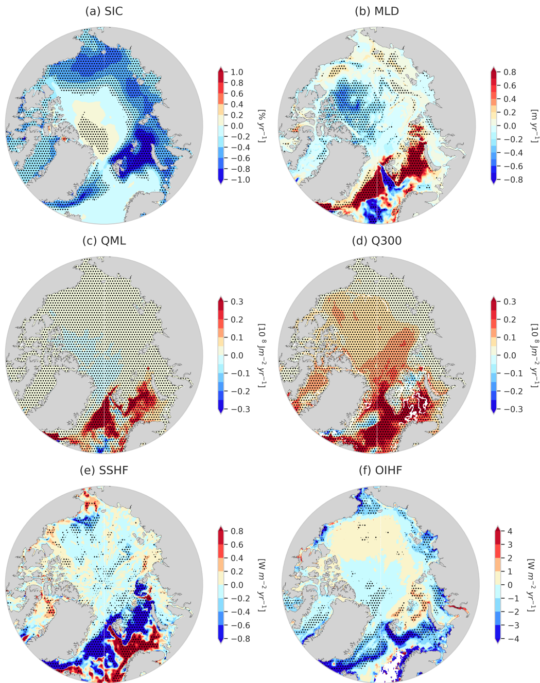
Figure 2. Annual trends (1980-2021) in (a) sea ice concentration (SIC, %), (b) mixed layer depth (MLD, m) (c) ocean heat content in the mixed layer and in (d) the 0-300 m layer ( Q_{ml} and Q_{300} , 10^8 \text{ J m}^{-2} ), (e) sea surface heat flux (SSHF, \text{W m}^{-2} ) and (f) ocean-ice heat flux (OIHF, \text{W m}^{-2} ) for the C-GLORSv5 ocean reanalysis. SSHF is defined as positive downward. Stippling denotes 95% significance.
