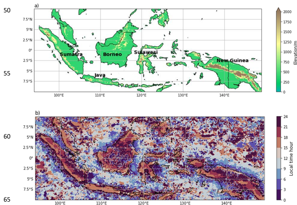
Figure 1. Maps of the selected islands within the MC showing a) the orography and b) the diurnal cycle of peak rainfall (interpolated to local solar time) using the Global Precipitation Measurement dataset (Hou et al., 2014) from December, January and February 2001 – 2020.
