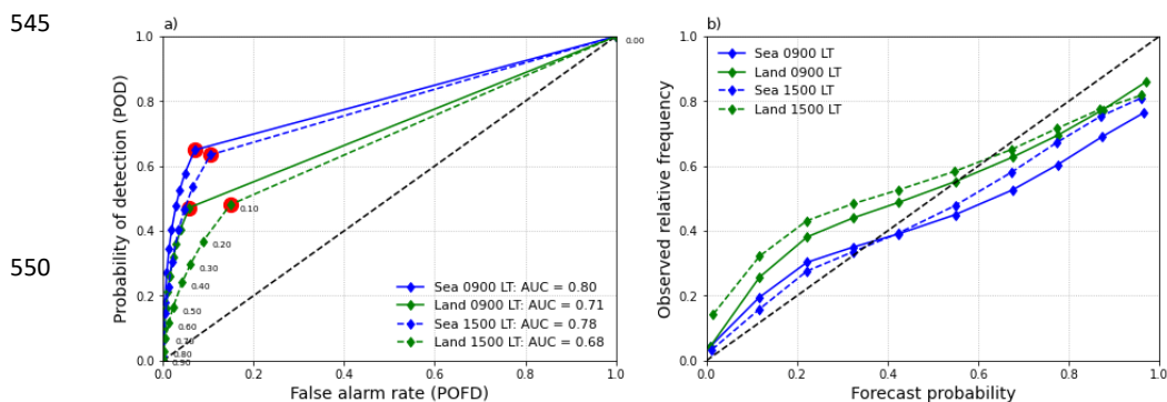
Figure 8. Composite a) ROC and b) reliability curves over the sea and land for STEPS 3-hour lead time nowcasts, initialised at 9am (441 nowcasts) and 3pm (405 nowcasts), with a threshold of < 235 K. The numbers next to the green points in a) represent the thresholds used to evaluate the nowcast at different likelihoods.
