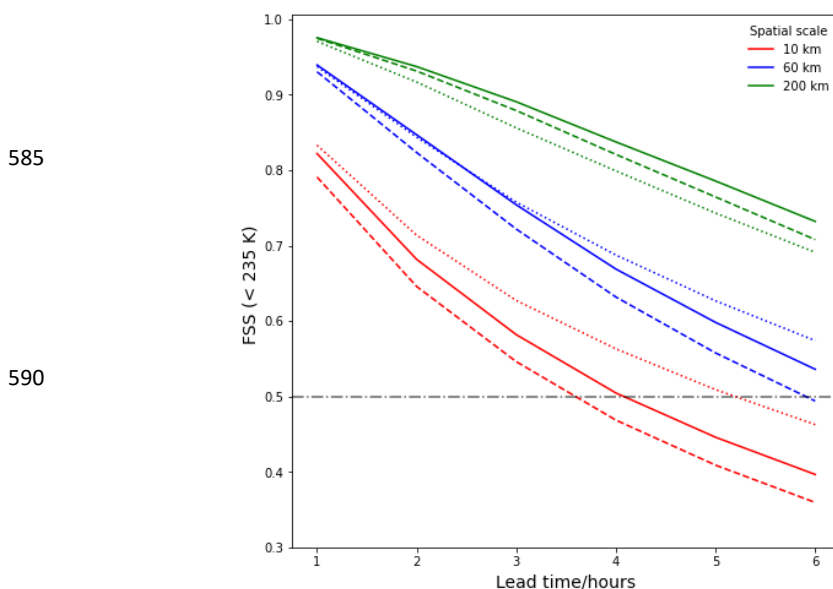
595 Figure 9. Composite FSSs against lead time for 3,457 LK (solid line), STEPS10 (dotted line) and persistence (dashed line) nowcasts, evaluated at a threshold of 235 K for 10 km, 60 km and 200 km spatial scales. The grey horizontal line marks the 0.5 FSS line, which is considered the cut-off for nowcast skill.
