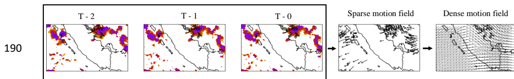
Figure 2. An example (using BT over Sumatra) of how a motion field is generated using the LK method. Features are identified and tracked across the three input images (T-0, T-1 and T-2) to generate the sparse motion field. The sparse motion field is then interpolated onto the rest of the domain to produce the dense motion field.
