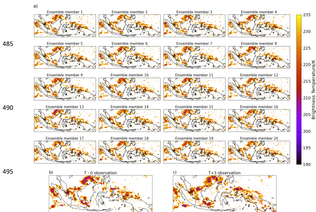
500 Figure 6. a) An example of a 20 member ensemble, 3-hour lead time BT nowcast produced by the STEPS implementation of pySTEPS on 11 December 2019. b) The observation at the nowcast initialisation time and c) the observation 3 hours later.
