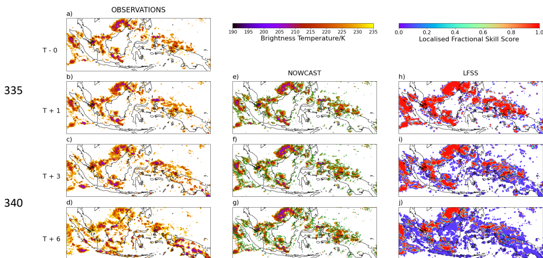
Figure 3. a)-d) are maps of BT observations showing convection propagating across the MC on 11 December 2019 starting from the initial observation at 0900 LT (T-0), followed by the observation at 1 hour (T+1), 3 hours (T+3) and 6 hours (T+6) later. e)-g) are the nowcasts produced by the LK algorithm at each of the corresponding observations, and the green lines show the contour of the corresponding persistence nowcast. h)-j) are the LFSS maps produced by evaluating each nowcast against the corresponding observation on a 20 km spatial scale.
