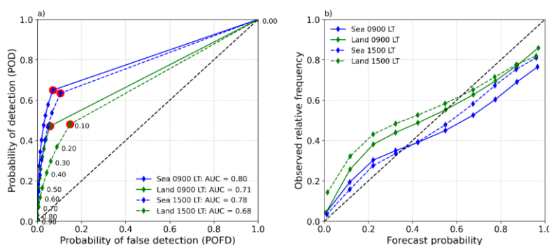
570 Figure 8. Composite a) ROC and b) reliability curves over the sea and land for STEPS 3-hour lead time nowcasts, initialised at 9am (441 nowcasts) and 3pm (405 nowcasts), with a threshold of < 235 K. The numbers next to the green points in a) represent the thresholds used to evaluate the nowcast at different likelihoods.
