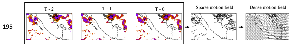
Figure 2. An example (using BT over Sumatra) of how a motion field is generated using the LK method. Features are identified and tracked across the three input images (T-0, T-1 and T-2) to generate the sparse motion field. The sparse motion field is then interpolated onto the rest of the domain to produce the dense motion field.
