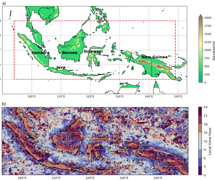
Figure 1. a) Orographic map of the Maritime Continent showing the domain over which the nowcasts were generated and the domain over which they were evaluated (red dotted line). Maps of the selected islands within the MC showing a) the orography and b) the diurnal cycle of peak rainfall within the evaluation region (interpolated to local solar time) using the Global Precipitation Measurement dataset (Hou et al., 2014) from December, January and February 2001 – 2020.
