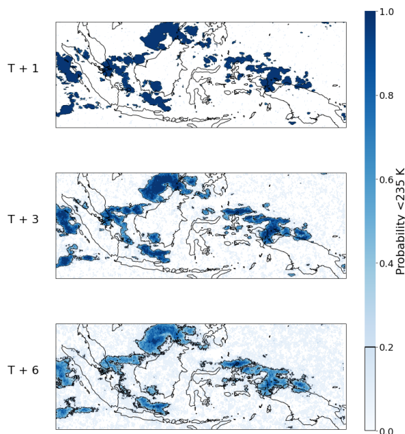
Figure 7. An example of a probabilistic BT nowcast for lead times of 1, 3 and 6 hours produced by the STEPS implementation of pySTEPS on 11 December 2019. A BT threshold of < 235 K is used in order to include all pixels in the nowcast.
