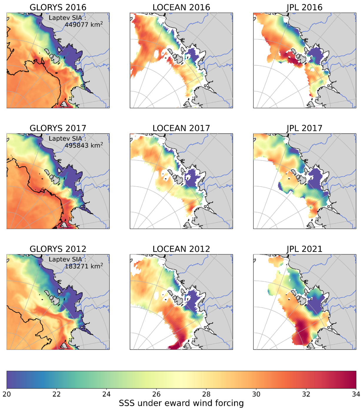
Figure A6: Years of eastward wind forcing for all years used to calculate eastward composites for (left to right) GLORYS12V1 SSS and LOCEAN SMOS (2016, 2017, 2012) and for JPL SMAP (2016, 2017, 2021). The GLORYS12V1 mean 30% sea ice concentration contour and mean GLORYS12V1 sea ice area (SIA) in the Laptev Sea (120-140, 68-85N) for each year shown is overlaid on that year's plot.
