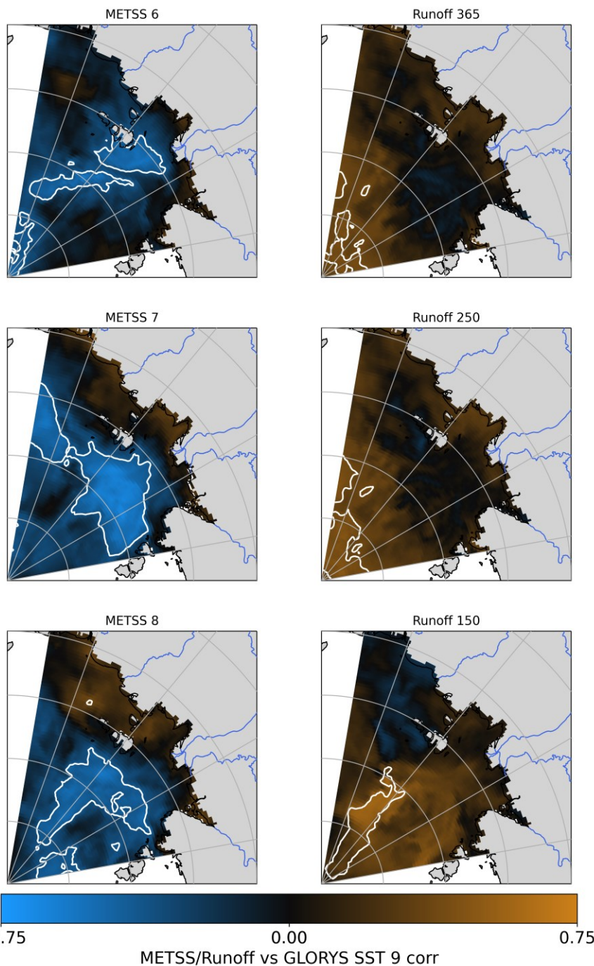
Figure A4: Correlation between GLORYS12V1 September SST and mean eastward turbulent surface stress (METSS) over 70-80 North and 120-160 East in June (6), July (7), August (8) (left column) over 1993-2022. Correlation between GLORYS12V1 September SST and cumulative Lena River runoff over the full year (Julian day 365), in summer (Julian day 250) and in spring (Julian day 150) (right column) over 1993-2022. Regions where correlations are statistically significant ( p \leq 0.05 ) are denoted by the white contour and brighter colours.
