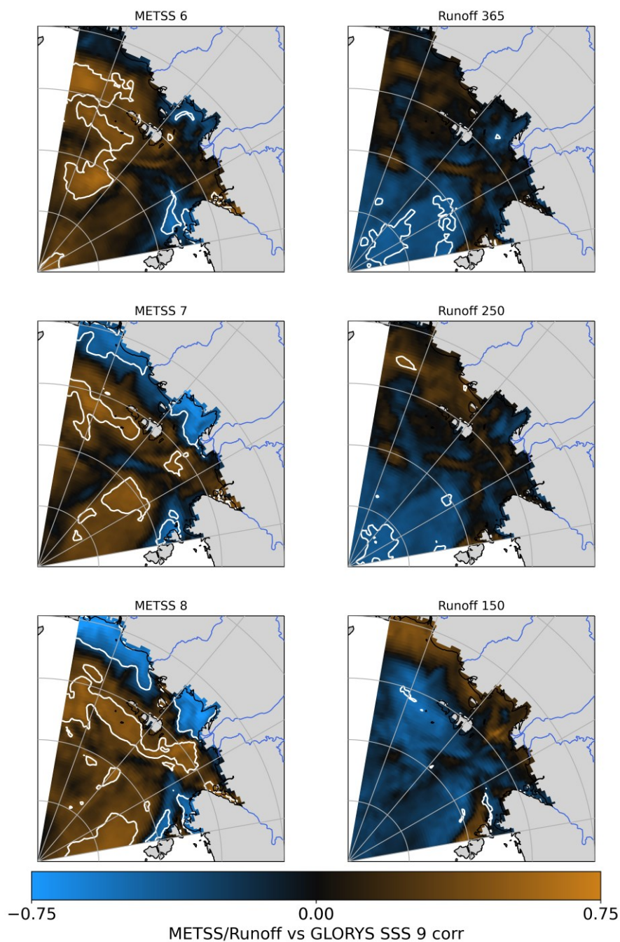
815 Figure A3: Correlation between GLORYS12V1 September SSS and mean eastward turbulent surface stress (METSS) over 70-80 North and 120-160 East in June (6), July (7), August (8) (left column) over 1993-2022. Correlation between GLORYS12V1 September SSS and cumulative Lena River runoff over the full year (Julian day 365), in summer (Julian day 250) and in spring (Julian day 150) (right column) over 1993-2022. Regions where correlations are statistically significant ( p \leq 0.05 ) are denoted by the white contour and brighter colours.
