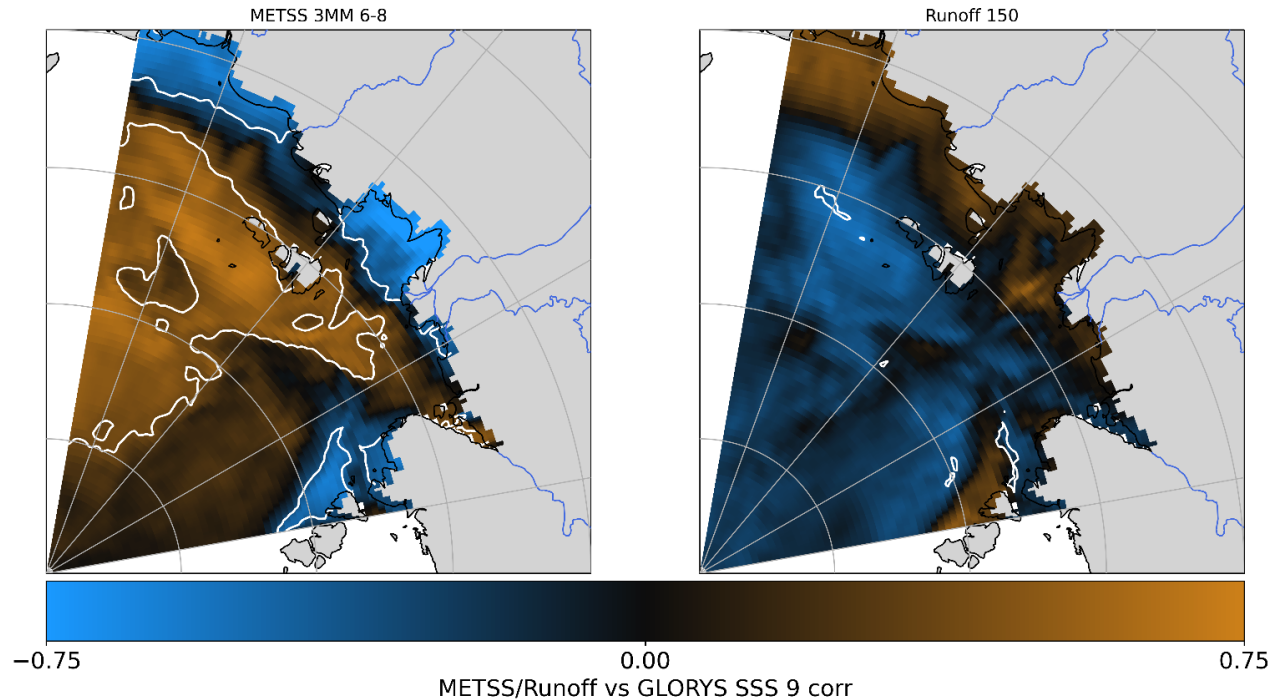
Figure 4: Correlation between GLORYS12V1 September SSS and the three-month mean ERA5 eastward turbulent surface stress (METSS) over June to August (6-8) (left) over 1993-2022. Correlation between GLORYS12V1 September SSS and cumulative Lena River runoff in spring (Julian day 150) (right) over 1993-2022. Regions where correlations are statistically significant ( p \leq 0.05 ) are denoted by the white contour and brighter colours.
