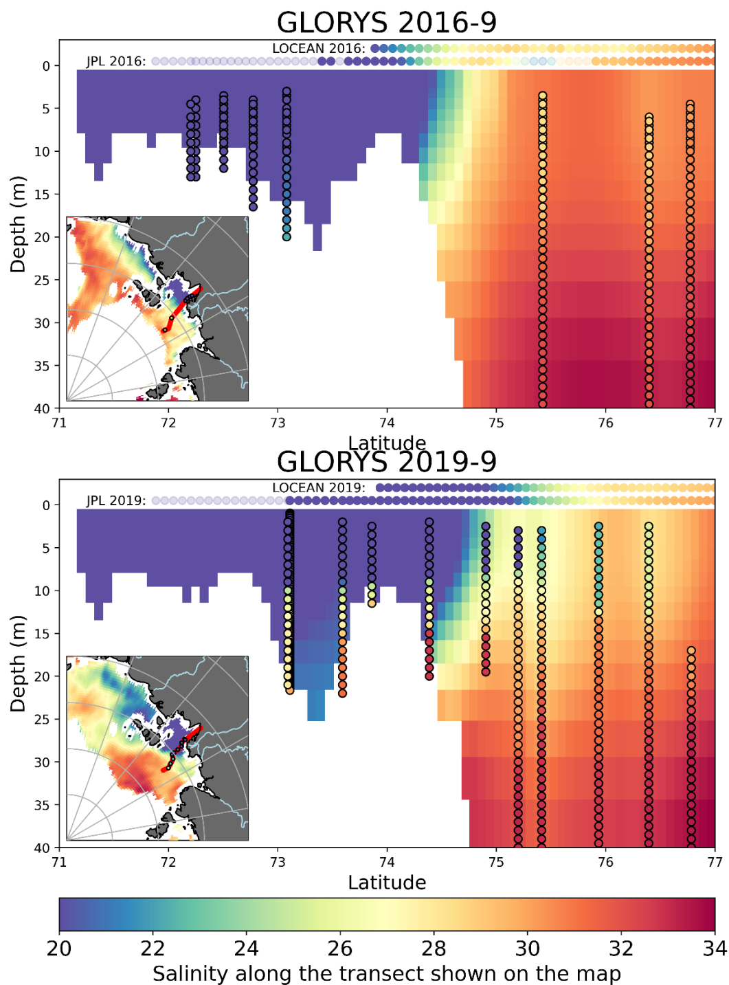
Figure 3: GLORYS12V1 salinity vertical transect in 2016 (top) and 2019 (bottom) along red transect interpolated through in-situ data (shown in map of JPL SMAP SSS in bottom left for each year) with in-situ data overlaid with black rings and satellite data for that transect in JPL SMAP and LOCEAN SMOS SSS shown as a line of points. JPL SMAP data is made semi-transparent where the provided SMAP SSS uncertainty is > 1 pss.
