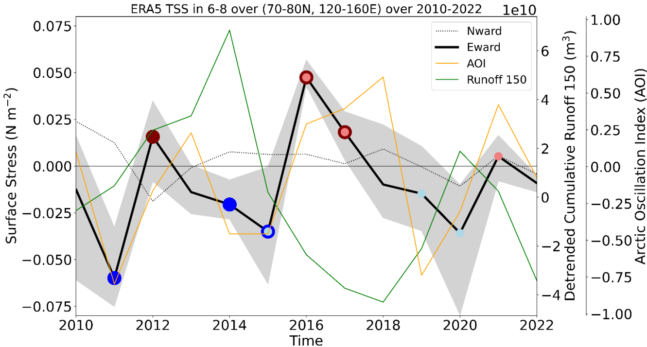
390 Figure 7: Three-month (June to August) mean ERA5 eastward (black solid) and northward (black dashed) turbulent surface stress over 70-80 North and 120-160 East. Overlaid are dots indicating the most eastward (red dots) and westward (blue dots) years chosen for analysis for both the longer SMOS/GLORYS12V1 timeseries (2011-2020) (darker red and blue dots) and the shorter SMAP timeseries (2015-2022) (lighter red and blue dots). The range of the maximum and minimum eastward turbulent surface stress between June and August is shaded in grey. Spring cumulative Lena River runoff (until the 150 th Julian day) (green) and mean June to August arctic oscillation index (AOI) (orange) are overlaid.
