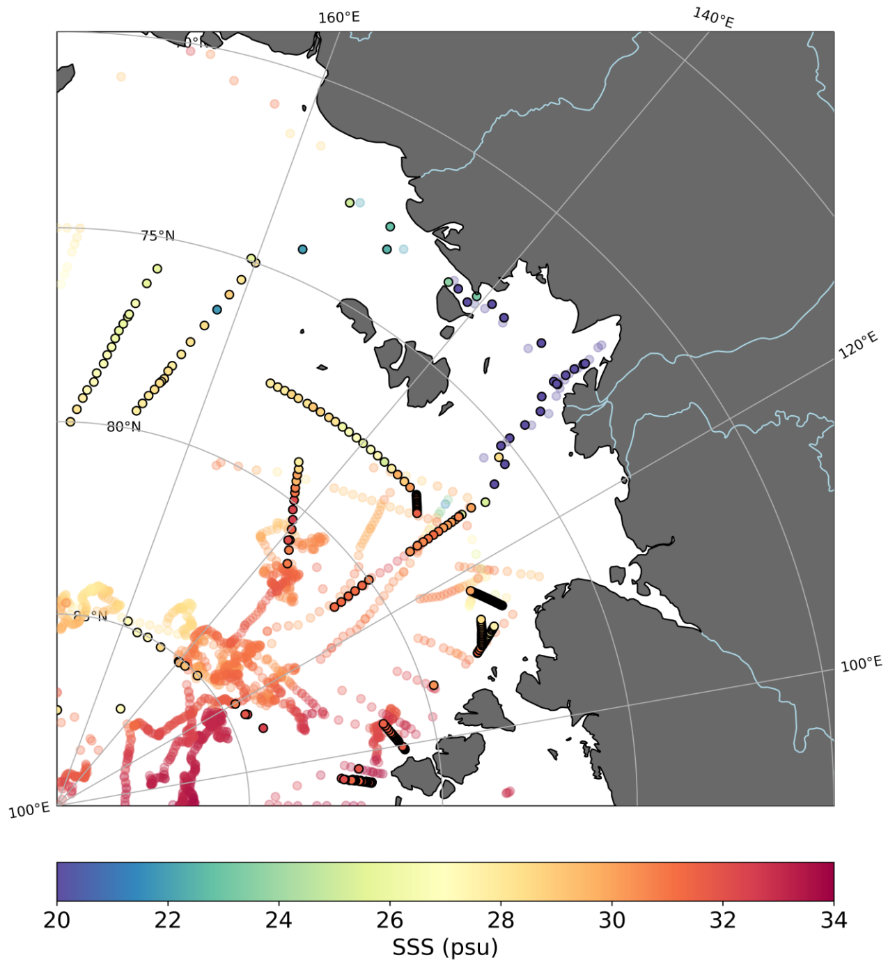
765 Figure A1: In-situ data (<10 m) used for validation of satellite and reanalysis products, coloured by their salinity value. Data with black circles were collected over the SMAP period (2015-present), and those without black circles were collected over the SMOS period (2010-present).
