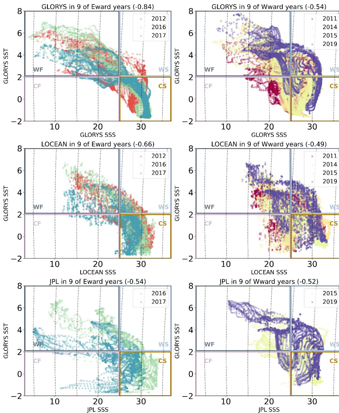
835 Figure A7: T-S diagrams over the Laptev Sea (65-80 °N, 120-160 °E)-for September under eastward (2012, 2016, 2017) (left column) and westward (2011, 2014, 2015, 2019) (right column) wind forcing for GLORYS12V1 SST and GLORYS12V1 SSS (top), LOCEAN SMOS SSS (middle) and JPL SMAP SSS (bottom) colour coded by year over 2010-2020. Density contours are overlaid as dashed black lines. Spearman correlation coefficients between the SSS product and GLORYS12V1 SST across all eastward/westward years shown is displayed in the title of each subplot. Boxes are overlaid for 4 water masses depicting warm, fresh water (WF, SST>2 °C, SSS<25 pss), cold, fresh water (CF, SST<2 °C, SSS<25 pss), warm salty water (WS, SST>2 °C, SSS>25 pss) and cold, salty water (CS, SST<2 °C, SSS>25 pss) 840
