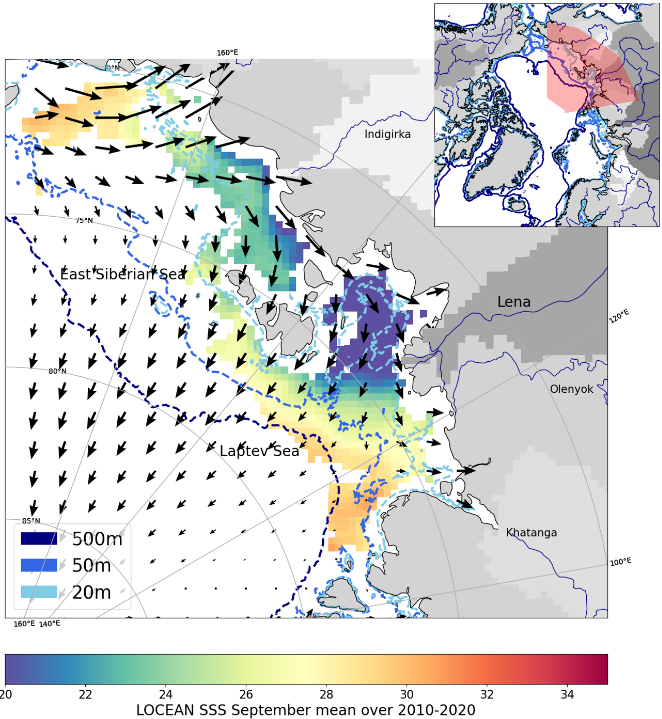
60 Figure 1 : 2010-2020 LOCEAN SMOS satellite mean September SSS with GEBCO bathymetry contours for 20m, 50m and 500m overlaid in blue with mean 2010-2020 ERA5 June-August wind vectors overlaid over the ocean. The inset in the top right corner depicts Arctic wide GEBCO bathymetry and the location of this region within the wider Arctic in red.
