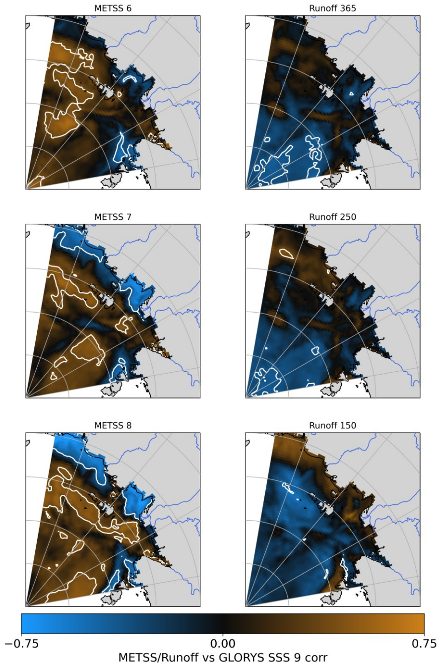
770 Figure A1: Correlation between GLORYS12V1 September SSS and mean eastward turbulent surface stress (METSS) over 70-80 North and 120-160 East in June (6), July (7), August (8) (left column) over 1993-2022. Correlation between GLORYS12V1 September SSS and cumulative Lena River runoff over the full year (Julian day 365), in summer (Julian day 250) and in spring (Julian day 150) (right column) over 1993-2022. Regions where correlations are statistically significant ( p \leq 0.05 ) are denoted by the white contour and brighter colours.
