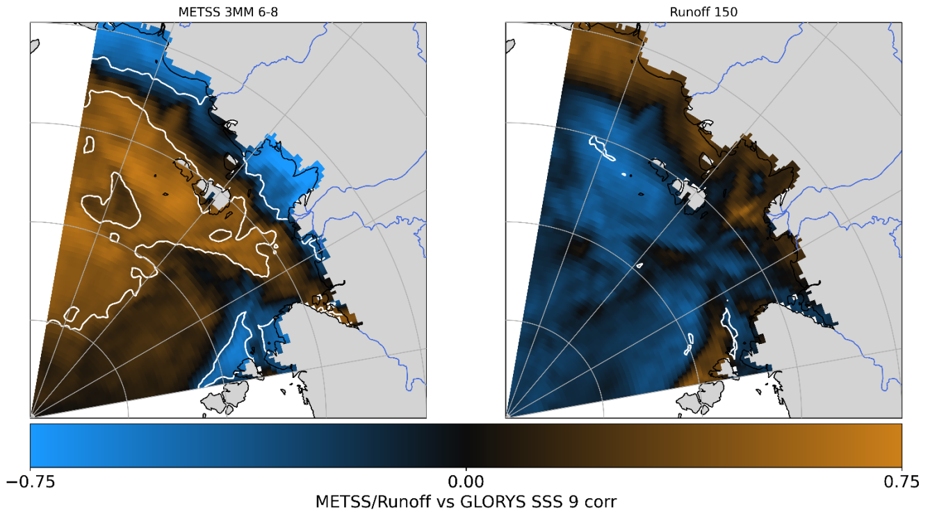
305 Figure 4: Correlation between GLORYS12V1 September SSS and the three-month mean ERA5 eastward turbulent surface stress (METSS) over June to August (6-8) over 1993-2022. Correlation between GLORYS12V1 September SSS and cumulative Lena River runoff in spring (Julian day 150) over 1993-2022. Regions where correlations are statistically significant ( p \leq 0.05 ) are denoted by the white contour and brighter colours.
