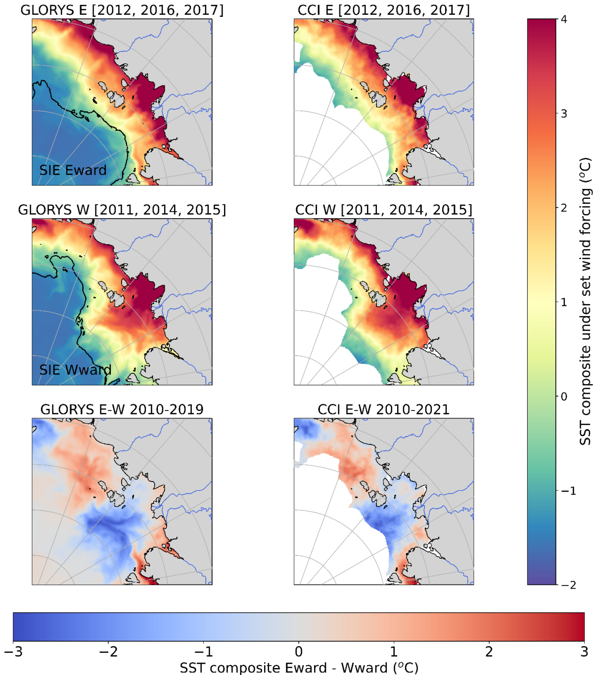
Figure 9 : Eastward ( E , top row) and westward ( W , middle row) composites calculated from the identified three most eastward and westward years for (left to right) GLORYS12V1 SST and L4 CCI SST (masked by 30% sea ice concentration). The difference composite (eastward – westward) for each product is shown on the bottom row. The mean 30% sea ice concentration contour for eastward and westward years is used to mask L4 CCI data and is overlaid in GLORYS12V1 in black on both eastward and westward composite plots.
