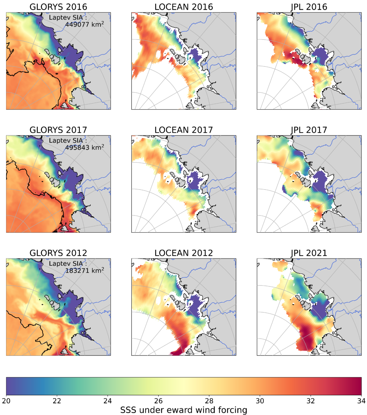
785 Figure A4: Years of eastward wind forcing for all years used to calculate eastward composites for (left to right) GLORYS12V1 SSS and LOCEAN SMOS (2016, 2017, 2012) and for JPL SMAP (2016, 2017, 2021). The GLORYS12V1 mean 30% sea ice concentration contour and mean GLORYS12V1 sea ice area (SIA) in the Laptev Sea (120-140, 68-85N) for each year shown is overlaid on that year's plot.
