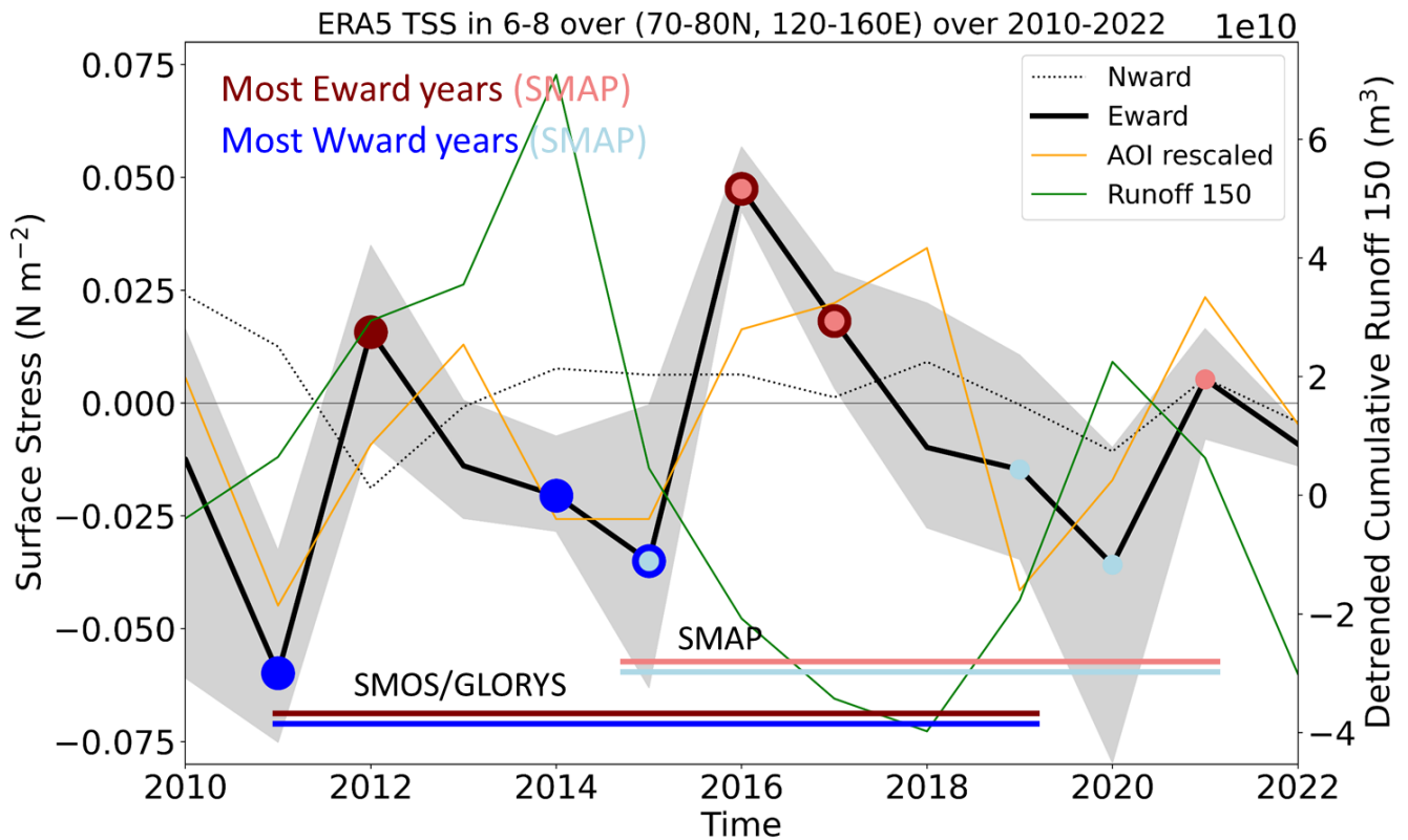
Figure 7: Three-month (June to August) mean ERA5 eastward (black solid) and northward (black dashed) turbulent surface stress over 70-80 North and 120-160 East. Overlaid are dots indicating the most eastward (red dots) and westward (blue dots) years chosen for analysis for both the longer SMOS/GLORYS12V1 timeseries (darker red and blue dots) and the shorter SMAP timeseries (lighter red and blue dots). The range of the maximum and minimum eastward turbulent surface stress between June and August is shaded in grey. Spring cumulative Lena River runoff (until the 150 th Julian day) (green) and mean June to August arctic oscillation index (AOI) (orange, standardized by standard deviation of surface stress) are overlaid.
